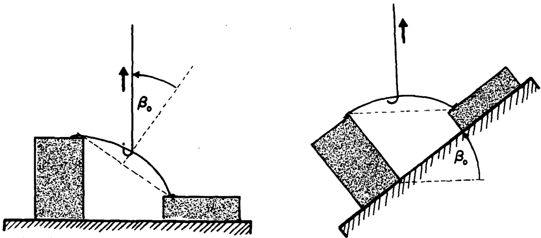
a. Level substrate; nominal pull angle \beta = \beta_0 . b. Tipped substrate; nominal pull angle \beta = \theta .
