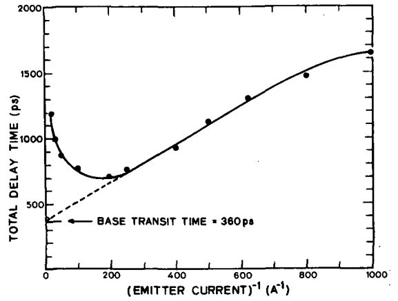
Figure 29. Transit time of a 2N2219 transistor derived from S-parameter measurements. ( V_{CB} = 5V ).
