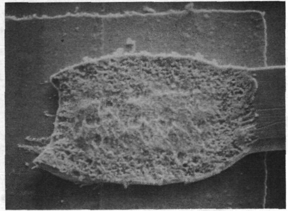
b. Second bond. Magnification \sim 500 \times .
