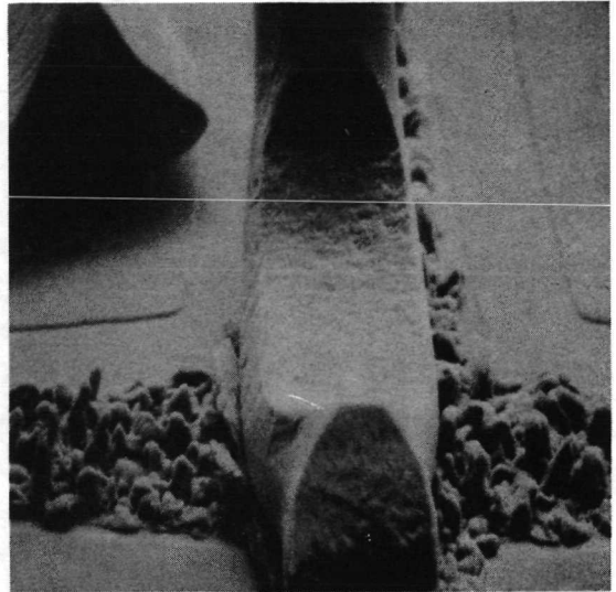
a. Small bond deformation ( \sim 1.2 times wire diameter). Magnification \sim 585 X.
