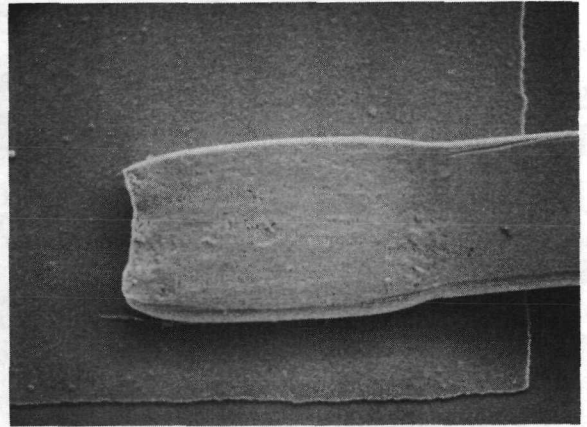
b. Second bond. Magnification \sim 470 \times .
