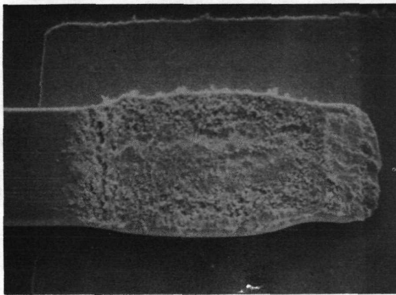
a. First bond. Magnification \sim 430 \times .
