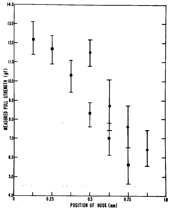
Figure 19. Measured pull strength of moderately deformed (●) and excessively deformed (■) single-level second bonds for different hook positions.
