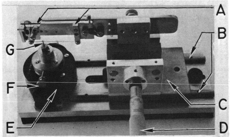
Figure 9. Device for polishing convex surfaces and grooves on bonding tools.
