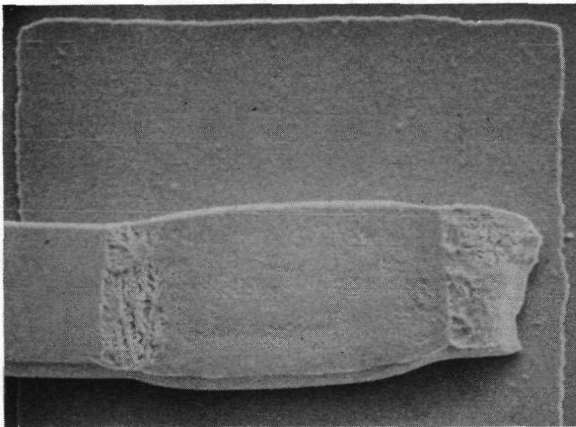
a. First bond. Magnification \sim 460 \times .
