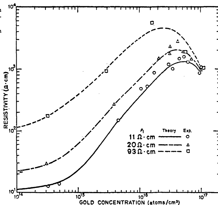
Figure 1. Resistivity as a function of gold concentration in p -type silicon with initial resistivity \rho_i of 11, 20, and 93 \Omega\cdot\text{cm} . (Error bars on the experimental points are not indicated. The standard deviation of the gold determination is estimated to be about 10 percent. Resistivity values are reproducible within about 5 percent. The parameters used to generate the theoretical curves are given in the text.)
