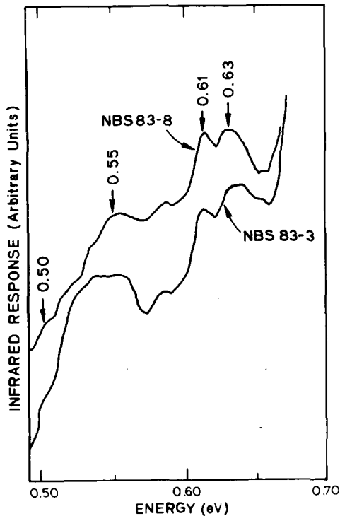
Figure 2. Infrared response spectra of two germanium gamma-ray detectors.
