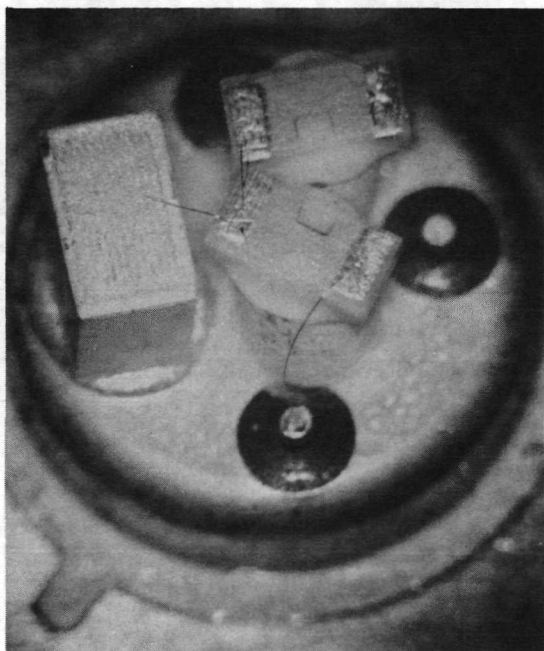
Figure 26. Photomicrograph of typical R-C plug-in network assembled on a TO-5 header. (Magnification \sim 8.4 \times ).
