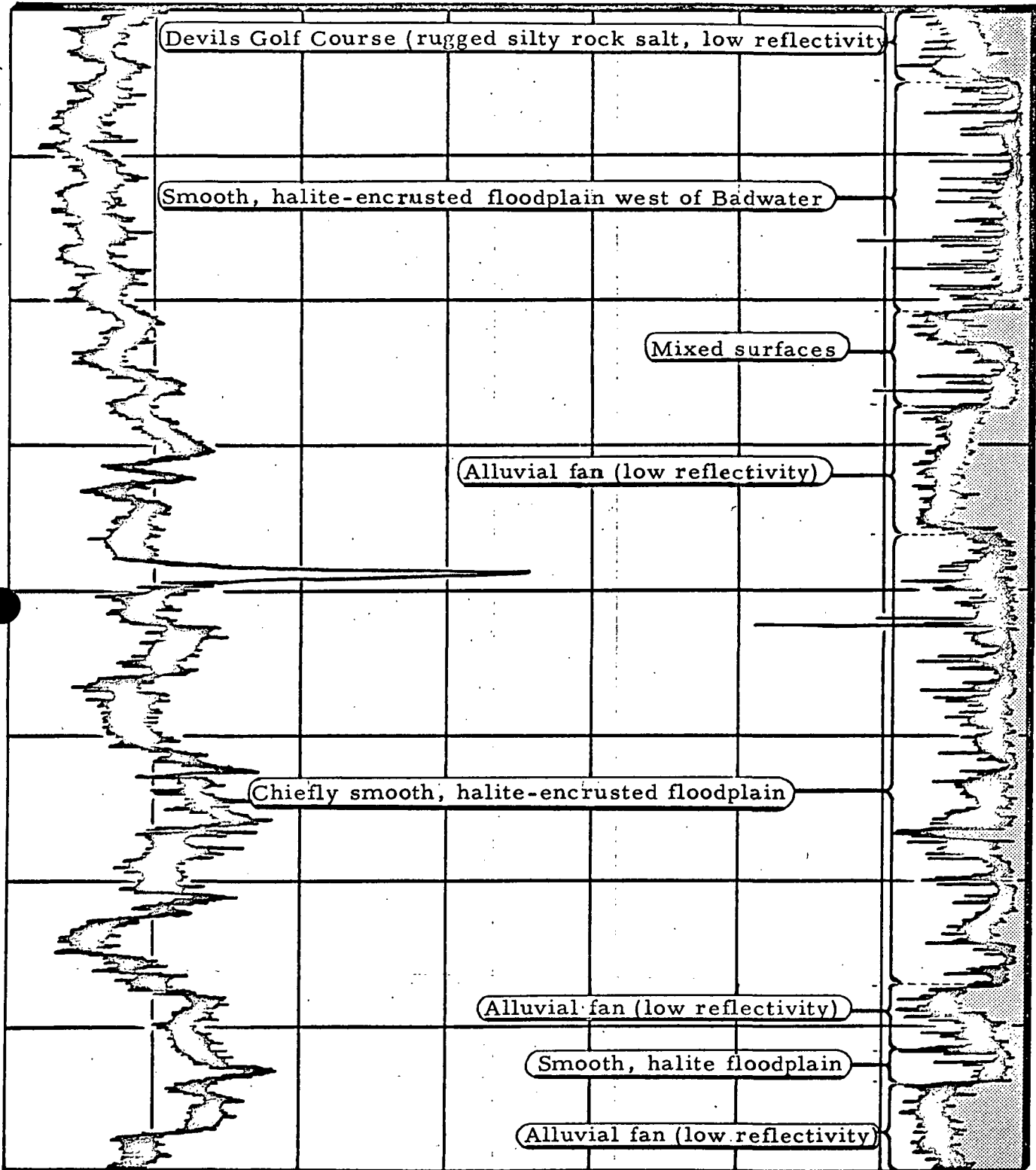
Figure 9. FLD response to materials of strongly contrasting reflectivity (December 9, 1969, Badwater Basin, Death Valley, California)
