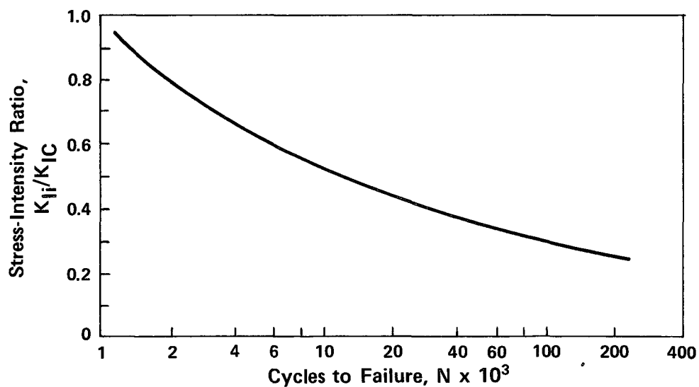
Figure I-5. Cyclic Flow Growth for 7079-T6 Aluminum Plate. One-Inch Thick Specimens, With a K_{IC} of 34 ksi-in. 1/2 and a Yield Strength of 65 ksi, Were Cycled at 1,800 rpm. [Source: Forsyth, 1969.]
