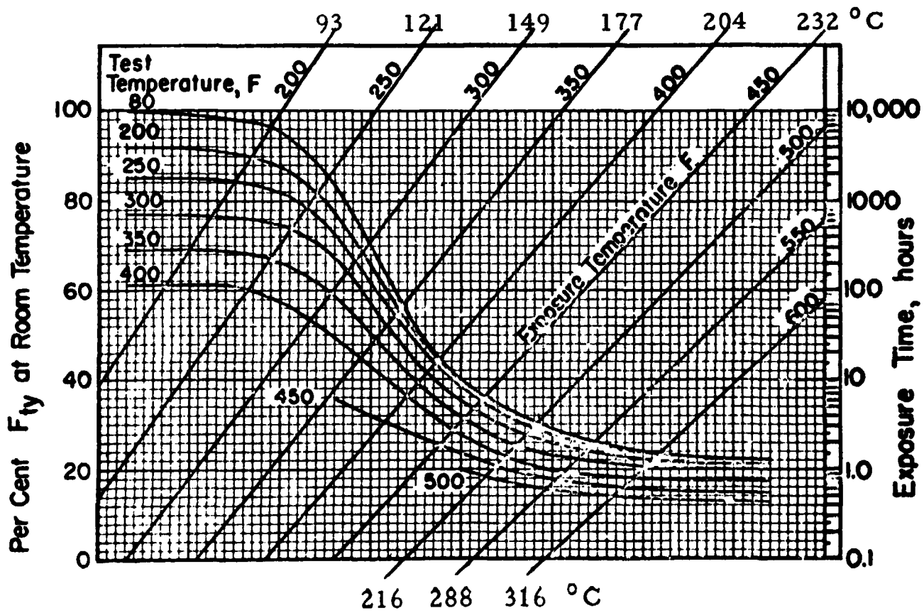
FIGURE 7.4133. — Effect of temperature on the tensile yield strength of 7075-T6 (all products). (Ref. 7.5)
