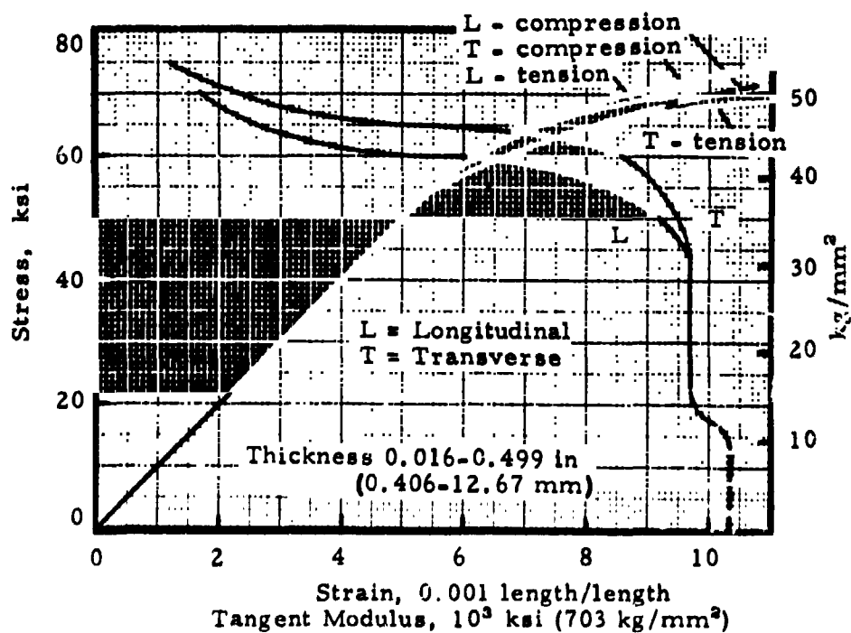
FIGURE 7.255. — Typical stress-strain and tangent modulus curves for Clad 7075-T6 sheet and plate at room temperature. (Ref. 7.5)
