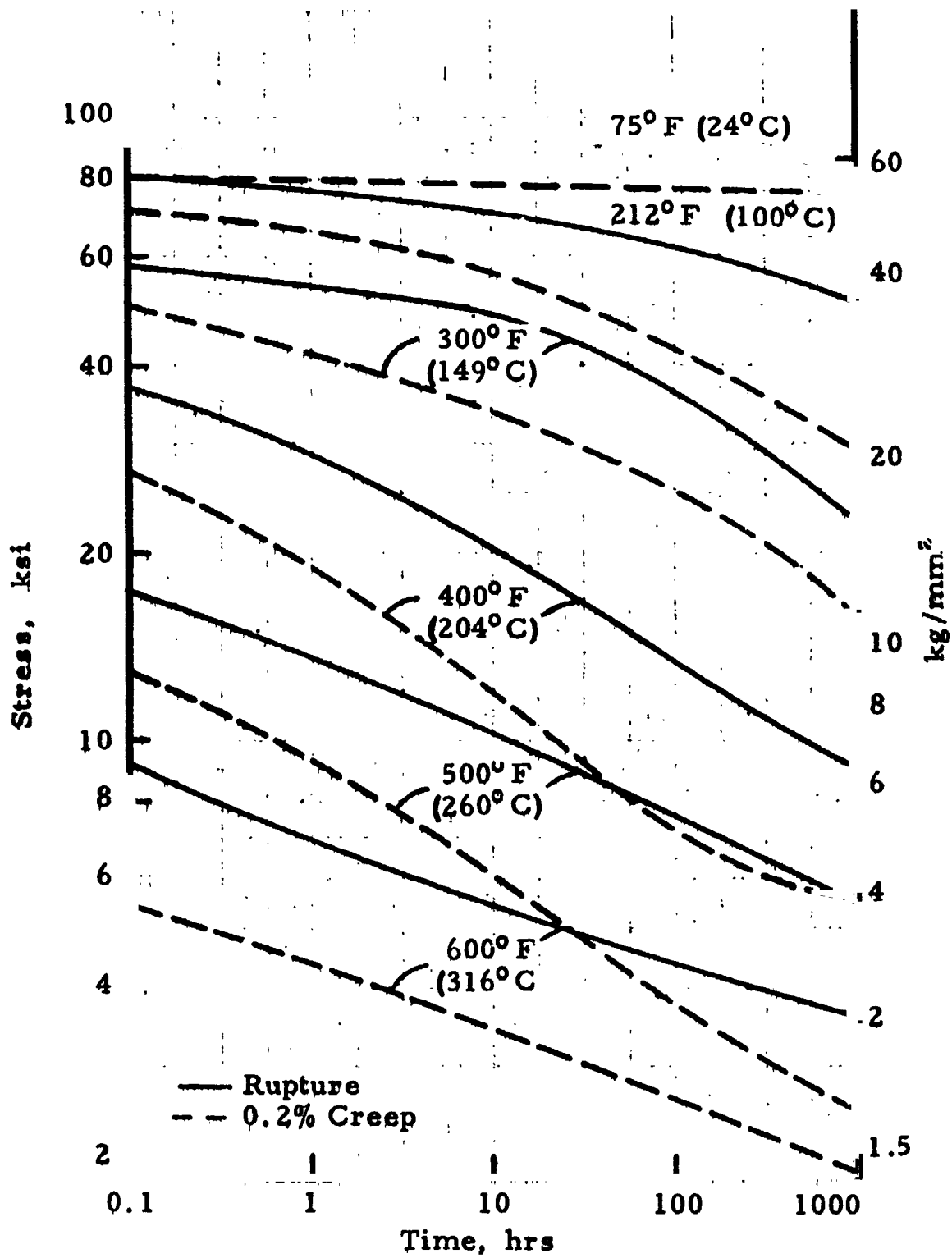
FIGURE 8.412. — Creep and creep rupture curves for 7075-T6 and -T6511 extrusions, 0.25 to 3.0 inches (6.35 to 76.2 mm) thick.
