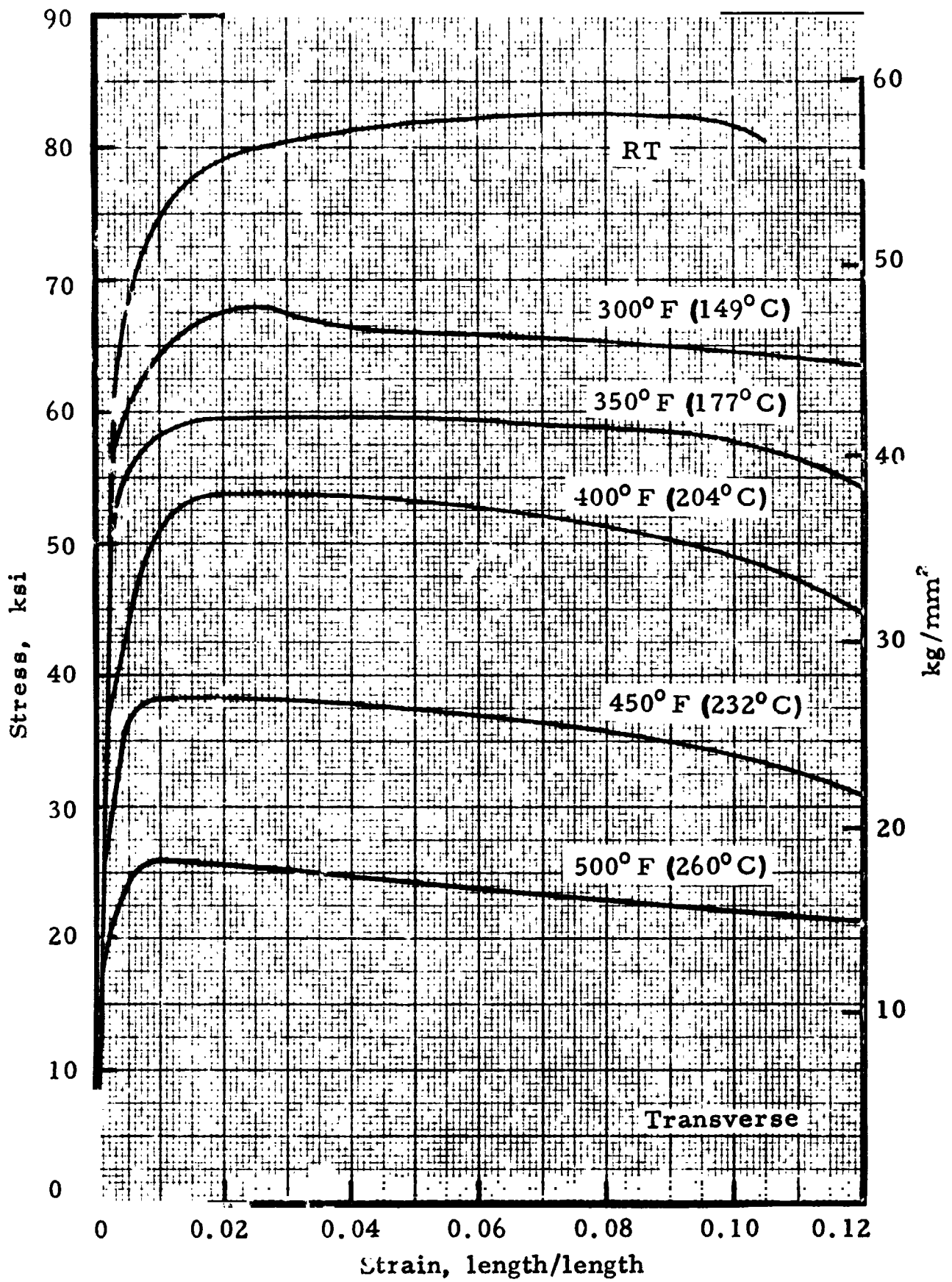
FIGURE 7.4125. — Complete stress-strain curves for 7075-T6 sheet at room and elevated temperatures.
