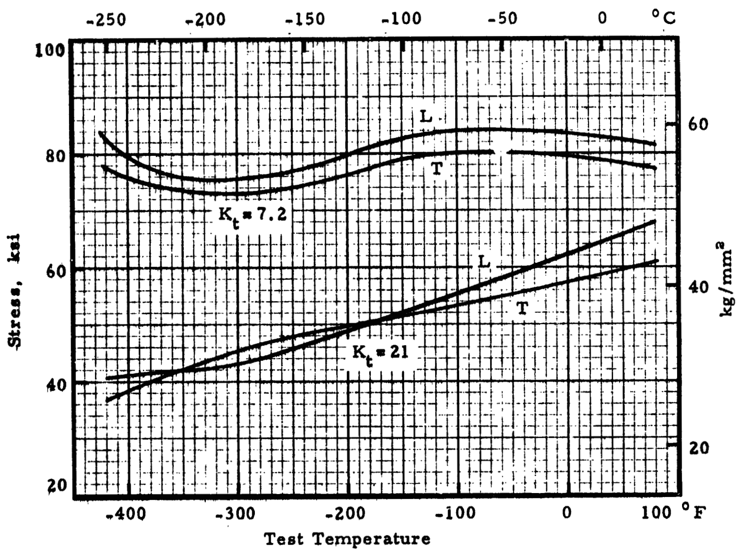
FIGURE 7.4613. — Effect of low temperatures on notch strength of 7075-T6 sheet; thickness, 0.125 inch (3.175 mm).
