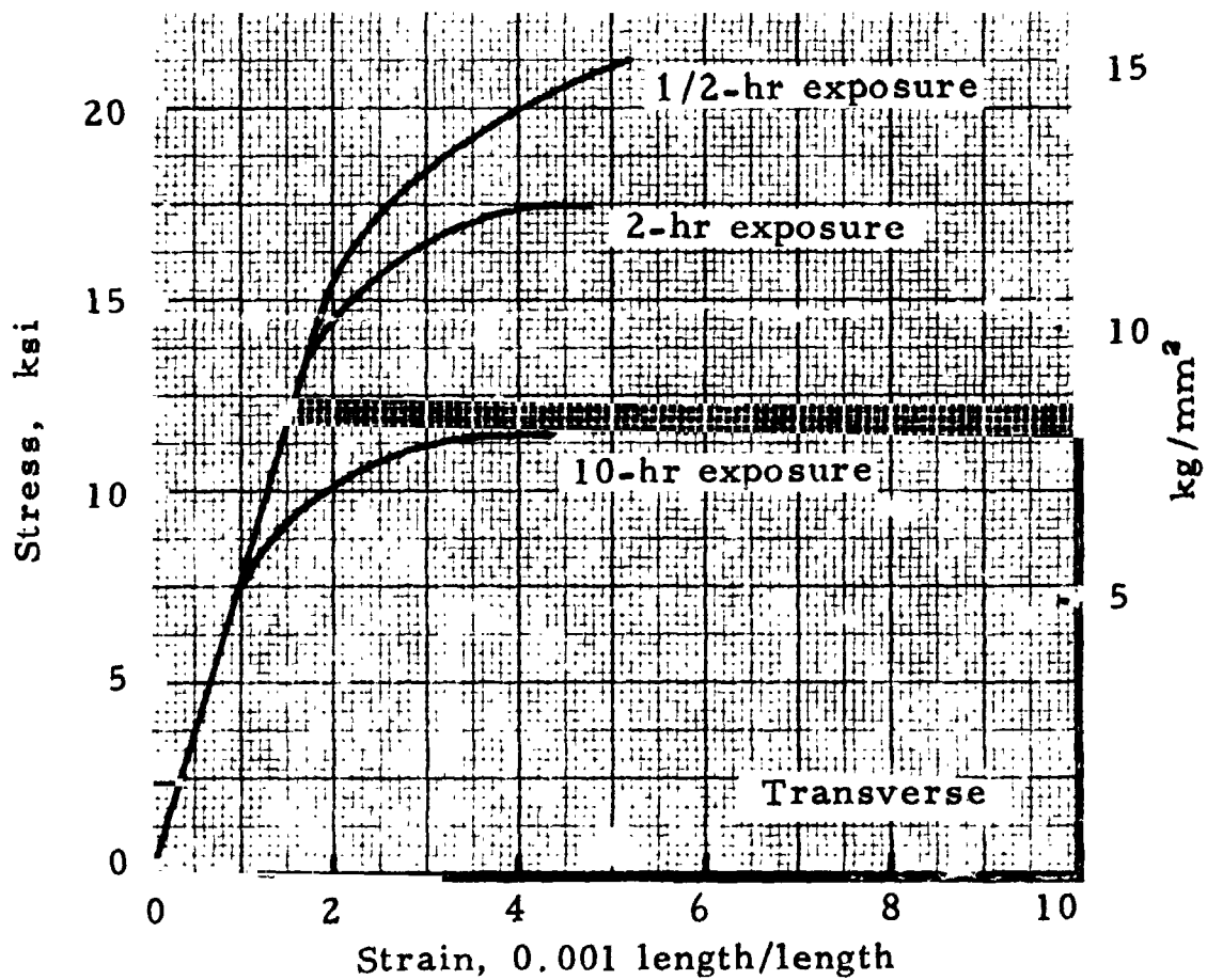
FIGURE 7.225. — Typical compressive stress-strain curves for Clad 7075-T6 sheet at 500° F (260° C). (Ref. 7.5)
