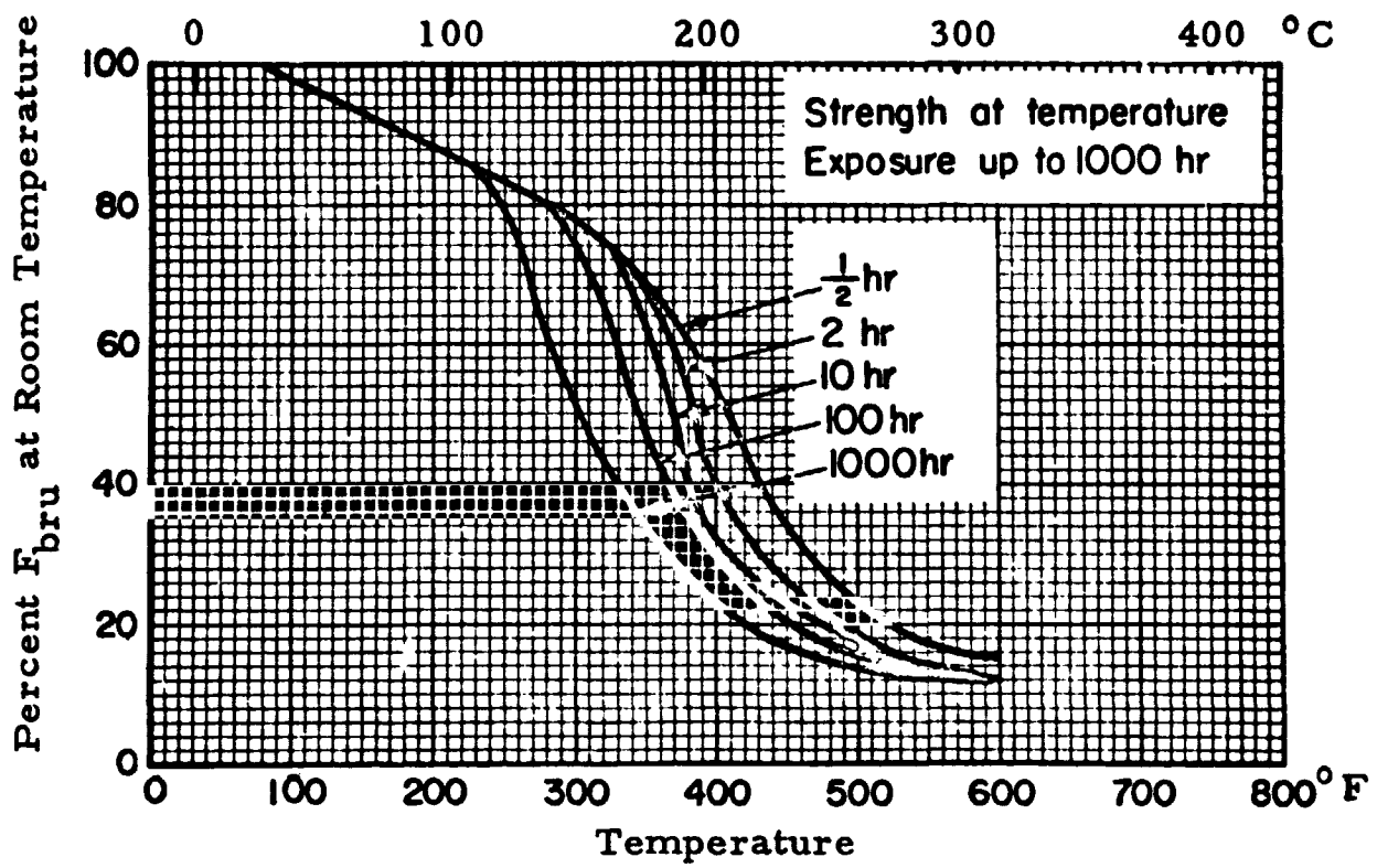
FIGURE 7.4519. — Effect of temperature on the ultimate bearing strength of 7075-T6 (all products).
