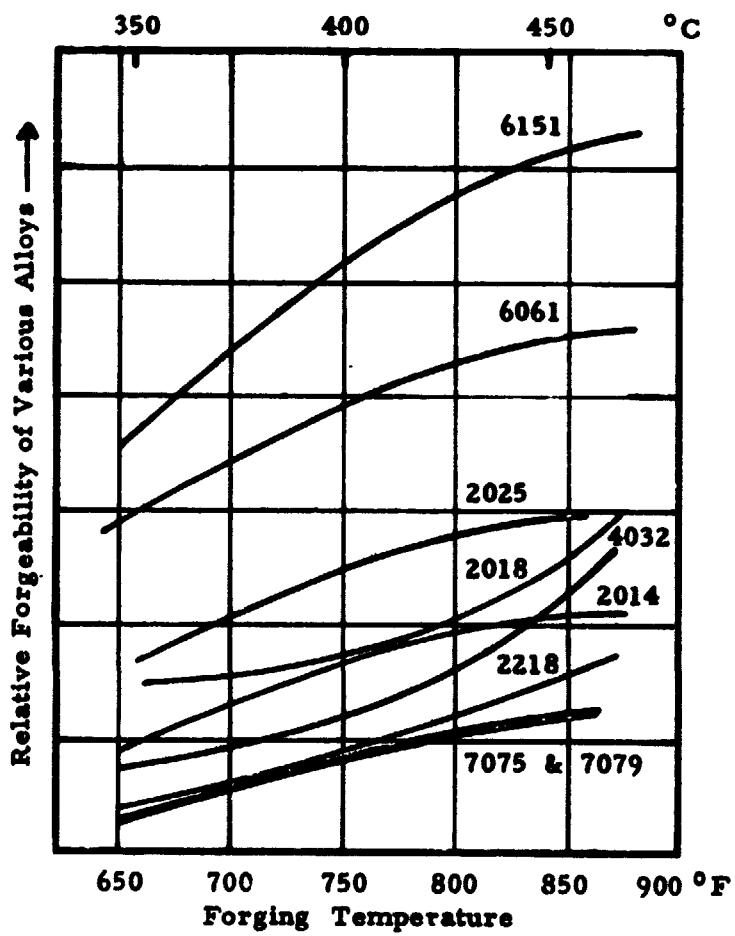
FIGURE 5.4. — Relative forgeability of various aluminum alloys. (Ref. 5.8)
