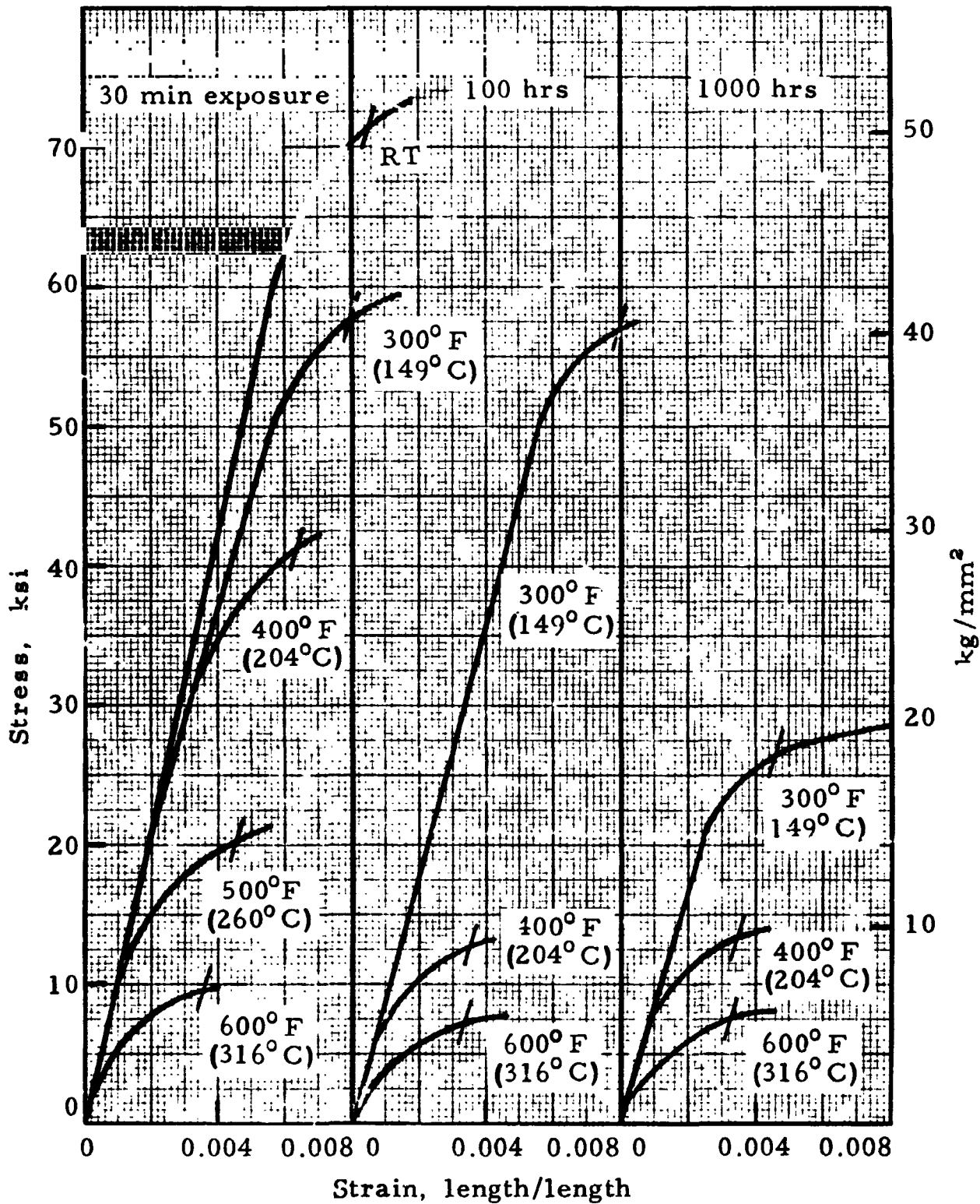
FIGURE 7.4221. — Stress-strain curves in compression for Clad 7075-T6 at room and elevated temperatures; thickness, 0.064 inch (1.625 mm). (Ref. 7.10)
