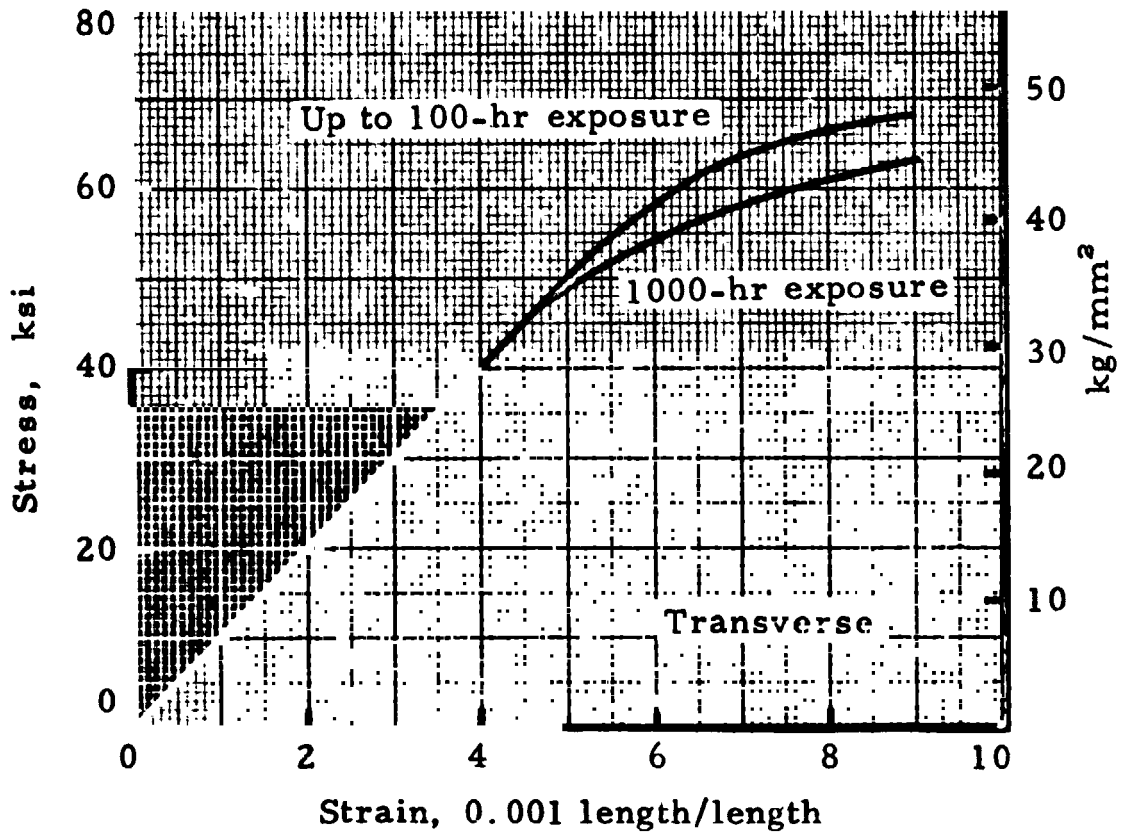
FIGURE 7.4222. — Typical compressive stress-strain curves for Clad 7075-T6 sheet at 200° F (93° C).
