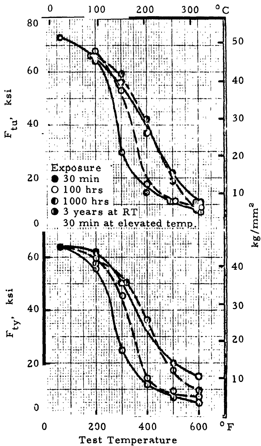
FIGURE 7.4138. — Effect of exposure and test temperature on tensile properties of Clad 7075-T6; thickness, 0.064 inch (1.625 mm). (Ref. 7.17)
