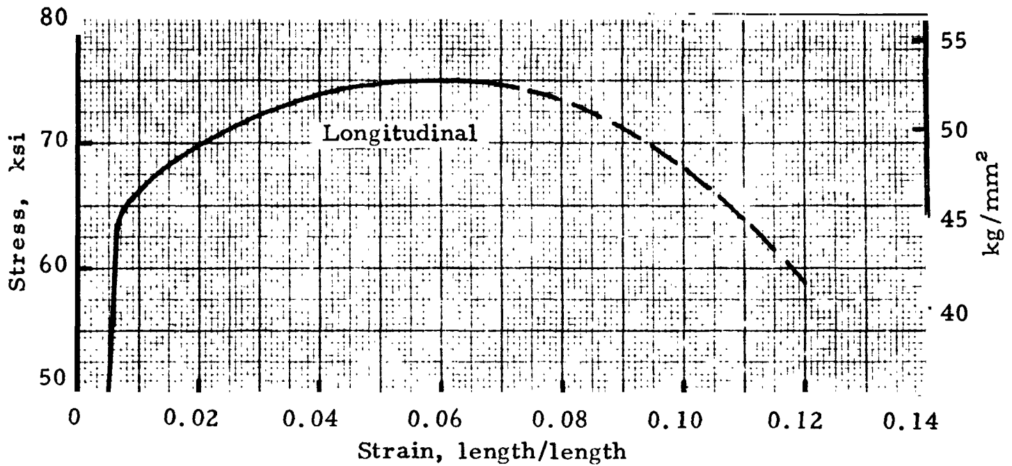
FIGURE 7.4123. — Typical tensile stress-strain curve (full-range) for 7075-T7351 extrusions (0.500-1.499 in, 12.7-38.1 mm) at room temperature. (Ref. 7.5)
