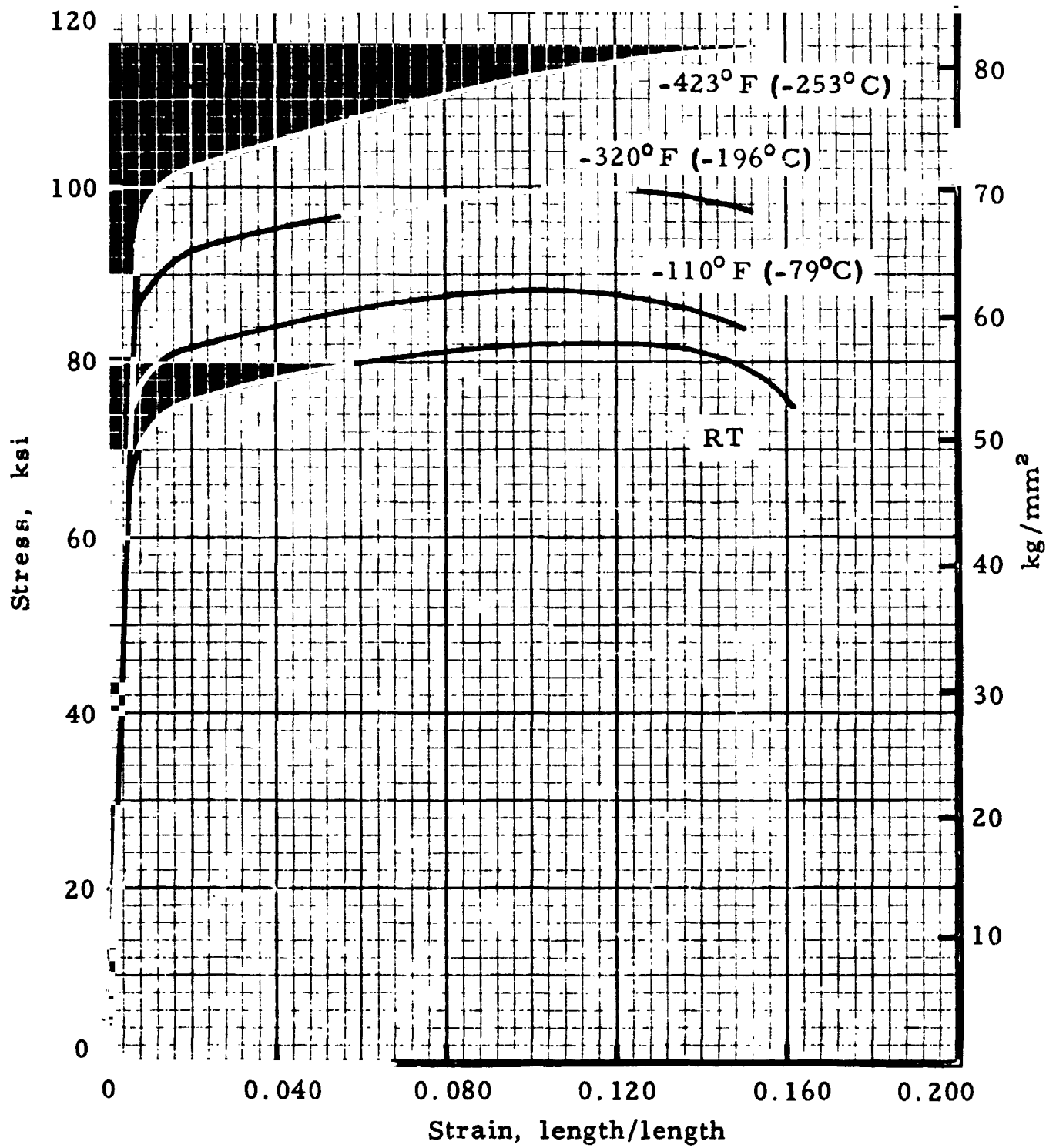
FIGURE 7.4127. -- Stress-strain curves for 7075-T6 bar at low temperatures; thickness, 0.750 inch (19.05 mm). (Ref. 7.14)
