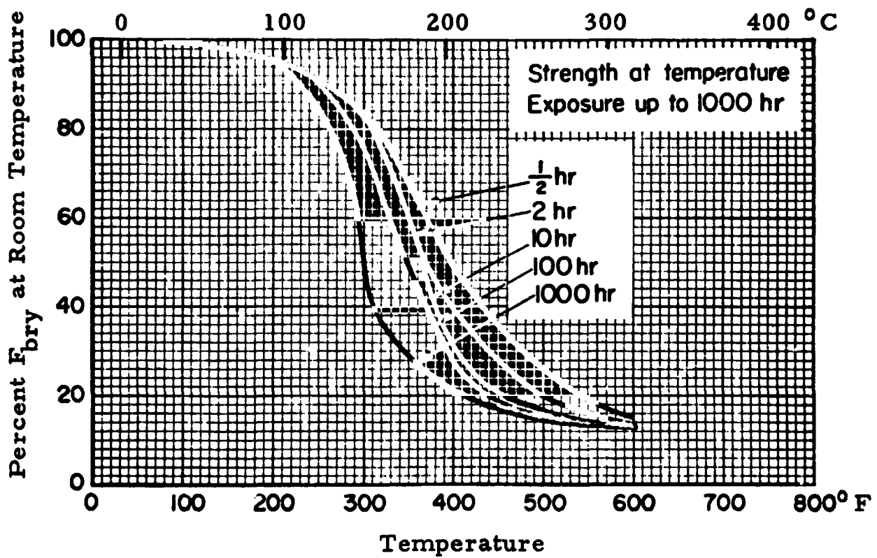
FIGURE 7.4520. — Effect of temperature on the bearing yield strength of 7075-T6 (all products).
