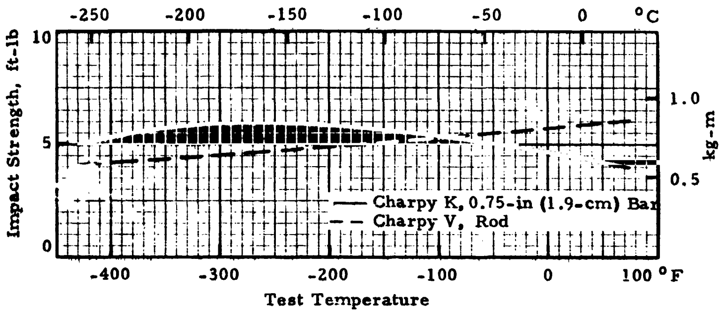
FIGURE 8.31. — Low temperature impact strength of 7075-T6 bar and rod.
