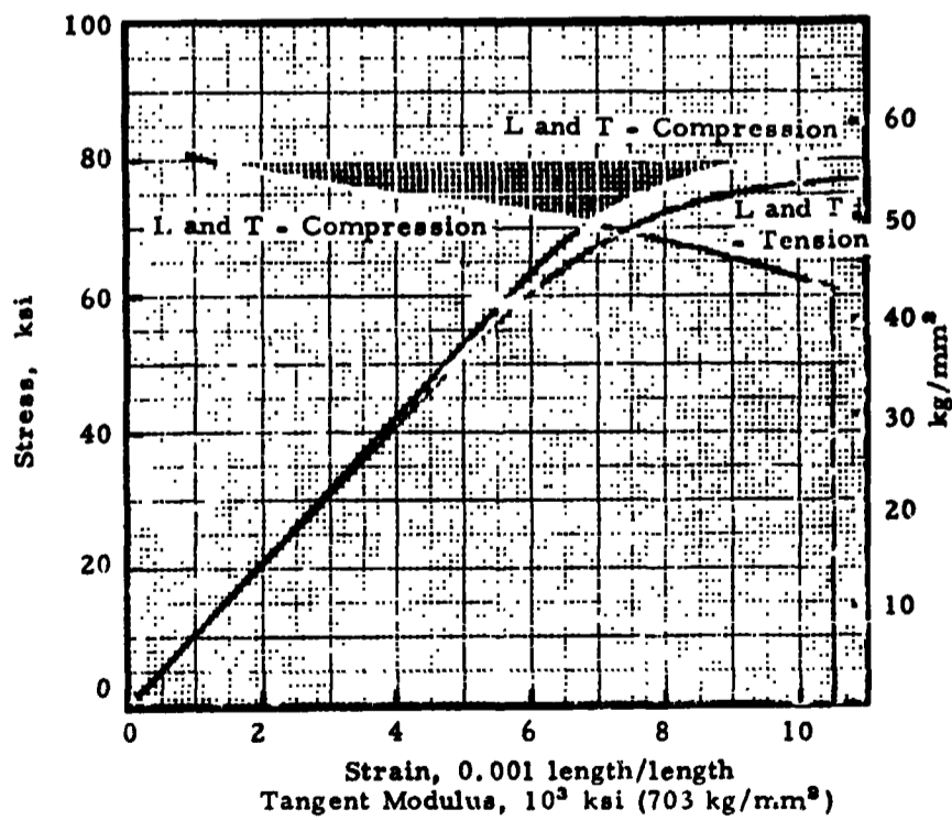
FIGURE 7.253. - Typical tensile and compressive stress-strain and tangent-modulus curves for 7075-T6 plate at room temperature; thickness, 0.250-2.000 inches (6.35-50.8 mm). (Ref. 7.5)
