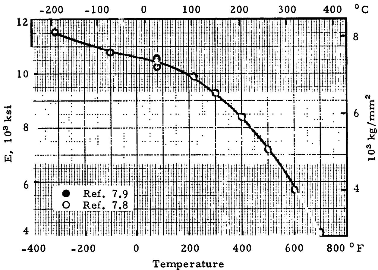
FIGURE 7.225. — Modulus of elasticity (static) of 7075-T6 bar at various temperatures.
