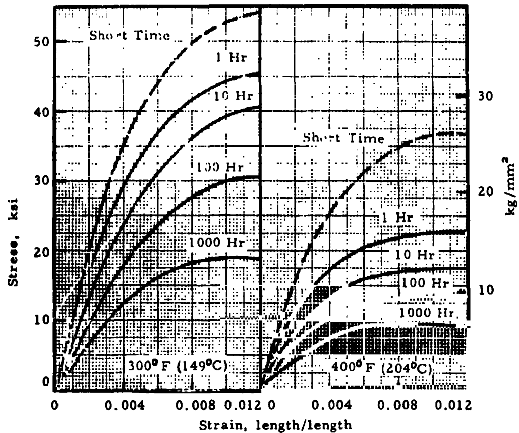
FIGURE 8.422. — Isochronous stress-strain curves (tension) at elevated temperatures for 7075-T6.
