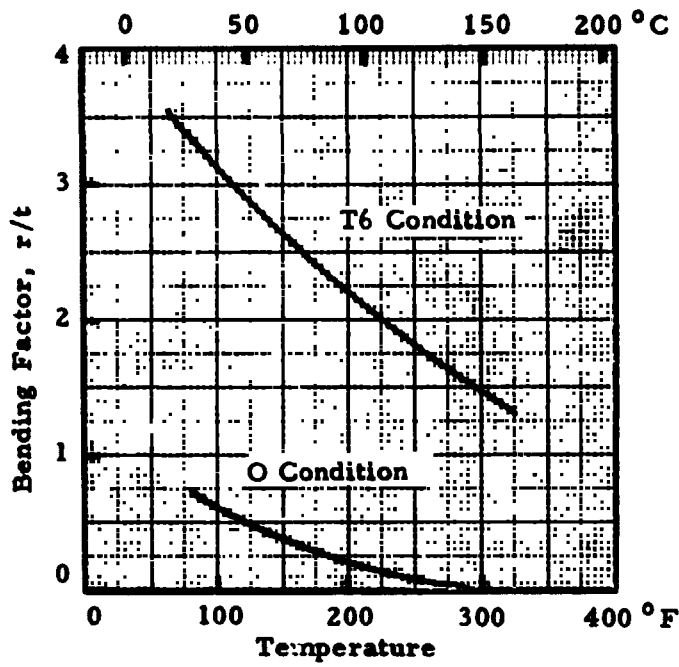
FIGURE 5.3. — Effect of forming temperature on bend factor in rubber forming of 7075 sheet in O and T6 conditions; thickness, 0.064 in (1.625 mm). (Ref. 5.15)
