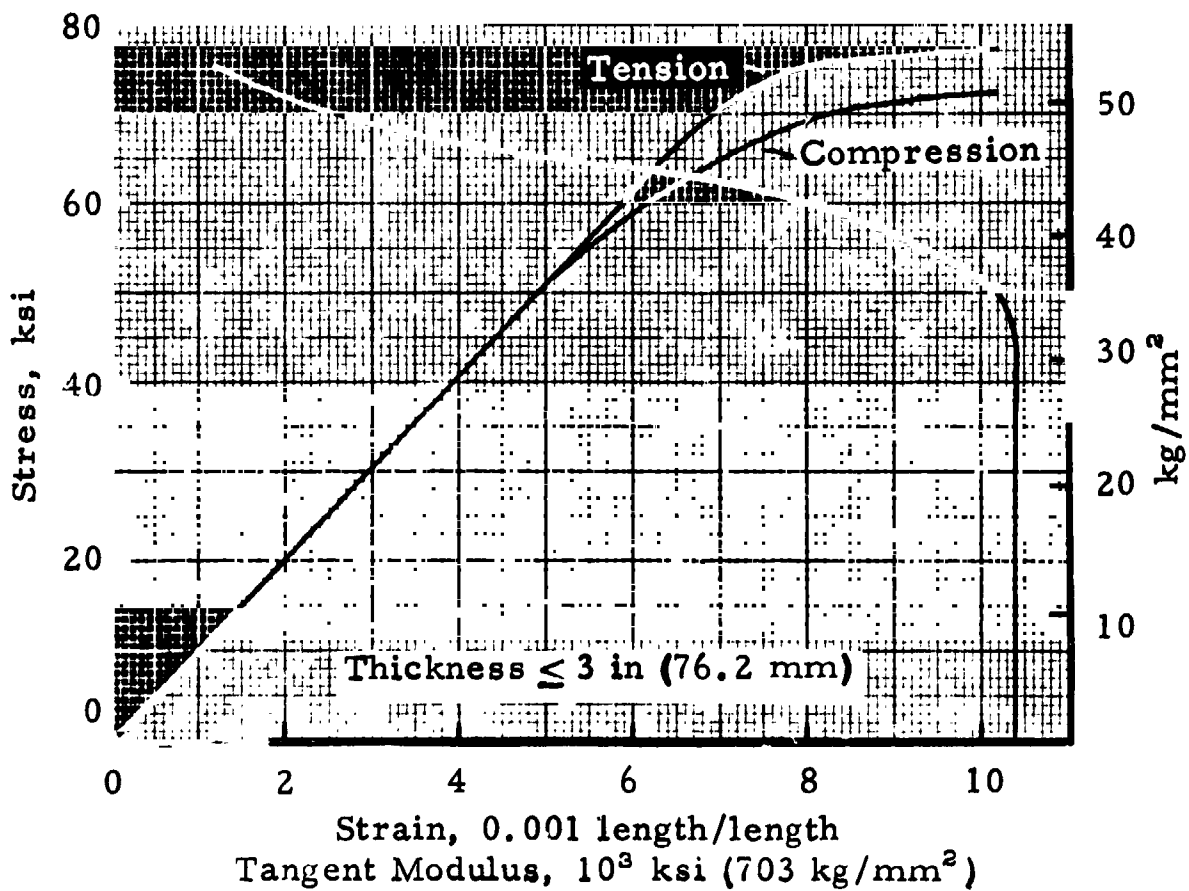
FIGURE 7.251. — Typical stress-strain and tangent-modulus curves (longitudinal) for 7075-T6 rolled bar, rod, and shapes at room temperature. (Ref. 7.5)
