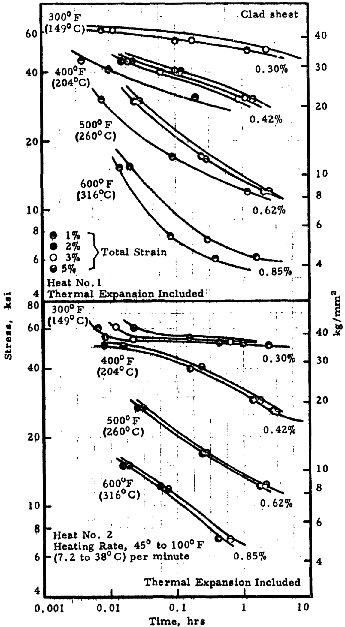
FIGURE 8.421. - Short-time total strain curves for 7075-T6 sheet at elevated temperatures; thickness, 0.064 inch (1.625 mm). (Ref. 8.5)
