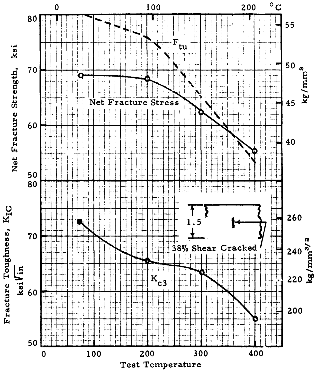
FIGURE 7.4621. — Net fracture stress and fracture toughness of 7075-T6 sheet at elevated temperatures; thickness, 0.063 inch (1.60 mm).
