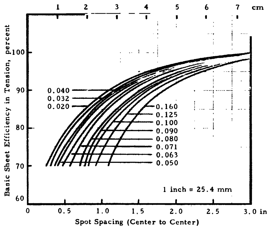
FIGURE 12.2. - Efficiency of the parent metal in tension for spotwelded aluminum alloys. (Ref. 12.6)
