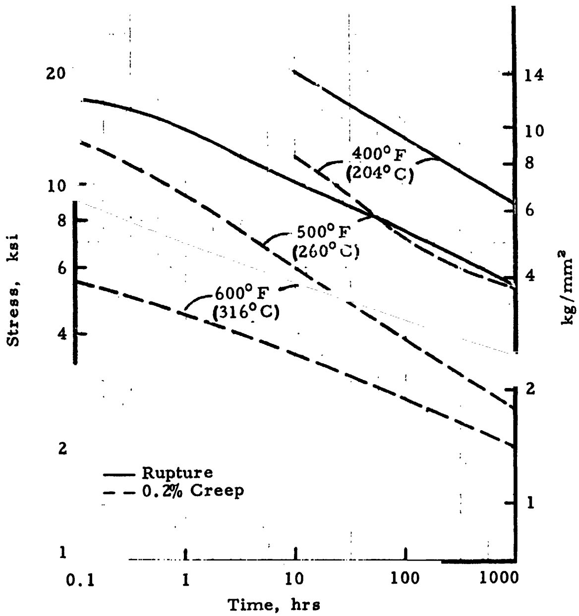
FIGURE 8.413. — Creep and creep rupture curves for 7075-T73 products.
