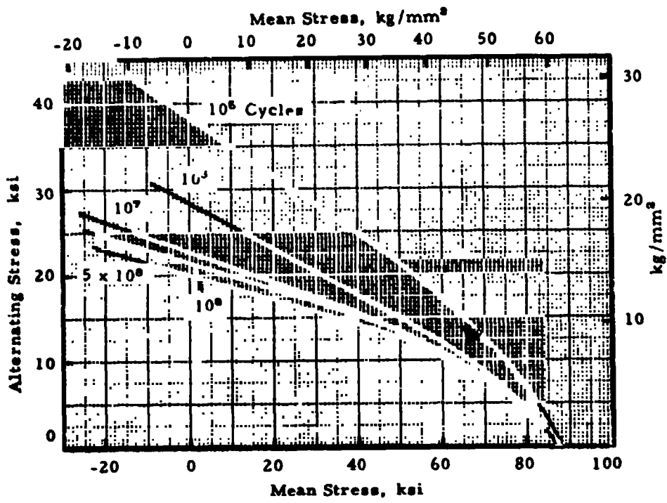
FIGURE 8.621. - Stress range diagram for 7075-T6 bar and extrusions.
