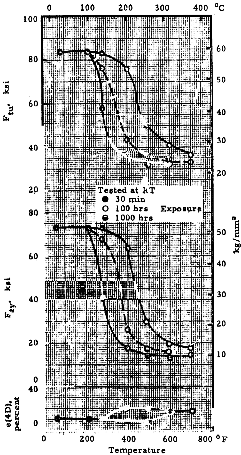
FIGURE 8.511. — Effect of exposure to elevated temperatures on room temperature tensile properties of 7075-T6.
