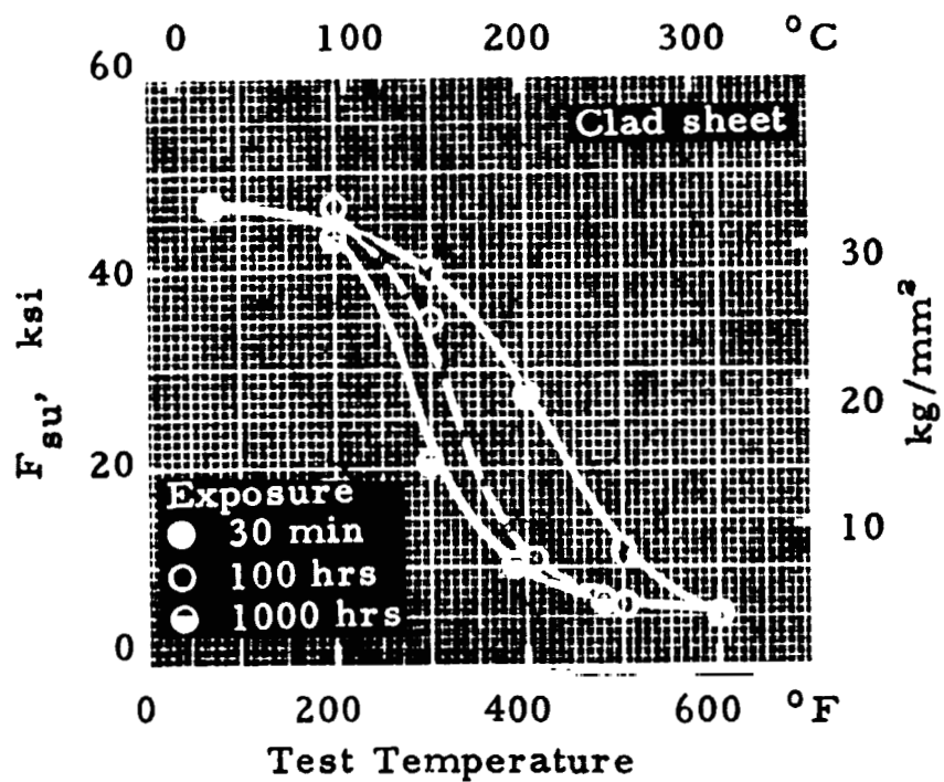
FIGURE 7.4419. — Effect of exposure and test temperature on shear strength of 7075-T6 sheet; thickness, 3/16 inch (4.76 mm).
