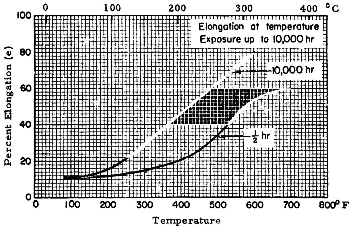
FIGURE 7.4134. — Effect of temperature on the elongation of 7075-T6 (all products except thick extrusions). (Ref. 7.5)
