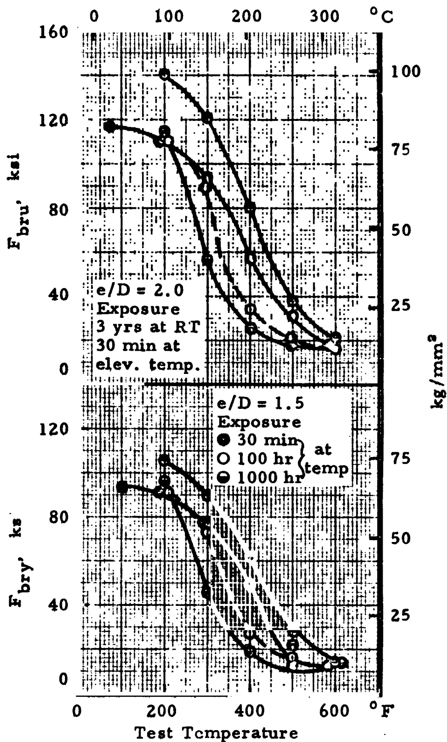
FIGURE 7.4518. — Effect of exposure and test temperature on bearing properties of Clad 7075-T6 sheet; thickness, 0.064 inch (1.625 mm).
