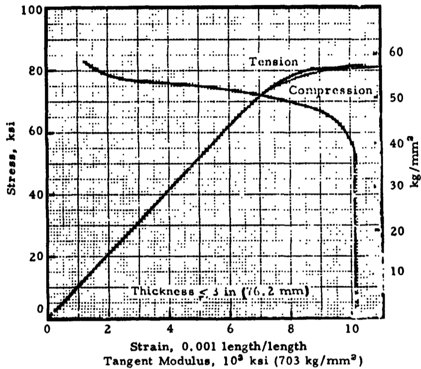
FIGURE 7.252. - Typical stress-strain and tangent-modulus curves (longitudinal) for 7075-T6 extrusions at room temperature. (Ref. 7.5)
