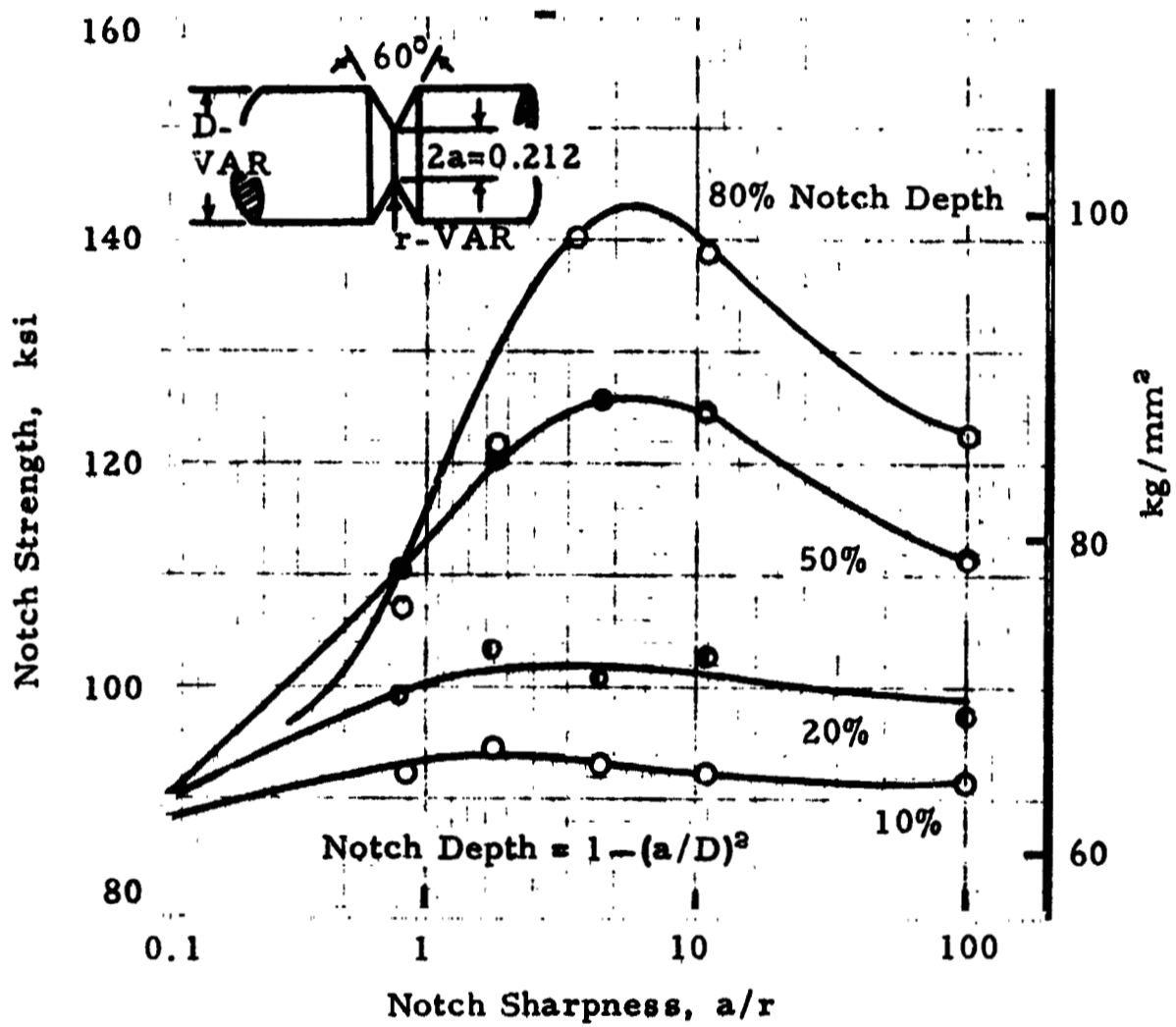
FIGURE 7.4611. — Effect of notch sharpness and notch depth on notch strength of 7075-T6 bar (3/4 inch, 19 mm).
