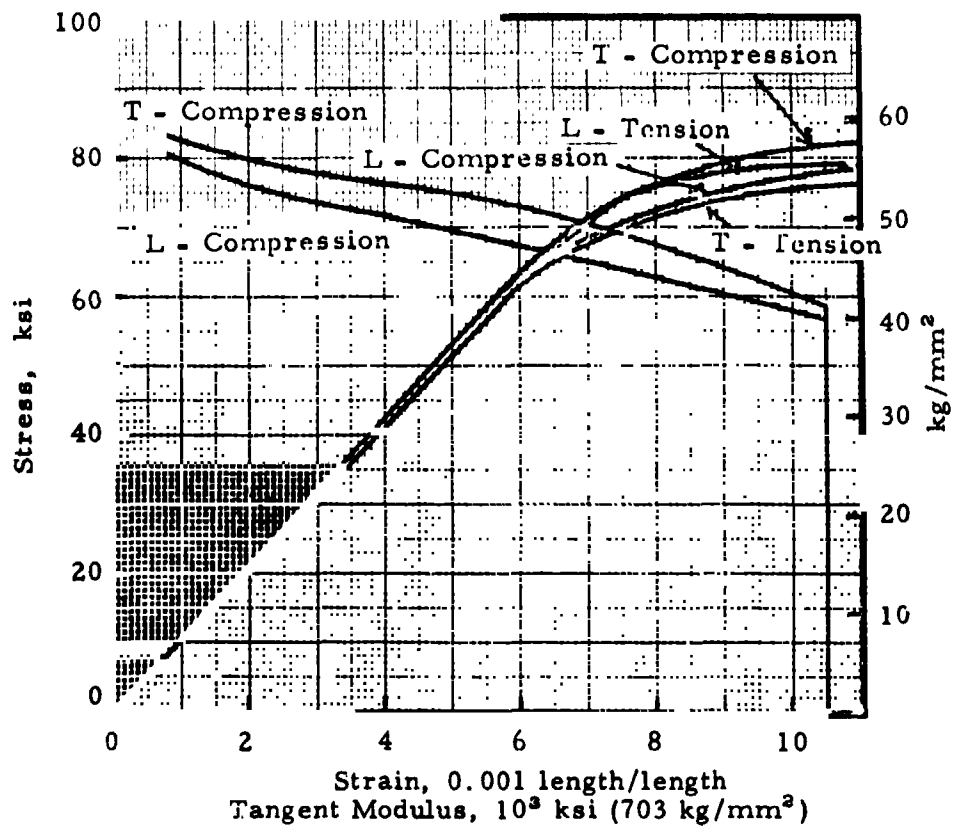
FIGURE 7.254. — Typical tensile and compressive stress-strain and tangent-modulus curves for 7075-T651 plate at room temperature; thickness, 0.250-2.000 inches (6.35-50.8 mm). (Ref. 7.5)
