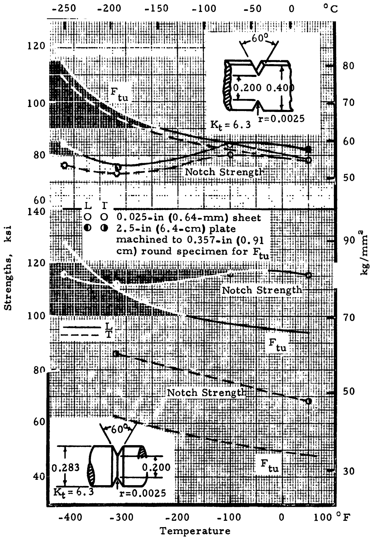
FIGURE 7.4612. — Effect of low temperatures on notch strength of 7075-T6 sheet and plate.
