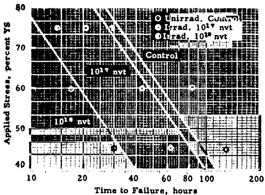
FIGURE 10.23. — Applied stress vs stress-corrosion time to failure in alternate-immersion (3.5% NaCl) tests on irradiated 7075-T6 specimens. (Ref. 10.17)
