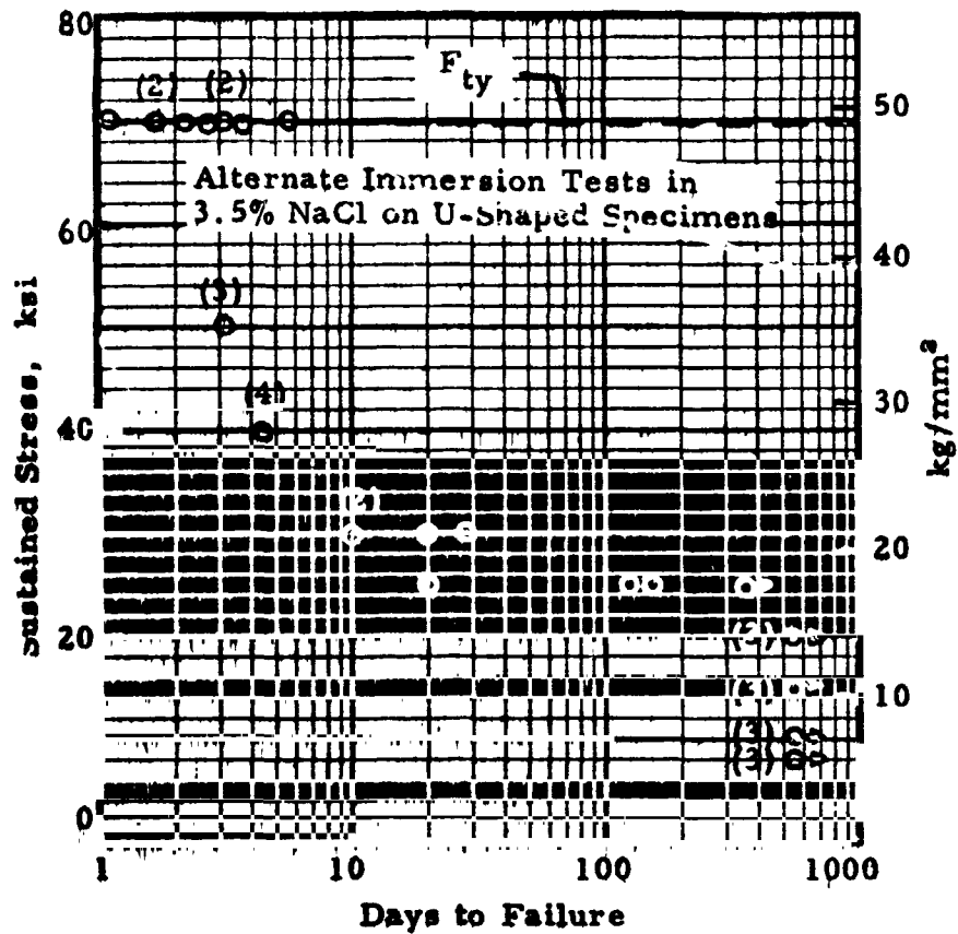
FIGURE 10.22. — Results of stress corrosion tests on 7075-T6 plate; thickness, 1.5 in (38.1 mm). (Ref. 10.10)
