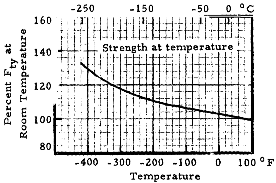
FIGURE 7.4137. — Effect of low temperature on the tensile yield strength of 7075-T6 (all products). (Ref. 7.5)
