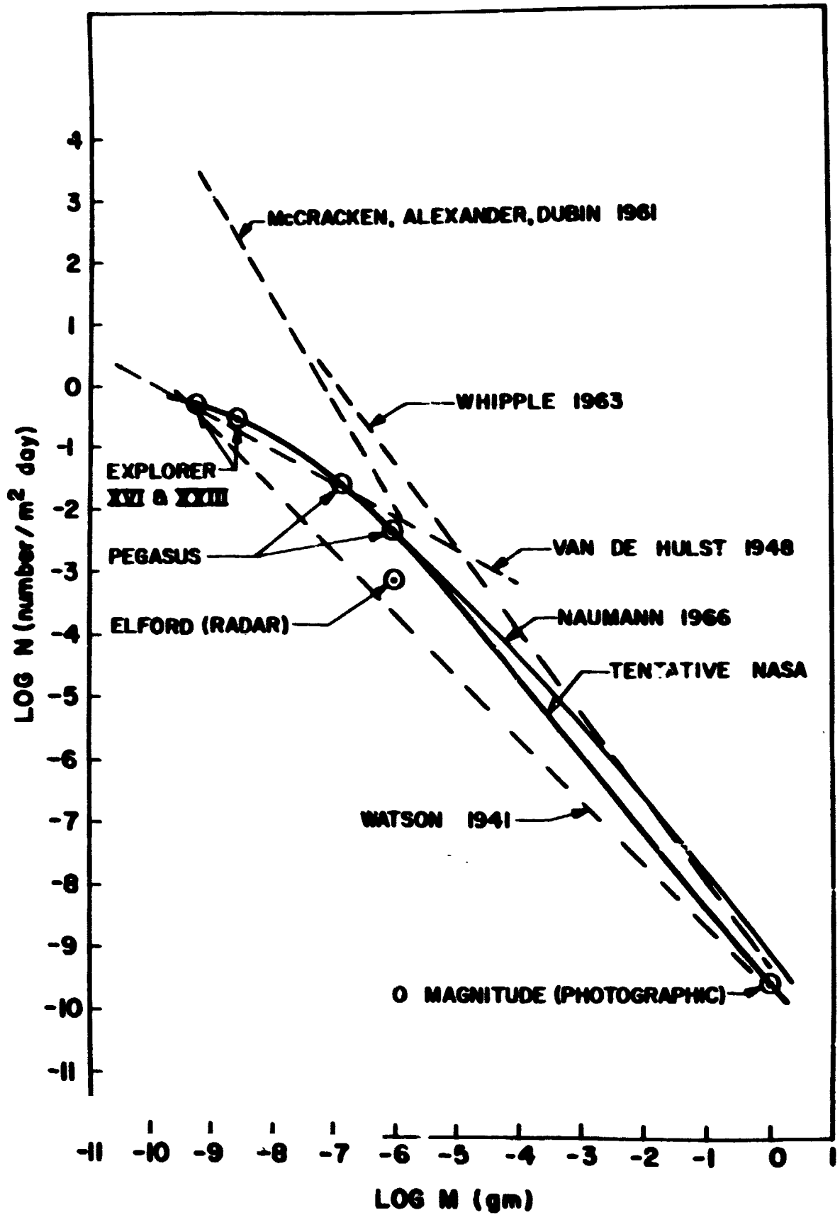
FIGURE 6.1. - Various estimates of meteoroid mass influx. (Ref. 6.3)
