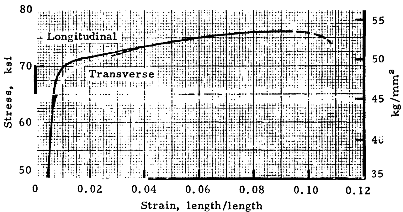
FIGURE 7.4124. — Typical tensile stress-strain curve (full-range) for Clad 7075-T6 sheet at room temperature. (Ref. 7.5)
