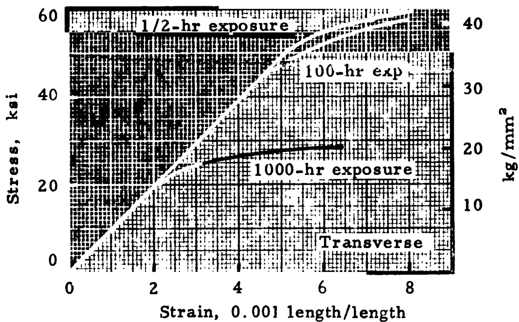
FIGURE 7.4223. — Typical compressive stress-strain curves for Clad 7075-T6 sheet at 300° F (149° C).
