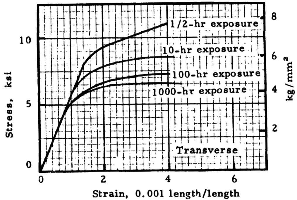
FIGURE 7.226. — Typical compressive stress-strain curves for Clad 7075-T6 sheet at 600°F (316°C). (Ref. 7.5)
