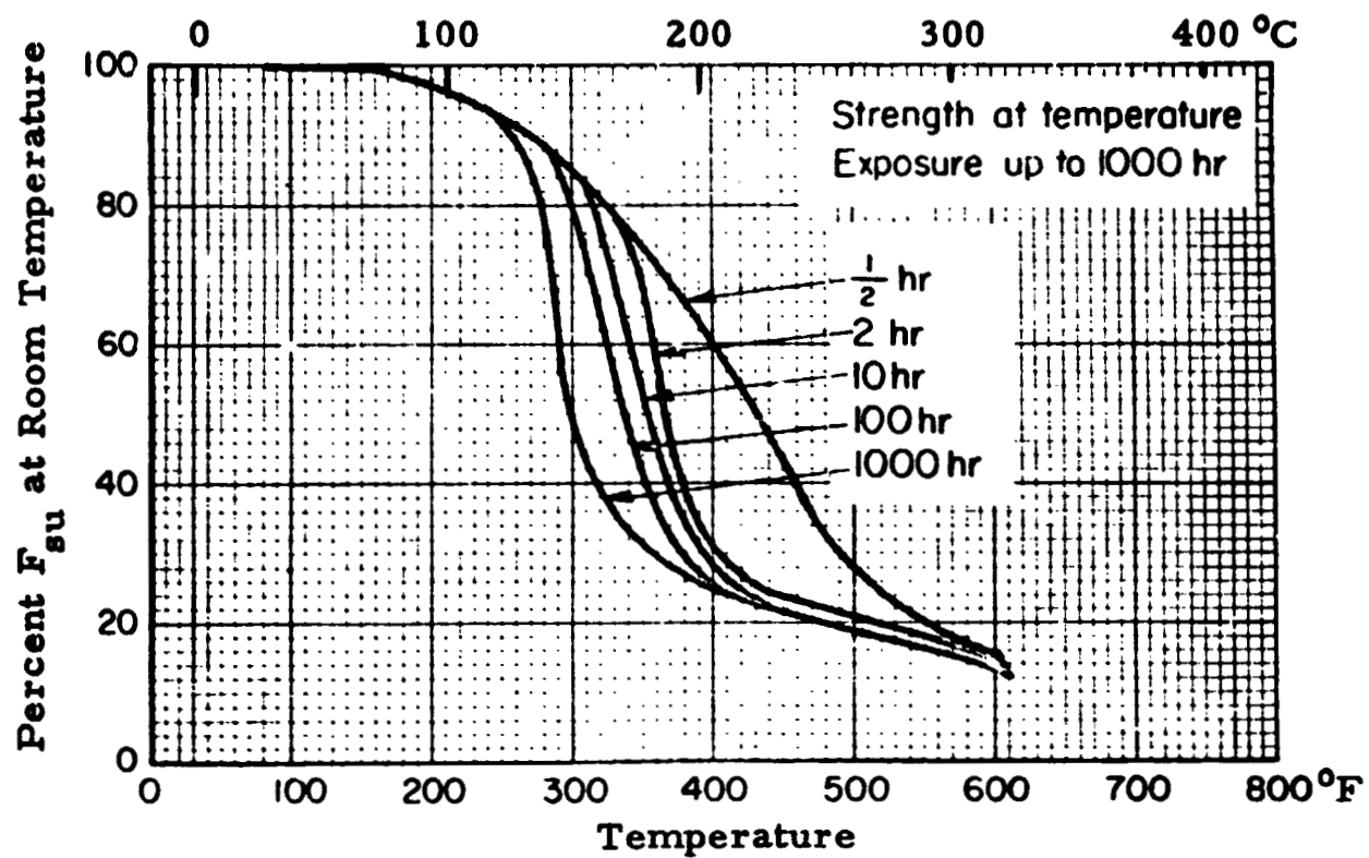
FIGURE 7.4418. — Effect of temperature on the ultimate shear strength of 7075-T6 (all products).
