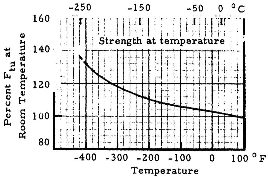
FIGURE 7.4136. — Effect of low temperature on the ultimate tensile strength of 7075-T6 (all products). (Ref. 7.5)
