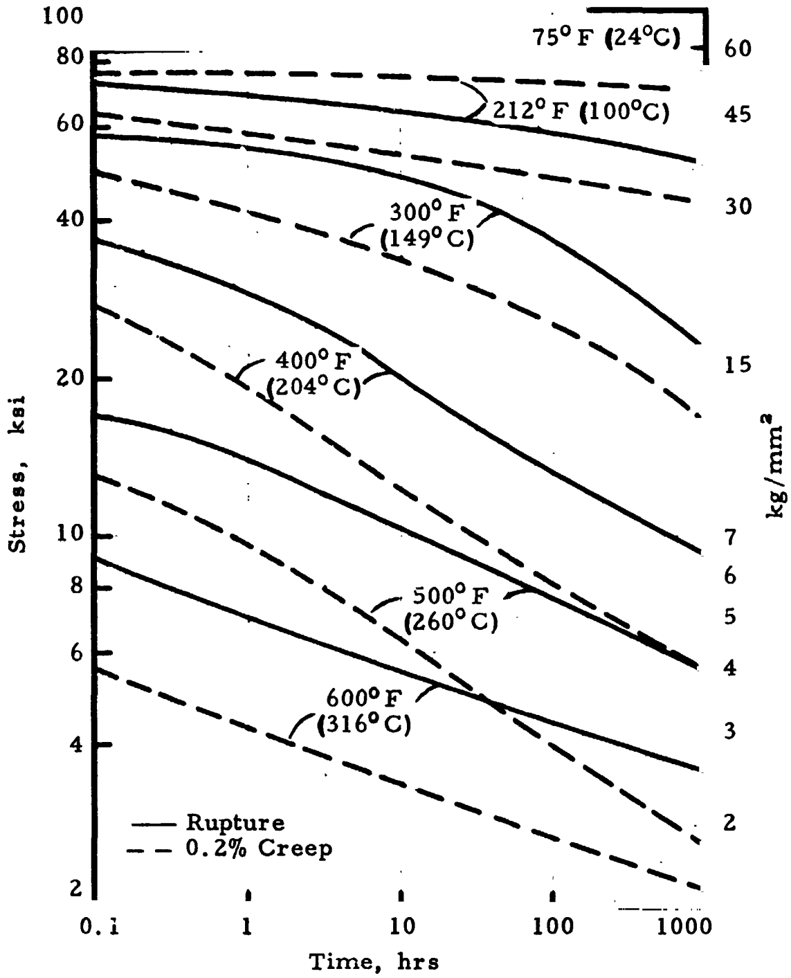
FIGURE 8.411. - Creep and creep rupture curves for all 7075-T6 and -T651 products (except extrusions and forgings). (Ref. 8.13)
