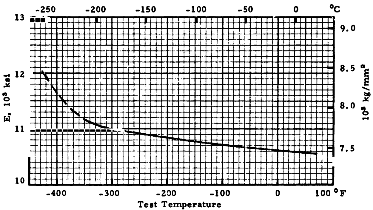
FIGURE 7.224. — Effect of low temperature on modulus of elasticity of 0.250-in (0.635-cm) 7075-T6 sheet. (Ref. 7.7)
