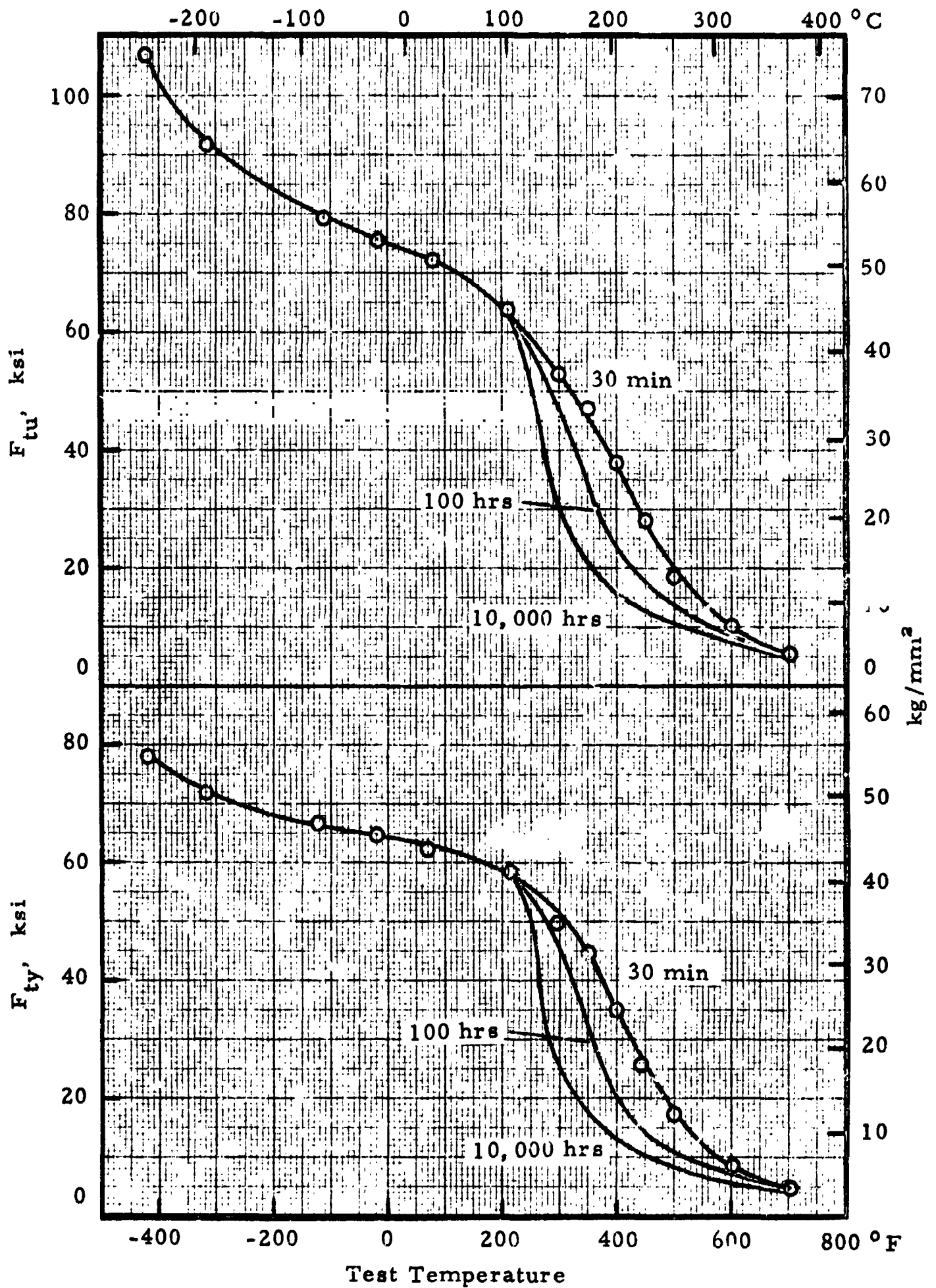
FIGURE 7.4139. — Effect of test temperature on tensile properties of 7075-T73 (typical data).
