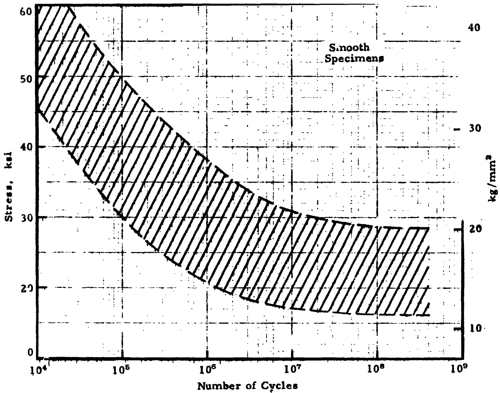
FIGURE 8.615. — Envelope of rotating beam S-N fatigue data points for 7075 plate, rod, and forgings in T73, T7351, and T6 conditions.
