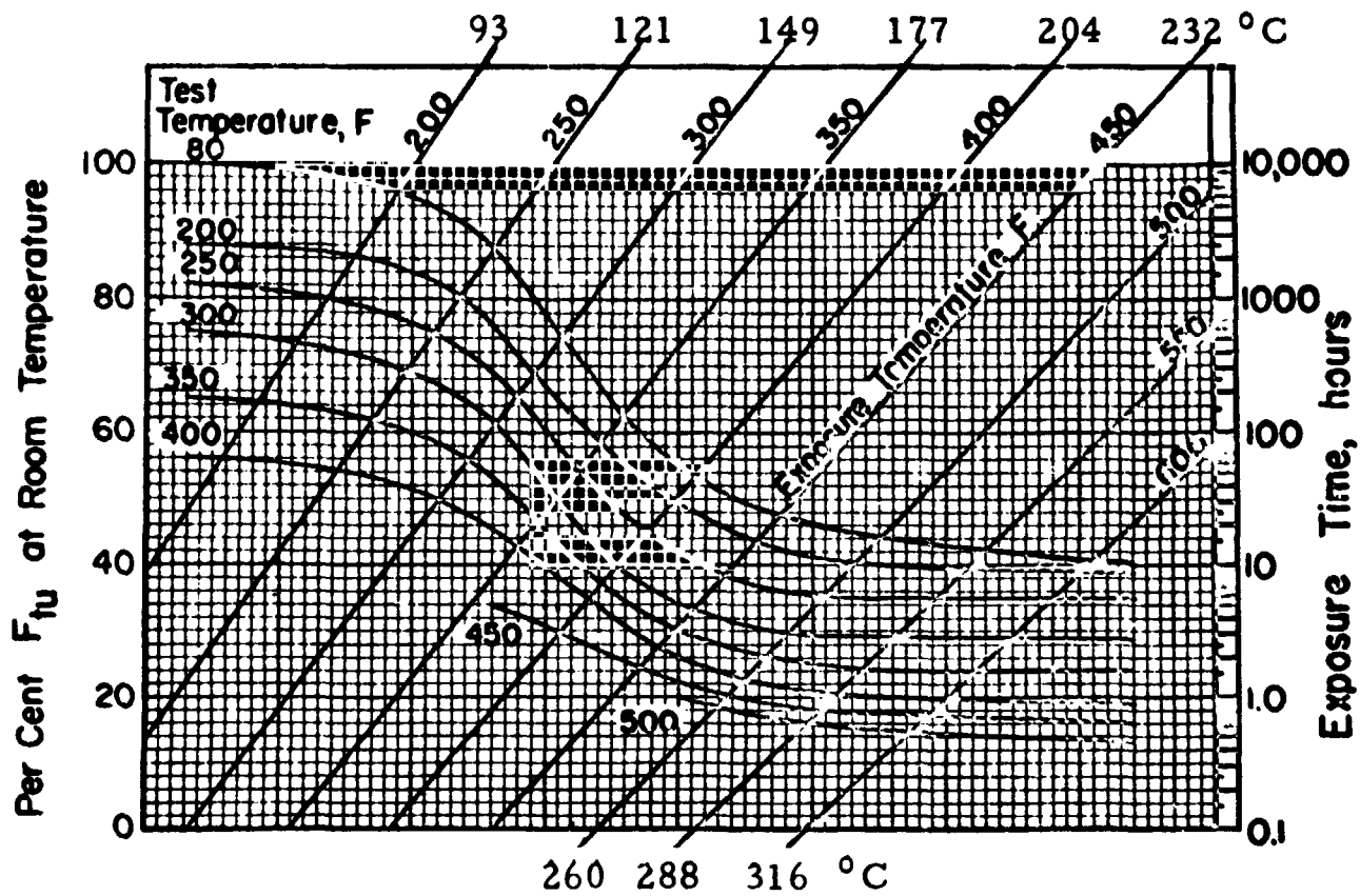
FIGURE 7.4132. — Effect of temperature on the ultimate tensile strength of 7075-T6 (all products). (Ref. 7.5)
