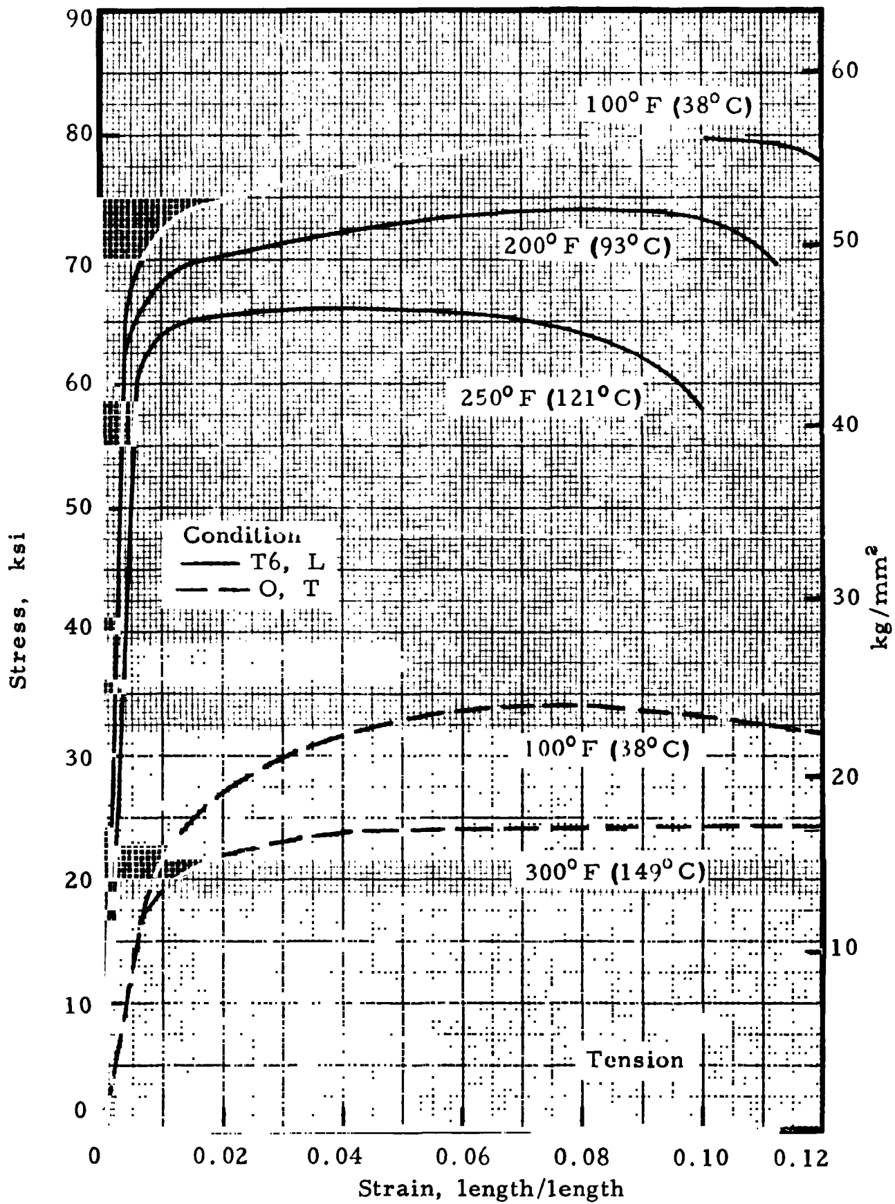
FIGURE 7.4126. — Complete stress-strain curves for Clad 7075 sheet in O and T6 conditions at room and elevated temperatures; thickness, 0.064 inch (1.625 mm). (Ref. 7.13)
