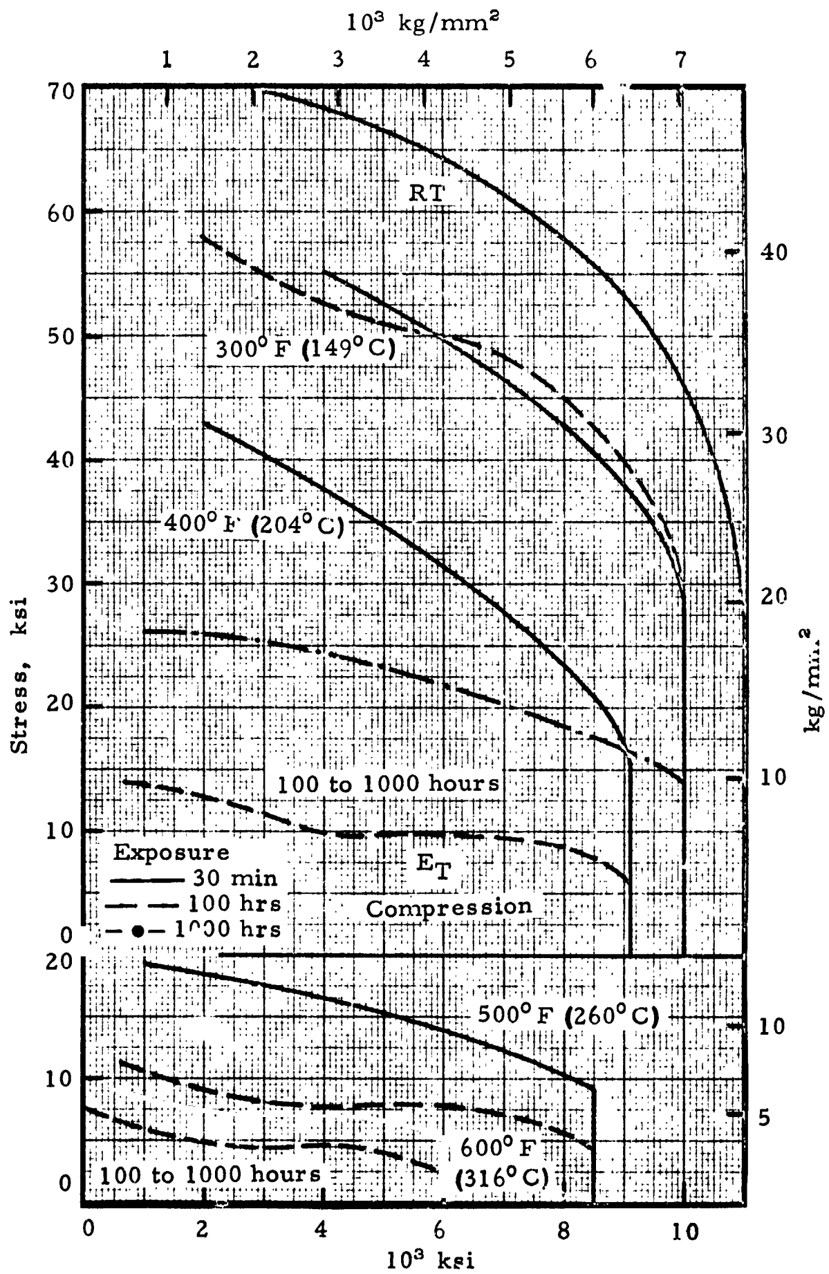
FIGURE 7.256. — Tangent modulus curves in compression for Clad 7075-T6 sheet at room and elevated temperatures; thickness, 0.064 in (1.625 mm).
