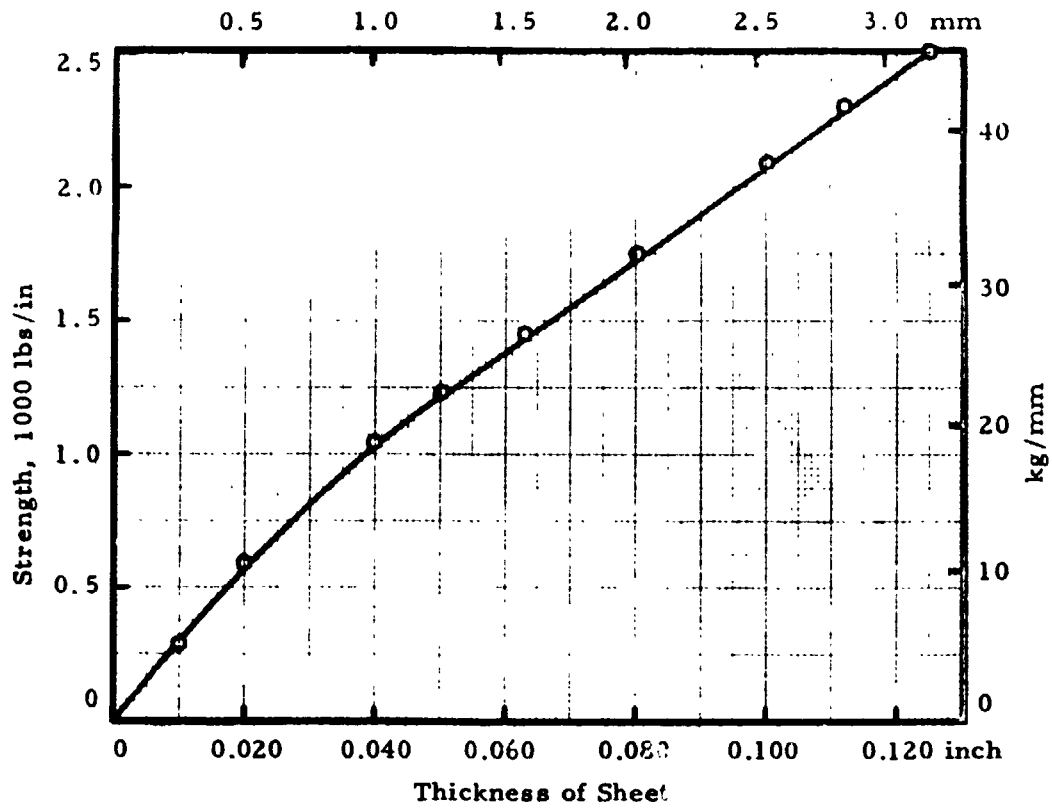
FIGURE 12.1. - Maximum static strength of typical single spotwelds in Clad 7075-T6 sheet of various thicknesses. (Ref. 12.6)
