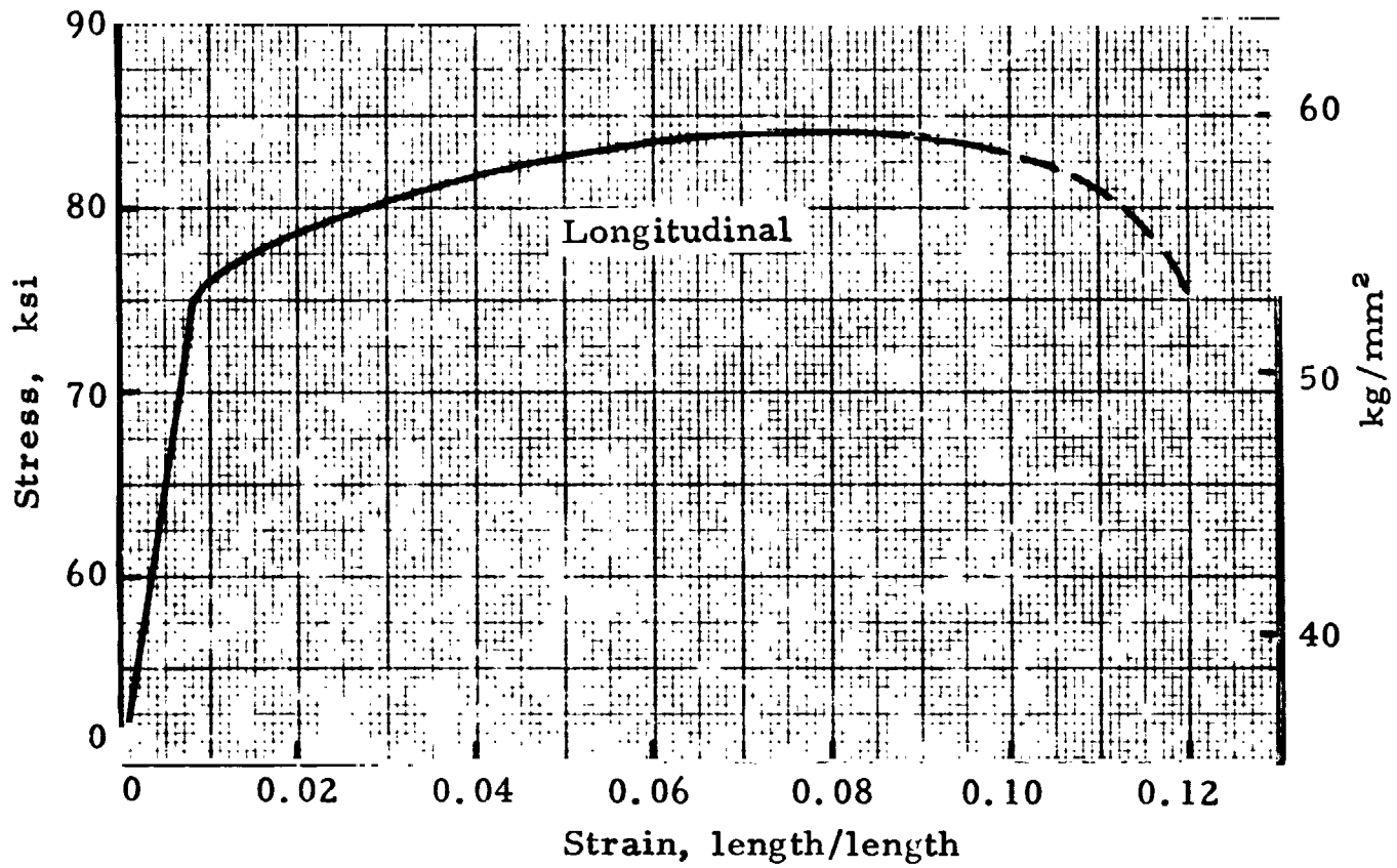
FIGURE 7.4121. — Typical tensile stress-strain curve (full-range) for 7075-T6 rolled or cold-finished bar at room temperature. (Ref. 7.5)
