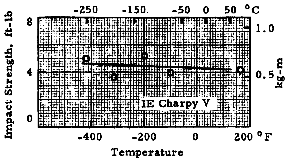
FIGURE 8.32. — Effect of test temperature on impact strength of 7075-T6.
