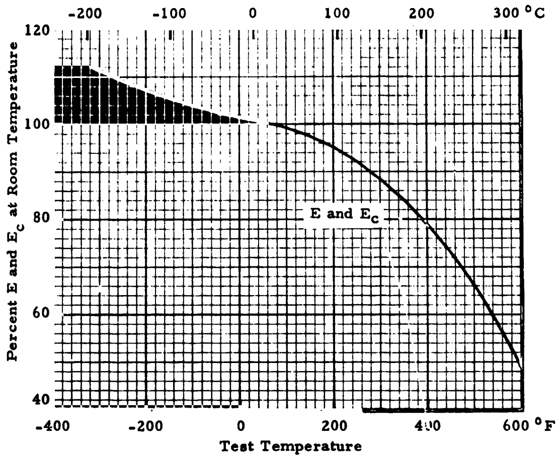
FIGURE 7.223. — Effect of temperature on E and E_c of aluminum 7075-T6. (Ref. 7.5)
