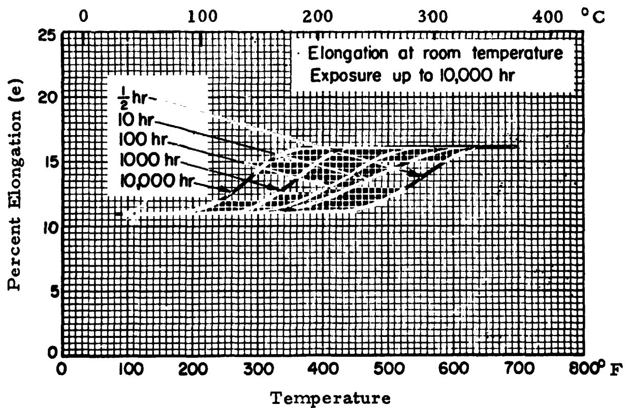
FIGURE 7.4135. — Effect of exposure at elevated temperatures on the elongation of 7075-T6 (all products except thick extrusions). (Ref. 7.5)
