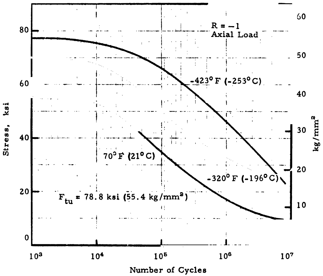
FIGURE 8.612. — S-N curves at low temperatures for 7075-T6 sheet; thickness, 0.100 inch (2.54 mm).
