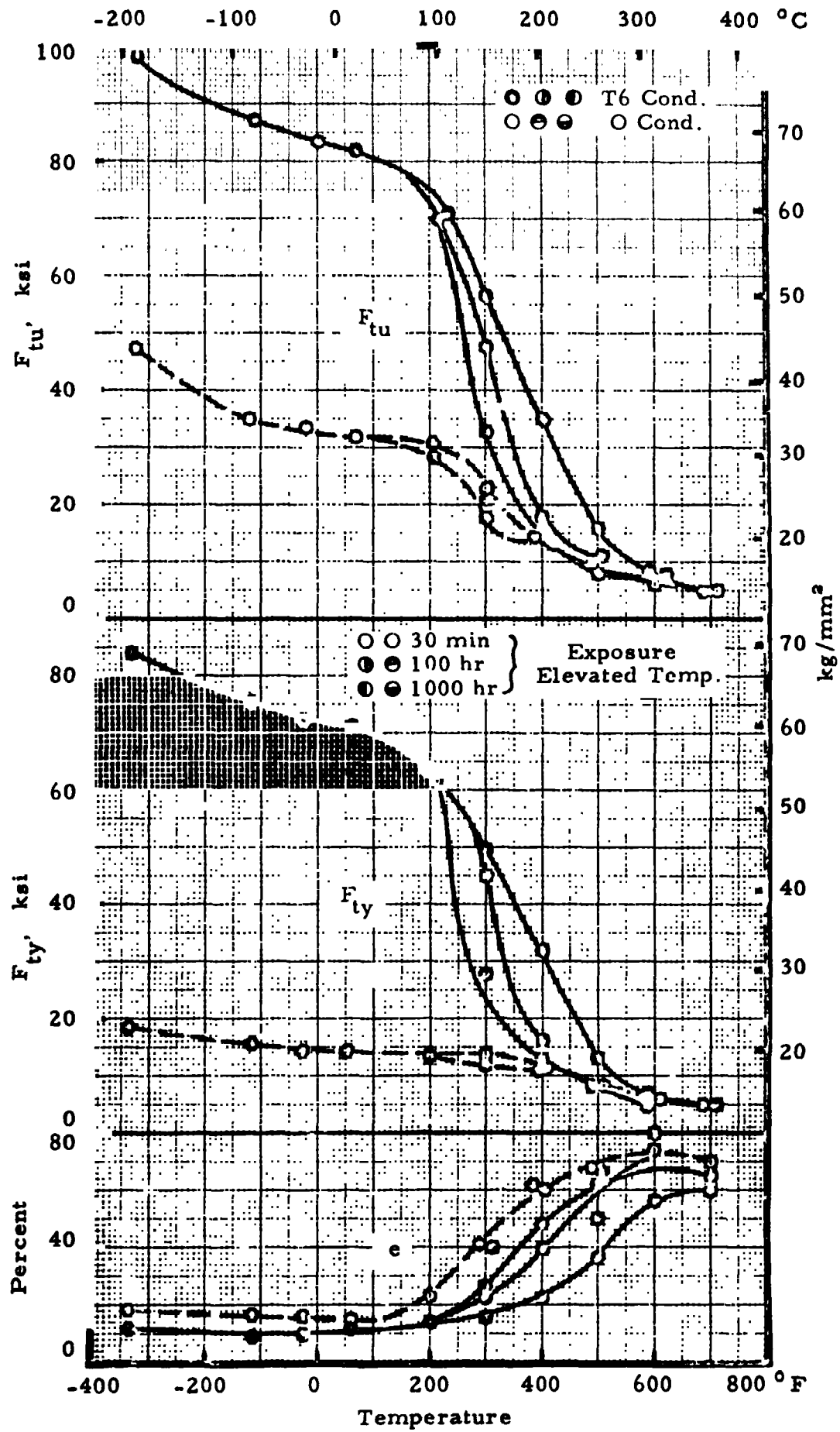
FIGURE 7.4131. - Effect of exposure and test temperature on tensile properties of 7075 in O and T6 conditions. (Refs. 7.13, 7.15)
