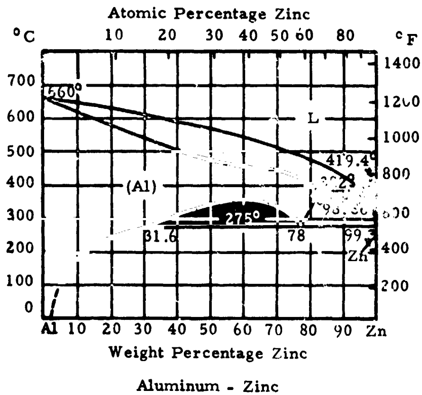
FIGURE 3.1. - Aluminum rich portion of binary equilibrium diagrams. (Ref. 3.3)
