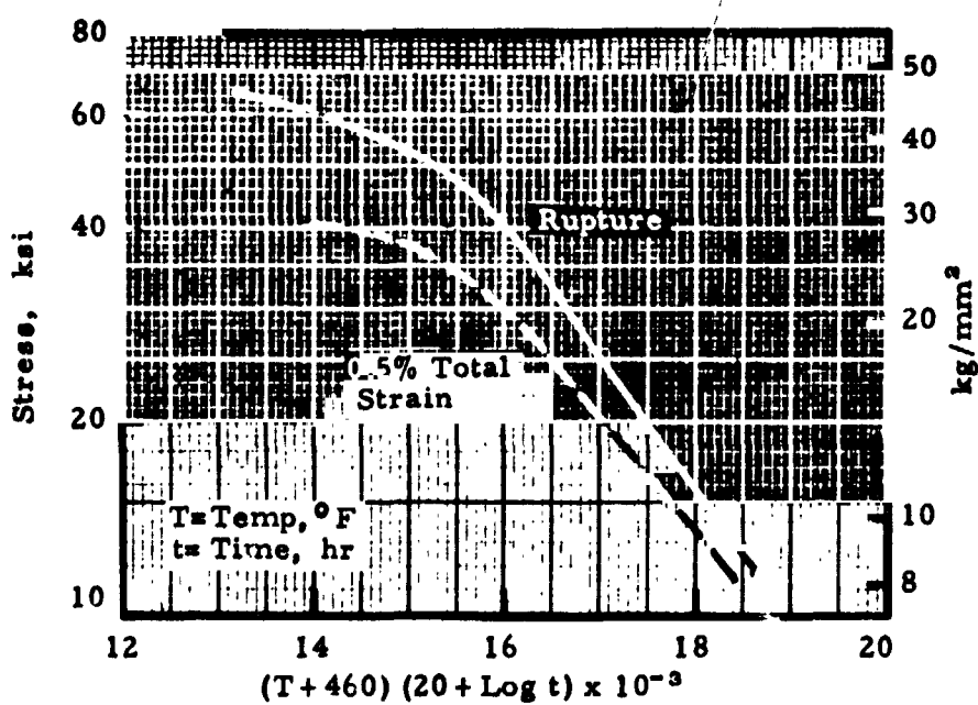
FIGURE 8.423. — Master curves for 0.5 percent total strain and creep rupture for Clad 7075-T6 sheet.
