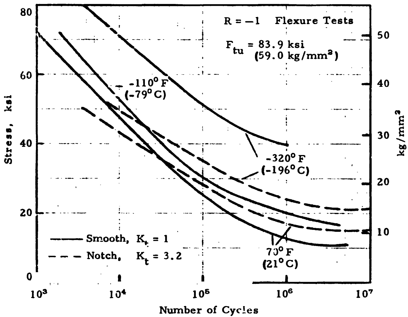
FIGURE 8.614. — Fatigue strength of smooth and notched 7075-T6 bar at low temperatures; thickness, 0.75 inch (19.1 mm).
