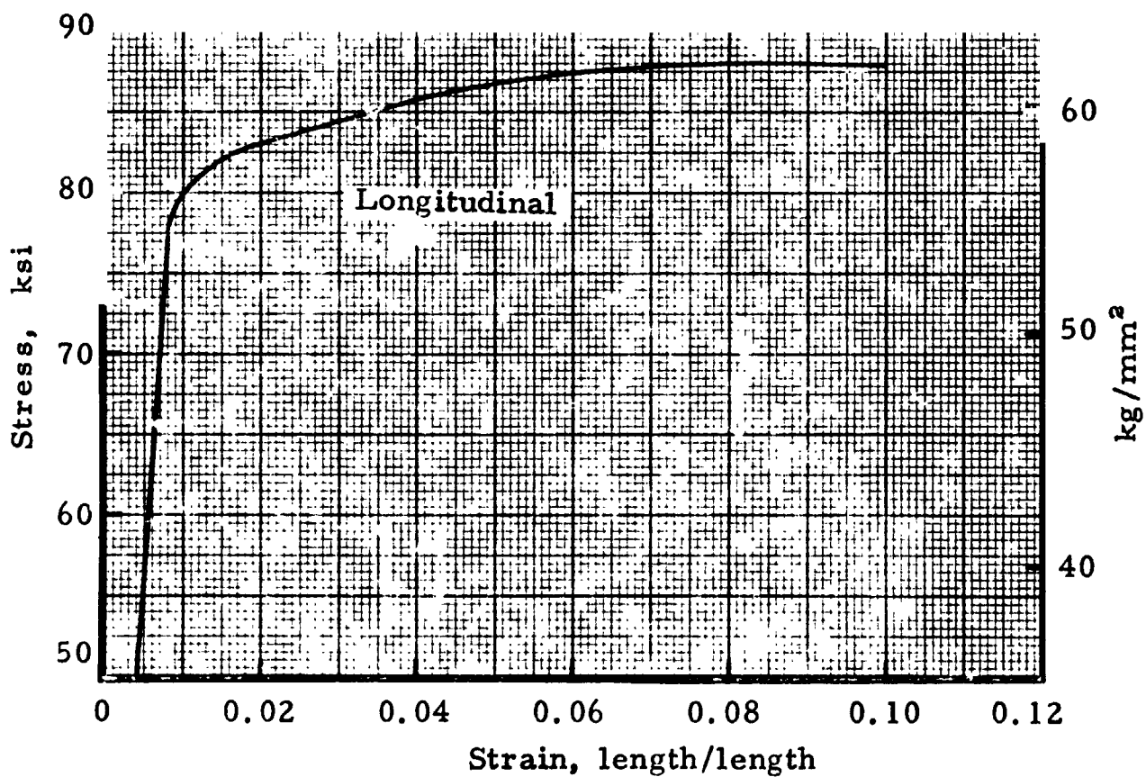
FIGURE 7.4122. — Typical tensile stress-strain curve (full-range) for 7075-T6 extrusions ( \leq 2.999 in, 76.17 mm) at room temperature. (Ref. 7.5)
