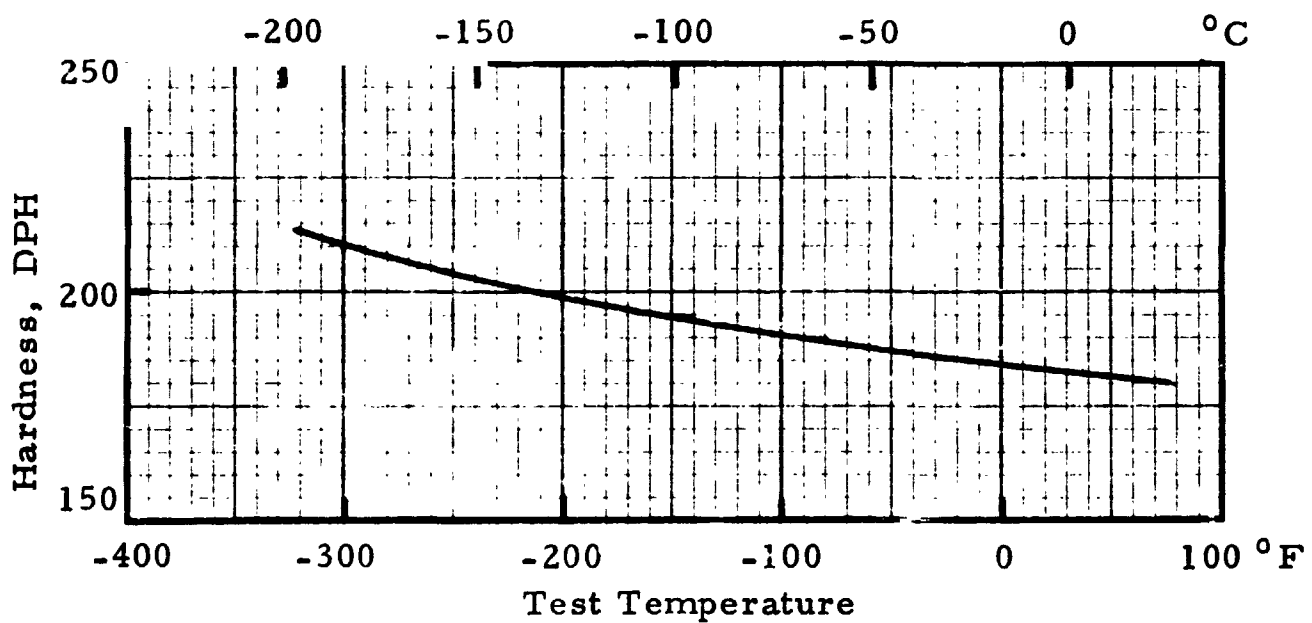
FIGURE 7.32. — Effect of low temperatures on hardness of 7075-T6 bar; thickness, 0.750 in (19.05 mm). (Ref. 7.11)
