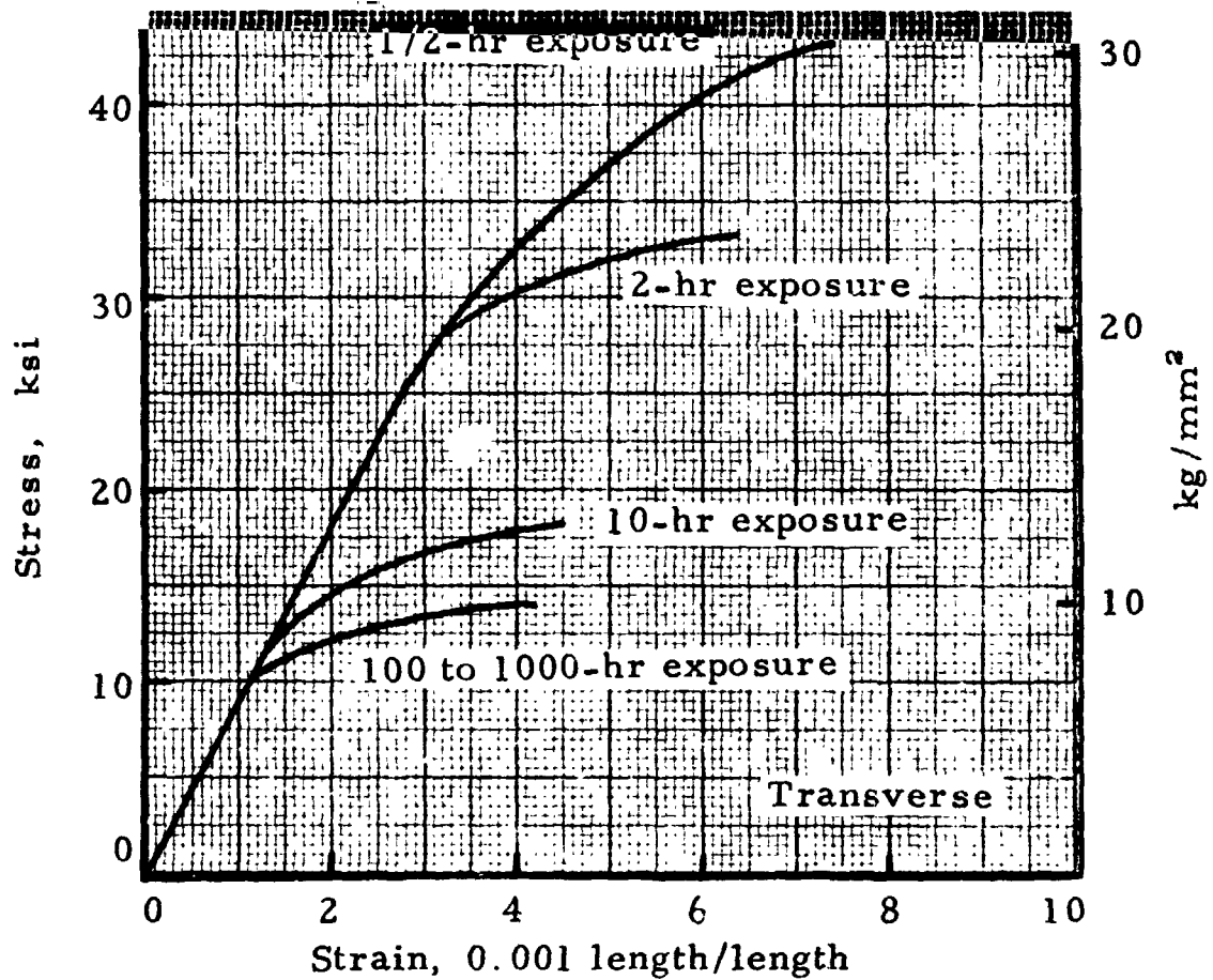
FIGURE 7.4224. — Typical compressive stress-strain curves for Clad 7075-T6 sheet at 400° F (204° C). (Ref. 7.5)
