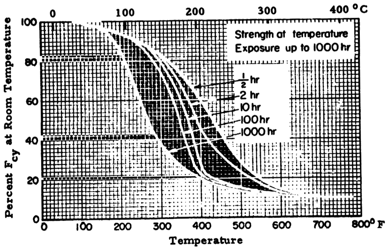
FIGURE 7.227. — Effect of temperature on the compressive yield strength of 7075-T6 (all products). (Ref. 7.5)
