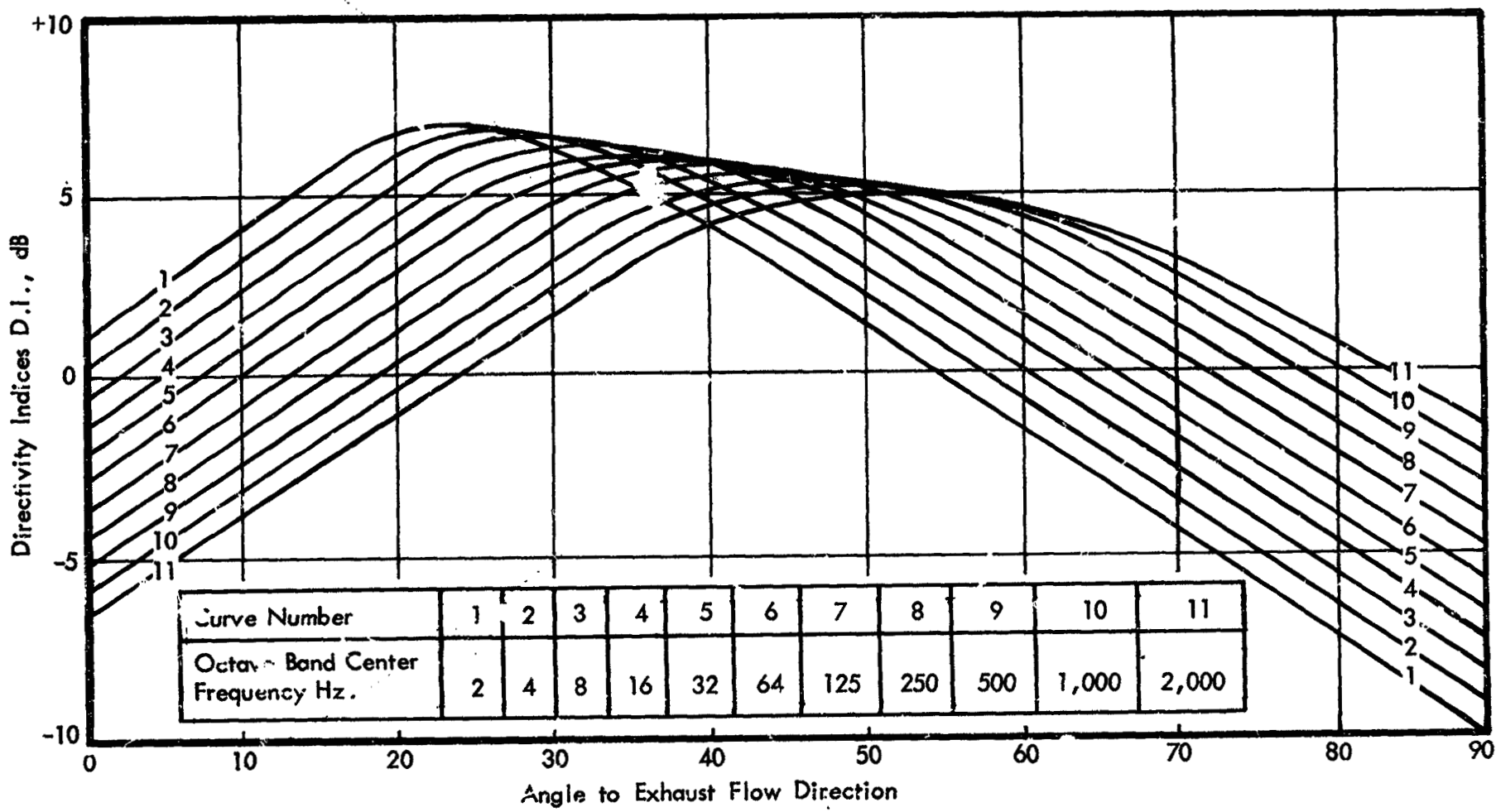
Figure 8. Directivity Curves
