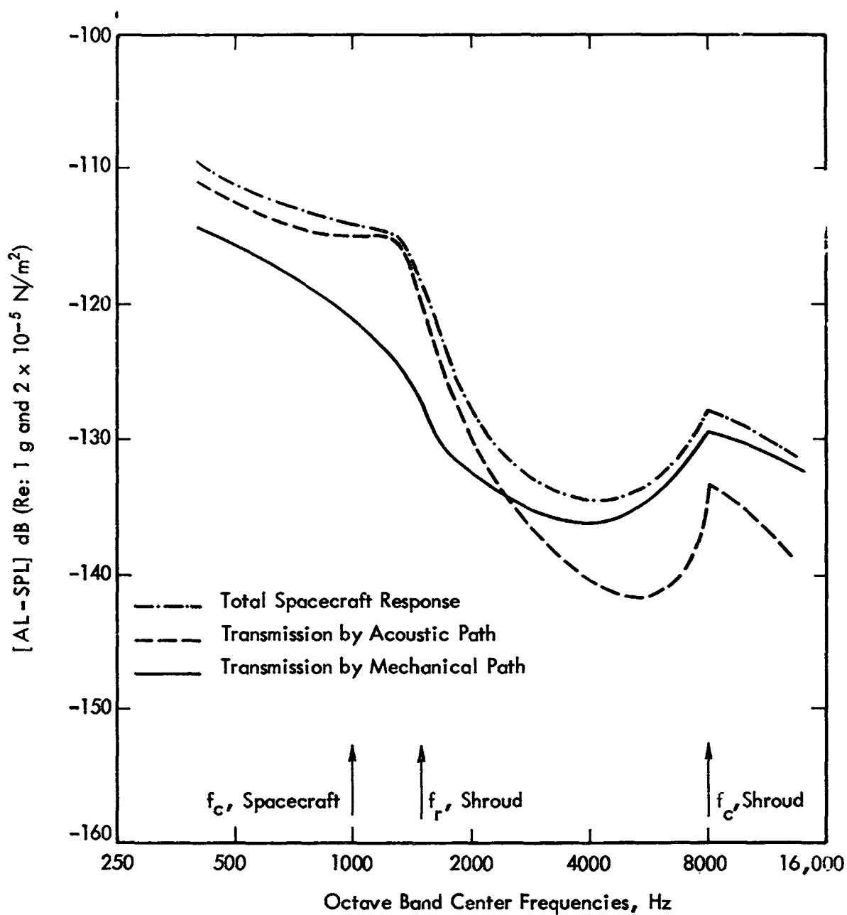
Figure 64. Predicted One-Third Octave Band Spacecraft Responses to Vibration Transmitted by the Different Paths; One-Half Scale Model of the Spacecraft-Shroud System from Reference 65
