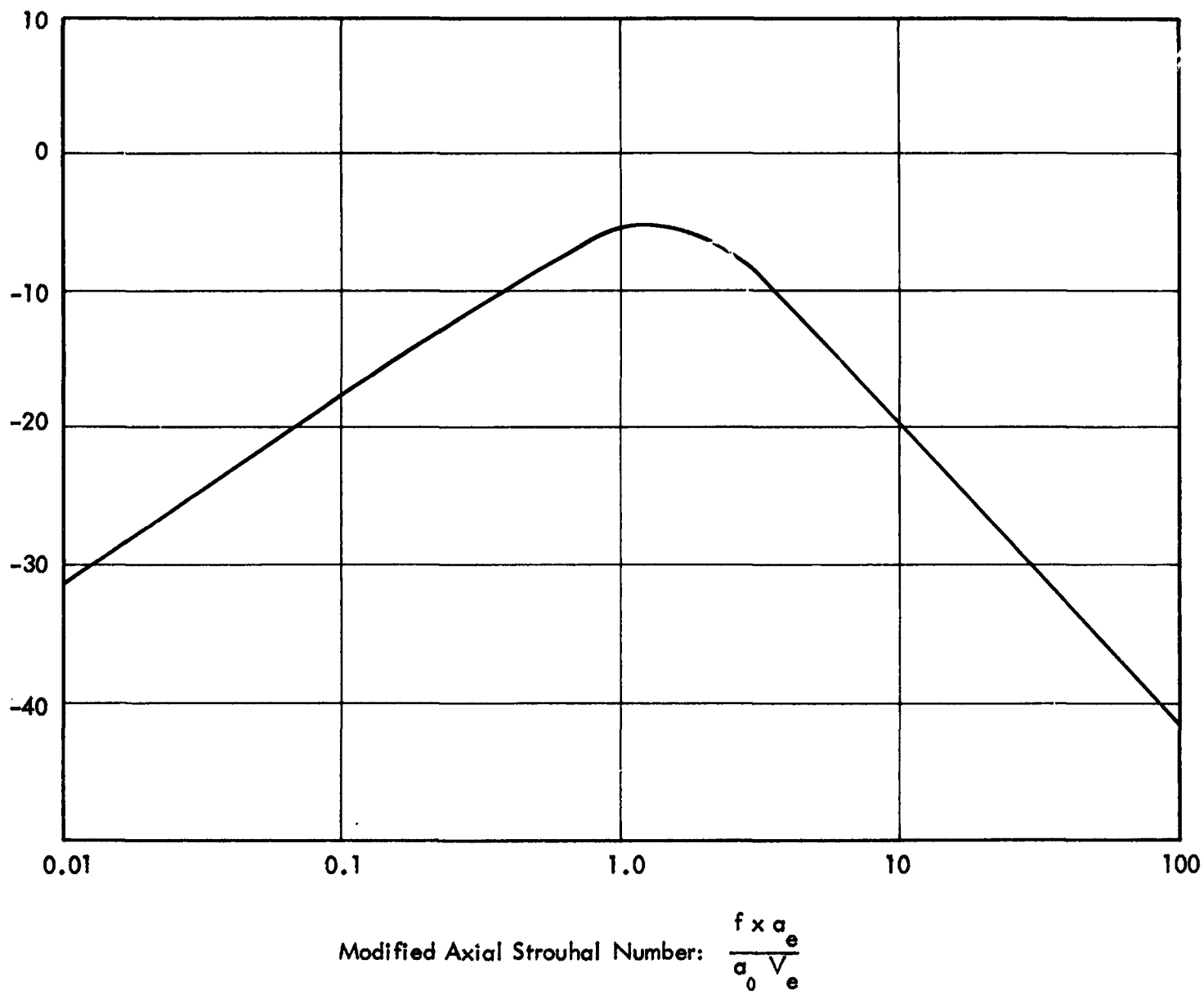
Figure 10: Normalized Power Spectrum with Distance Downstream; from Reference 15
