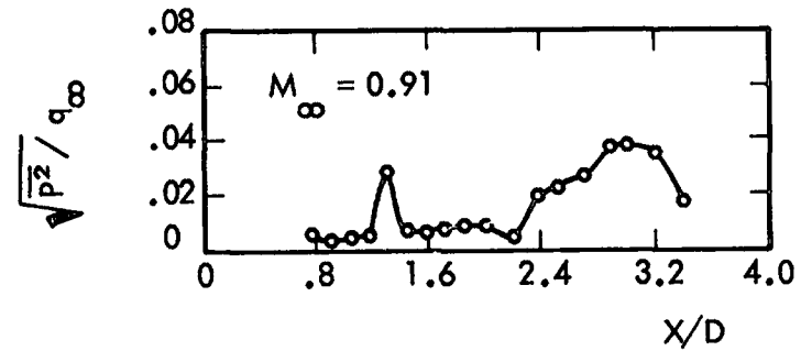
Figure 16. Axial Distributions of Fluctuating Pressures for Blunt Body Separated Flow; Ellipsoidal Nose Cone on a Cylindrical Body with a 30 Degree Step (Reference 43)
