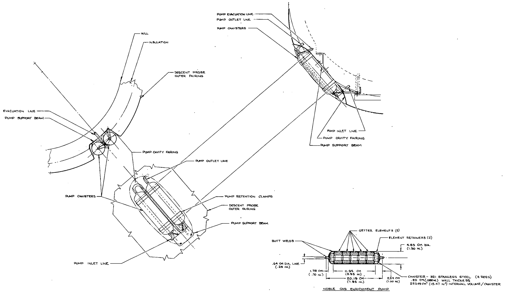
Figure 7.2 Noble Gas Experiment Pump Design
