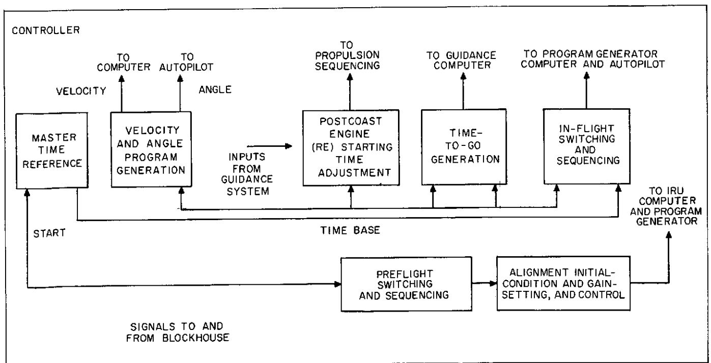
Fig. 15. Functional Block Diagram of Controller
