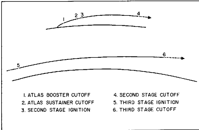
Fig. 9. Powered Flight Trajectory for Interplanetary Mission
