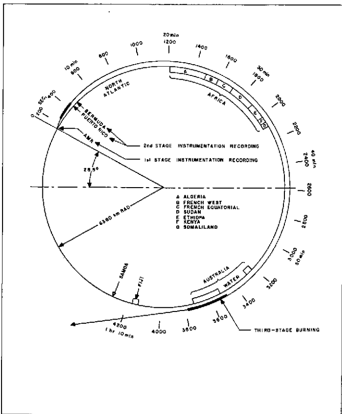
Fig. 20. Approximate Northeast Mars Trajectory Showing Typical Preinjection Flight Events
