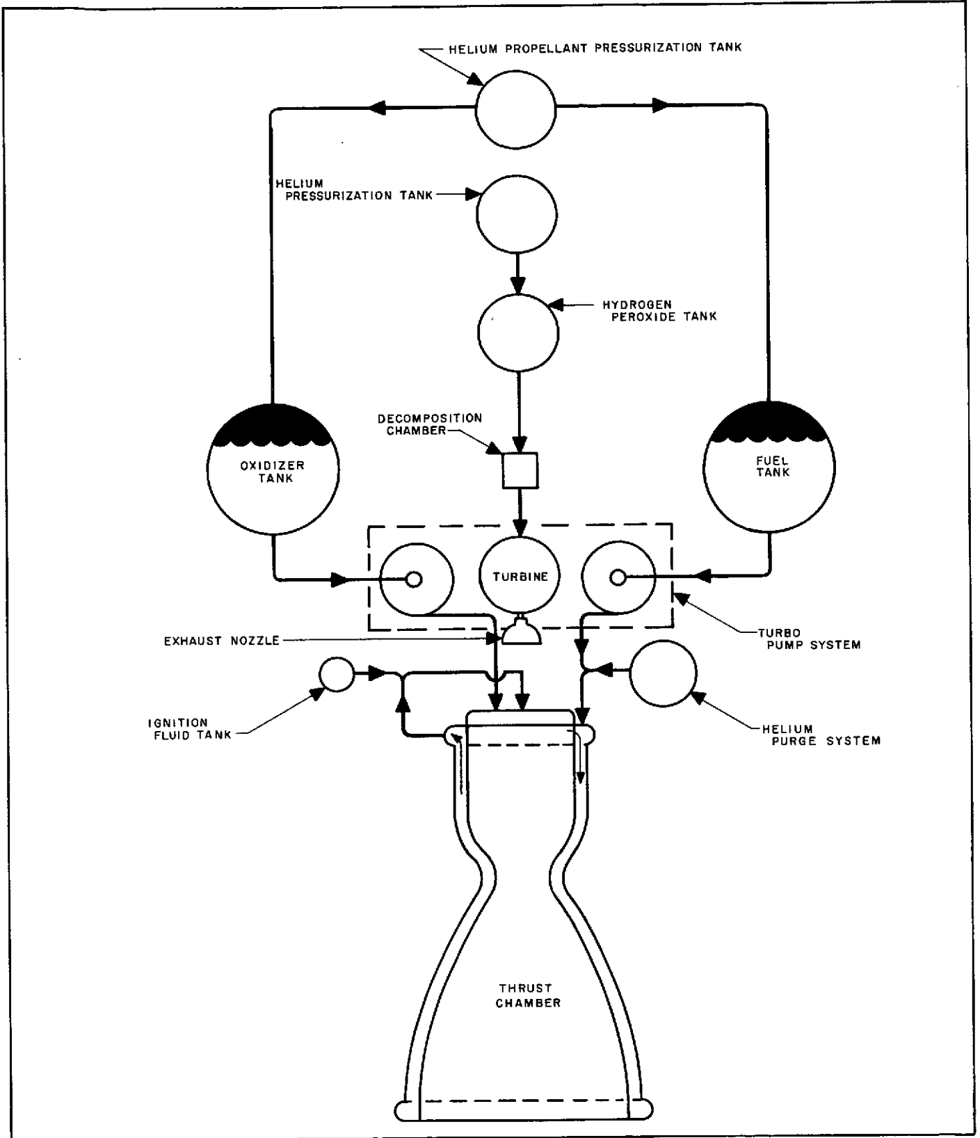
Fig. 11. Vega Second-Stage Propulsion System Employing GE 405H-2 Rocket Engine
