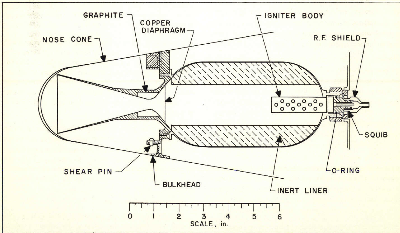
Fig. A-2. Small Solid Kick Rocket Employed on Explorer VI
