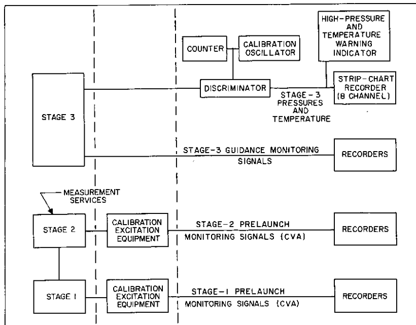
Fig. 28. Ground Monitoring System
