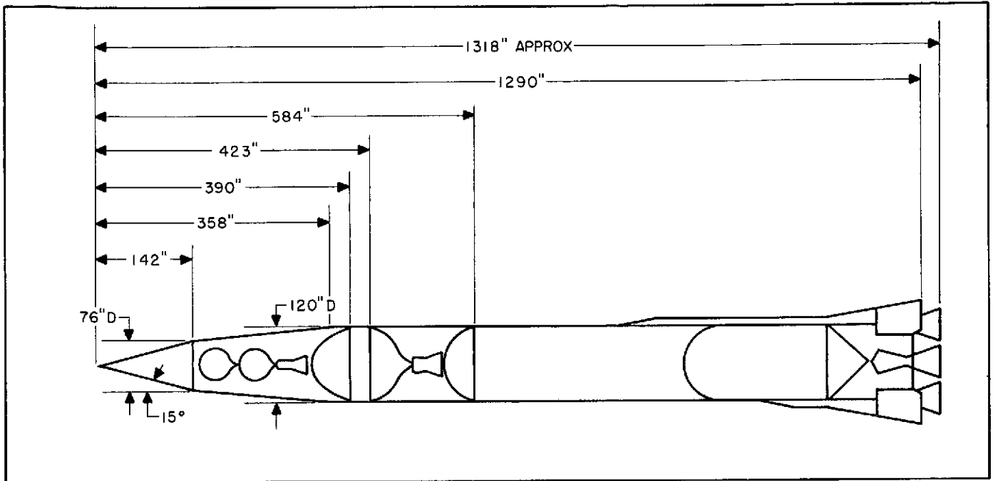
Fig. 8. Vega Vehicle Design Dimensions
