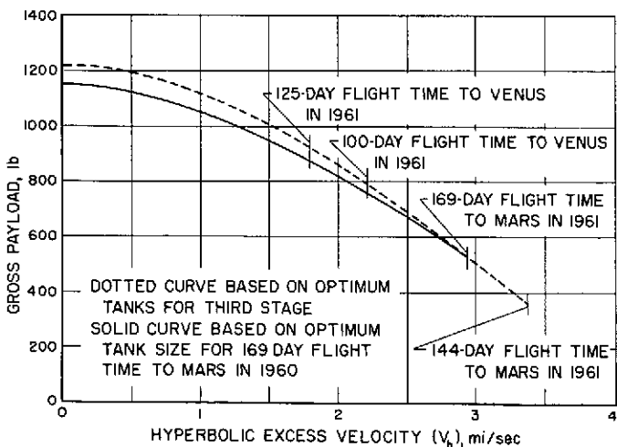
Fig. 3. Gross Payload Weight for a Three-Stage Vehicle as a Function of Hyperbolic Excess Speed
