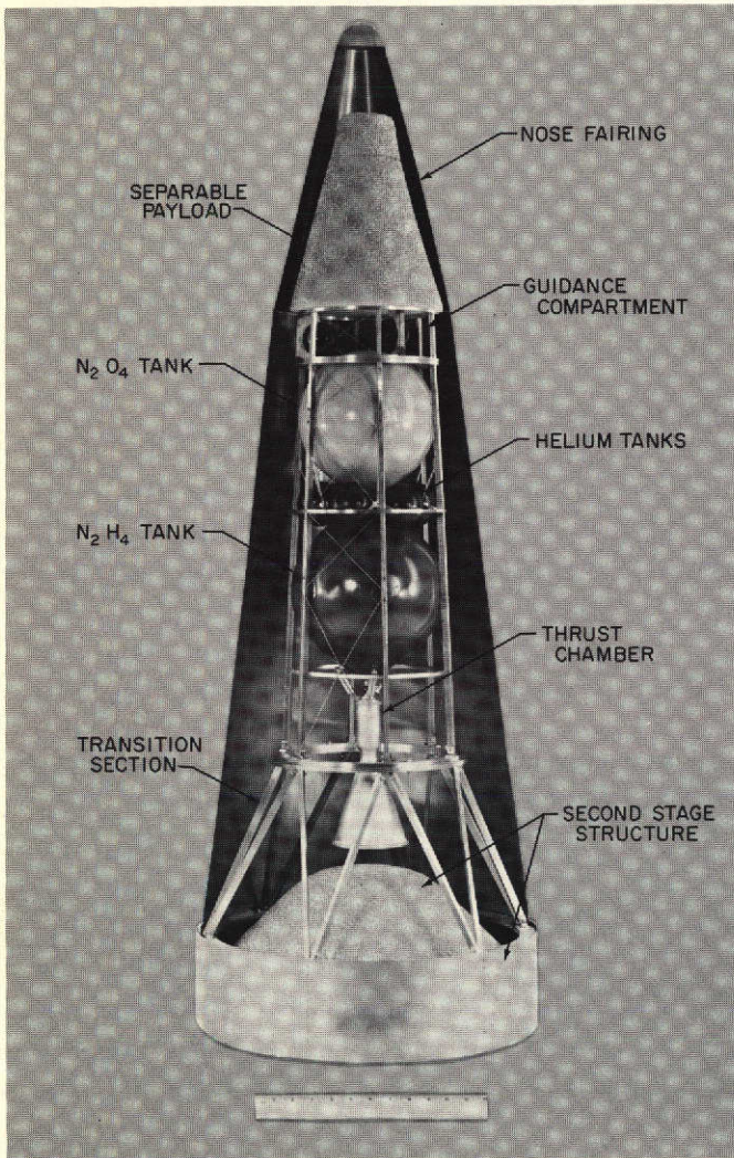
Fig. 7. Third-Stage and Payload Installation Showing Disposable Nose Fairing
