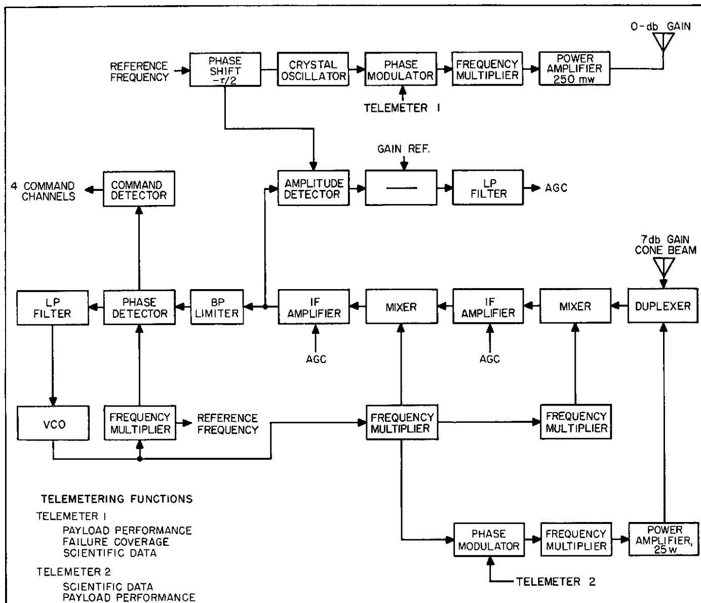
Fig. A-3. Payload Communication System
