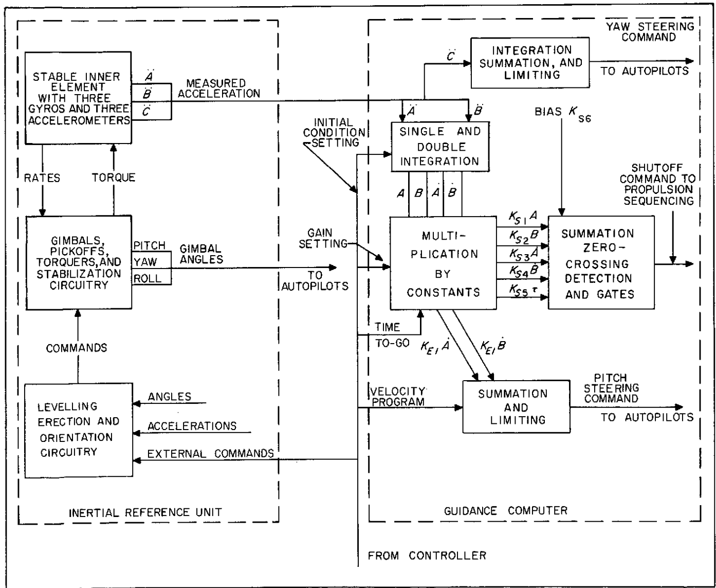
Fig. 13. Block Diagram of Vega Injection Guidance System
