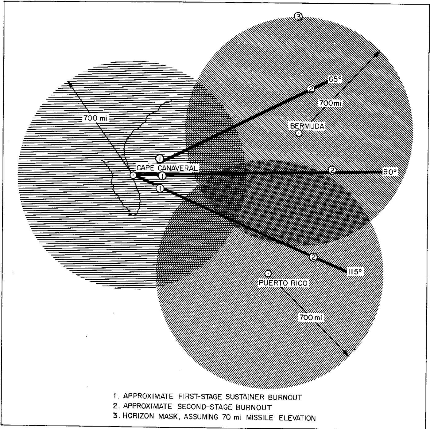
Fig. 18. Down-Range Radio Horizons
