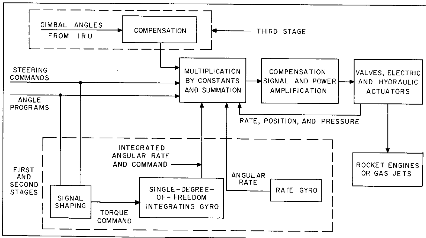
Fig. 14. Block Diagram of Autopilot
