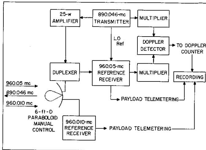
Fig. 21. Launch Instrumentation Station
