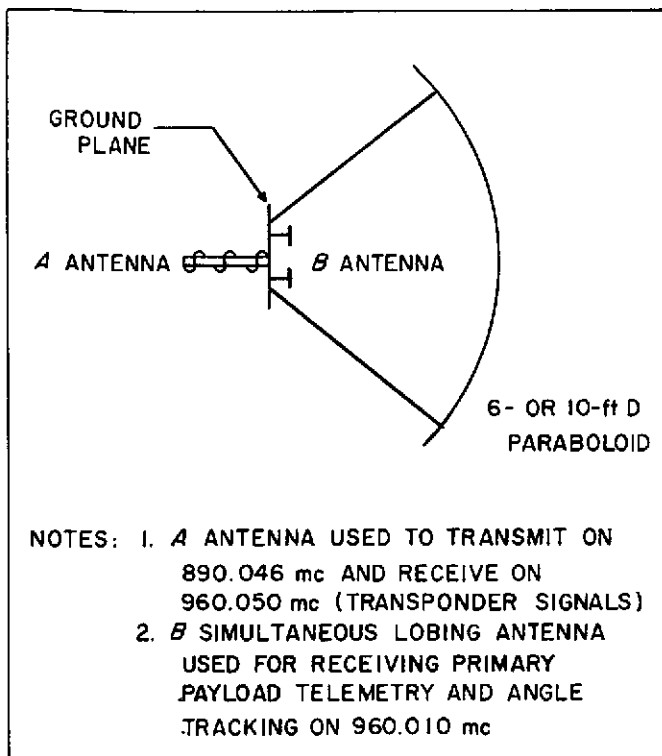
Fig. 22. Antenna Elements of Payload Telemetry and Tracking Ground Station
