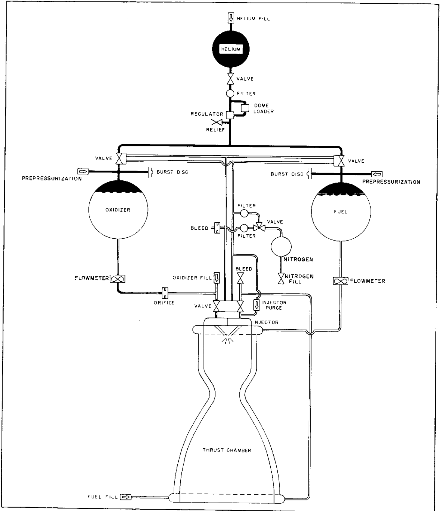
Fig. 12. Vega Third-Stage Propulsion System
