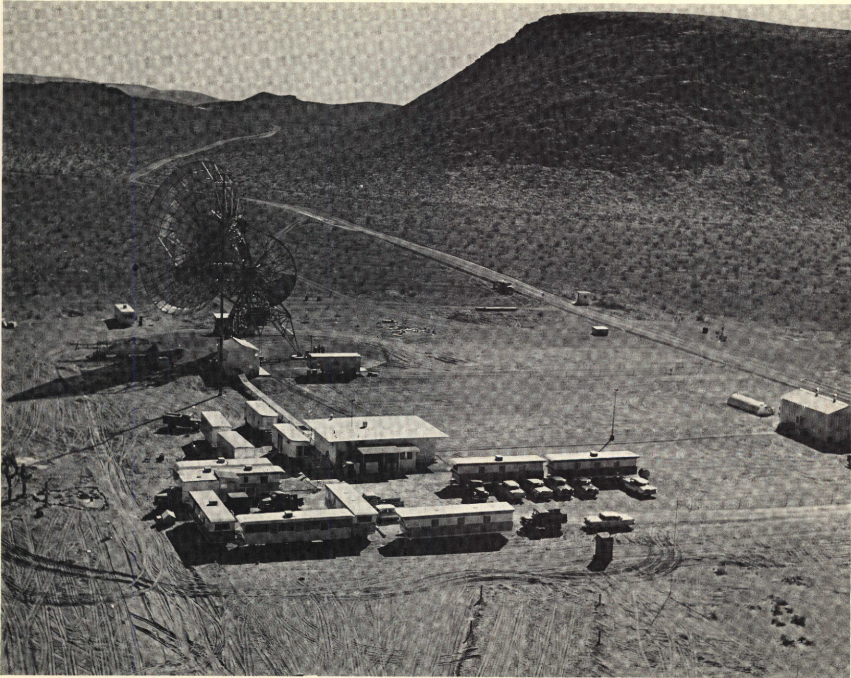
Fig. 25. Goldstone Station as Employed in Tracking Juno II to 407,000 Miles on March 6, 1959
