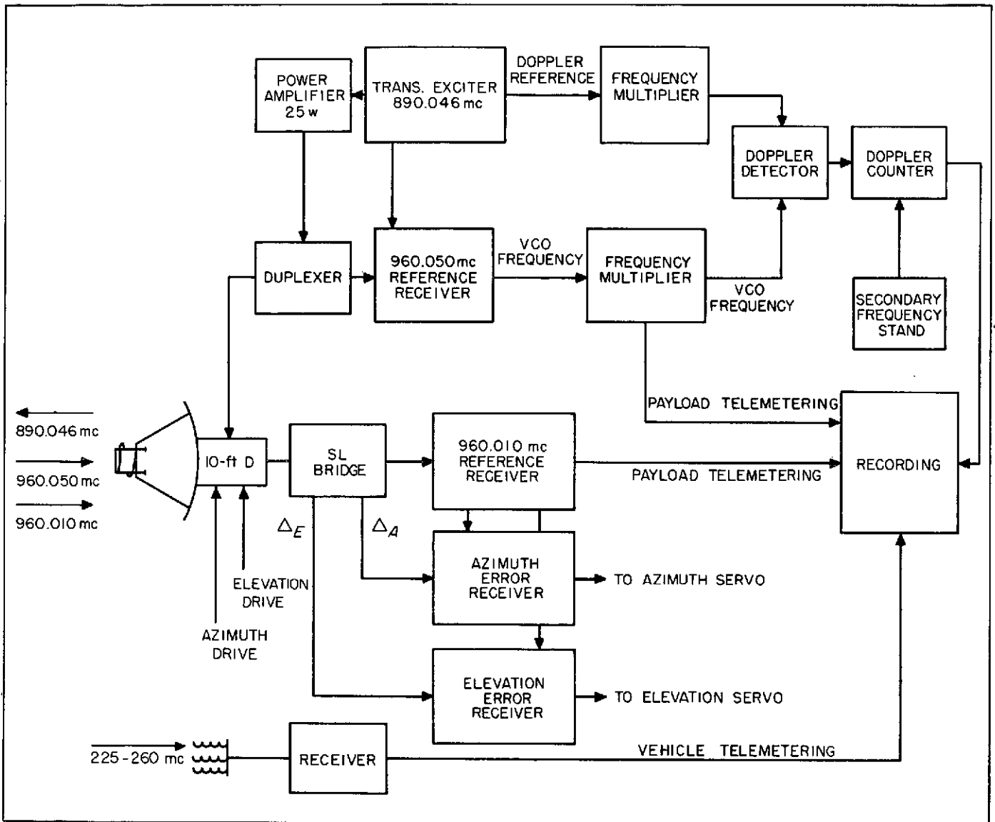
Fig. 23. JPL Down-Range Instrumentation Station
