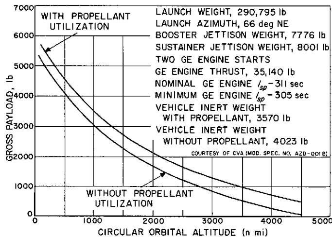
Fig. 4. Gross Payload Weight for a Two-Stage Earth Satellite Vehicle
