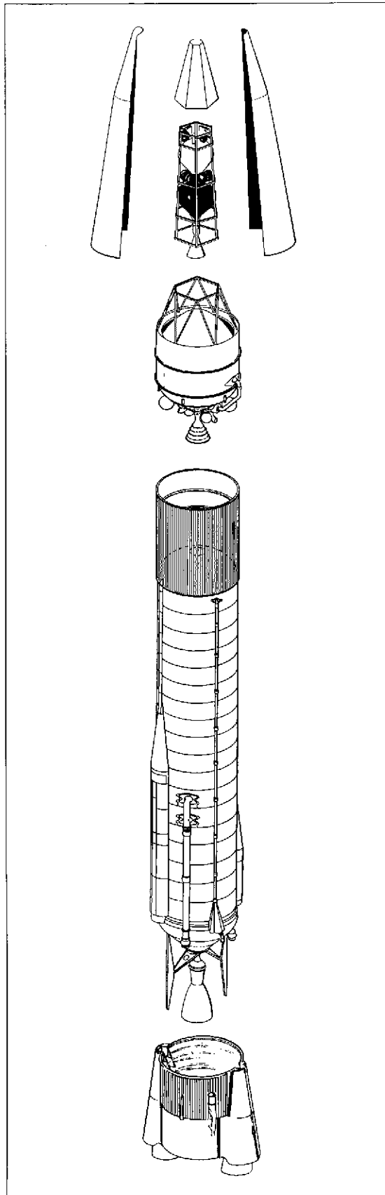
Fig. 6. Vega In-Flight Separations
