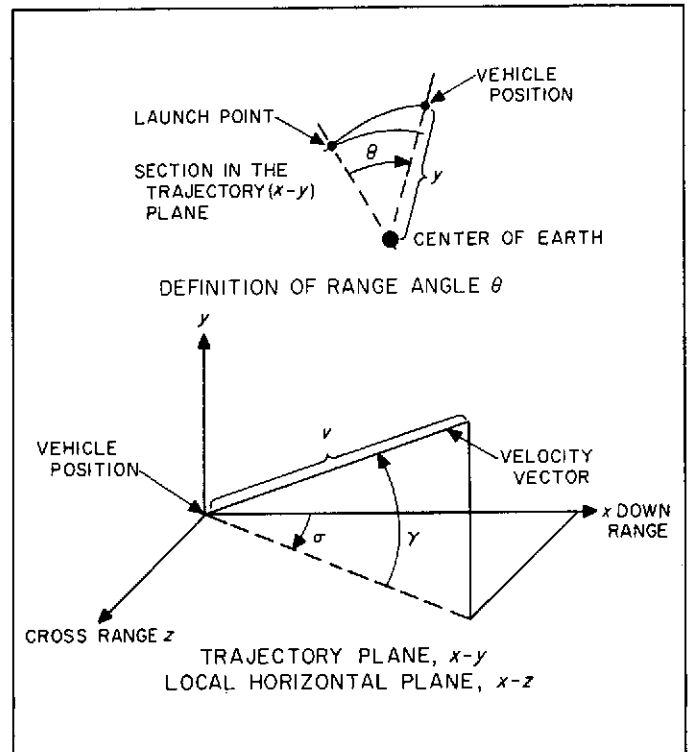
Fig. 5. Definition of Injection Coordinates
