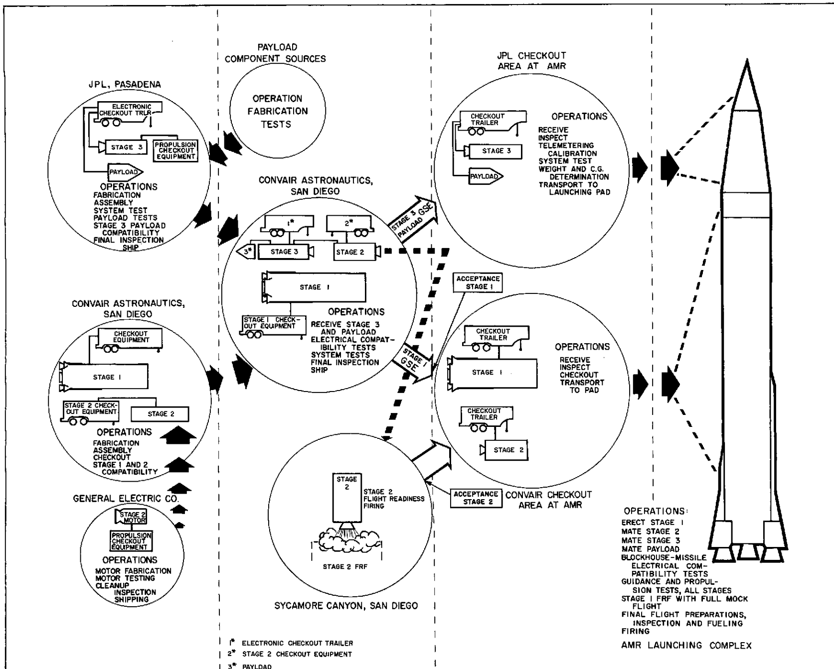
Fig. 26. Major Operations in Support of Vega Vehicle
