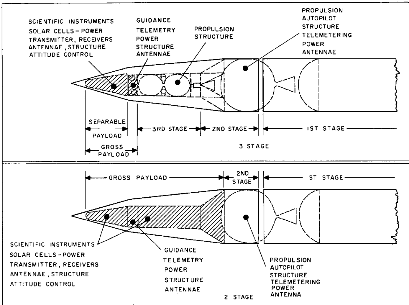
Fig. 2. Gross Payload Definition
