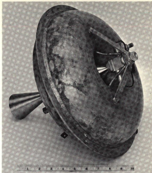
Fig. A-1. Small N_2H_4 Rocket Developed for Payload Use on Juno II
