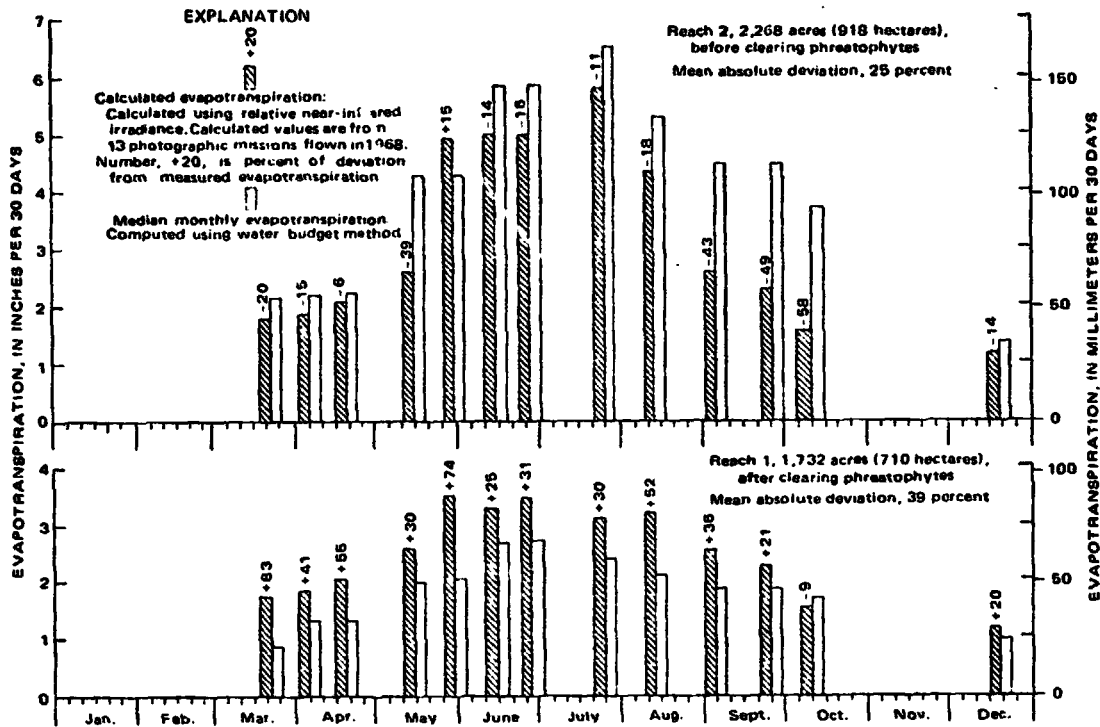
FIGURE 9.—Remote sensing and water-budget values of evapotranspiration versus time, Gila River Phreatophyte Project area.
