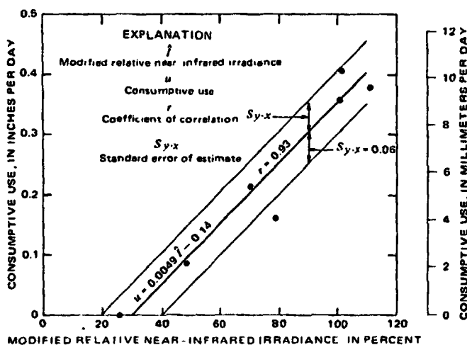
FIGURE 14.—Regression relation between consumptive use of water and modified relative near-infrared irradiance for grain sorghum during the 1969 growing season
