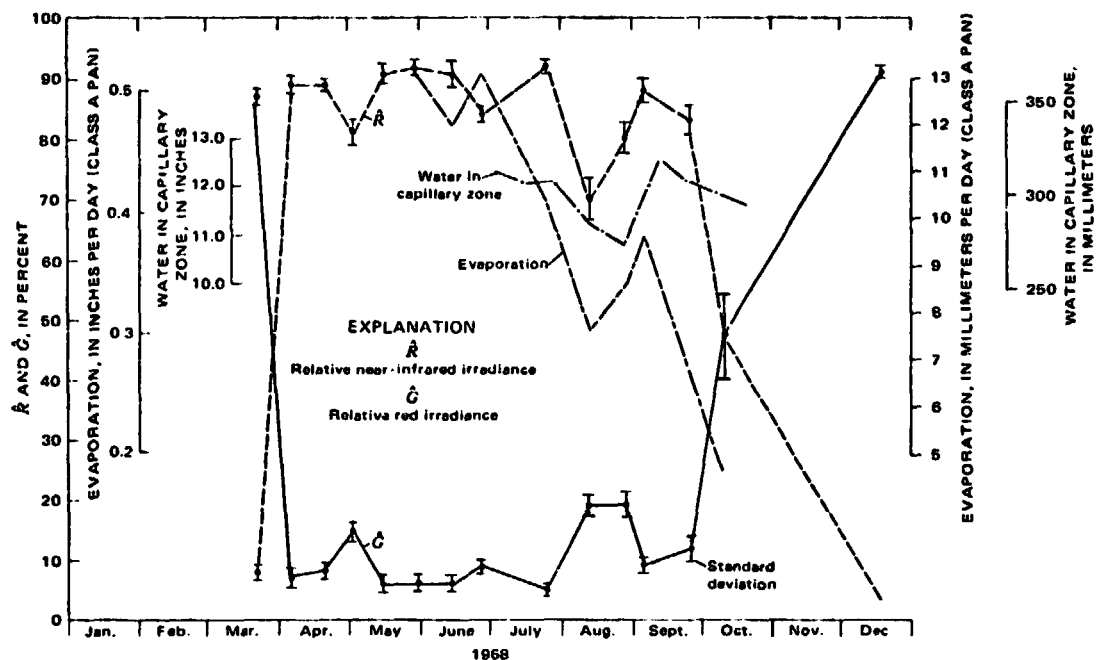
FIGURE 16.—Relative near-infrared irradiance, relative red irradiance, evaporation, and water in the capillary zone for a dense 40-acre (16-ha) saltcedar site, 1968
