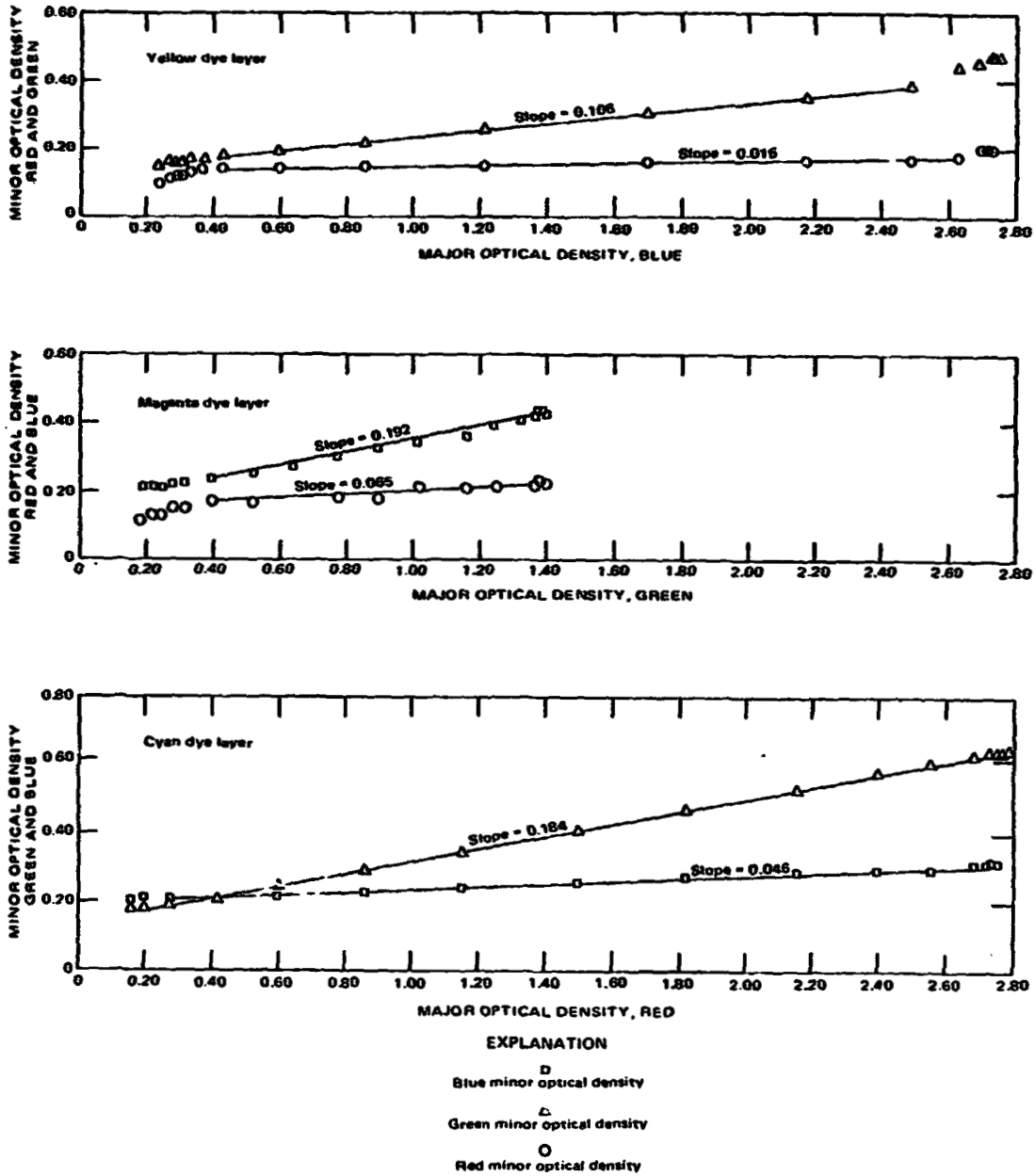
FIGURE 31.—Major versus minor optical densities for the three dye layers of film type 8443.
