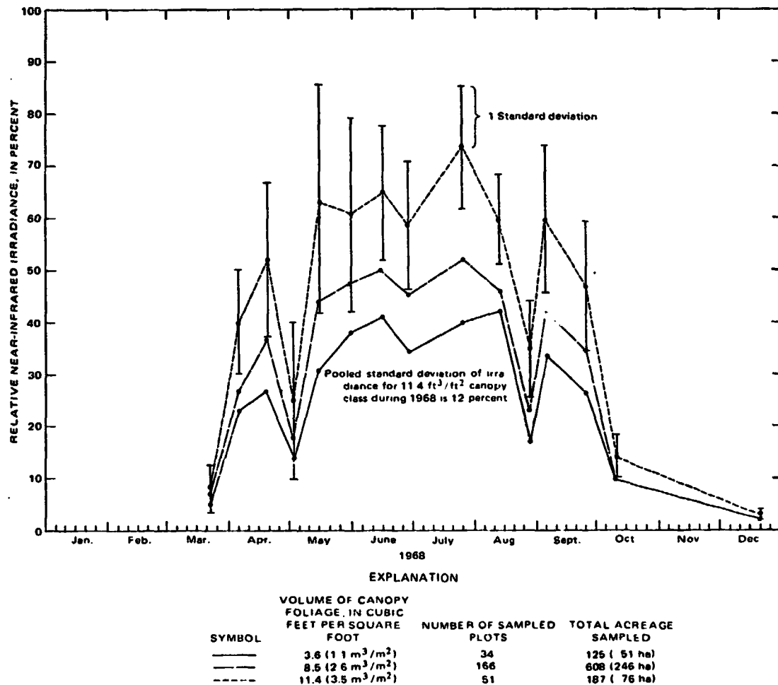
FIGURE 27.—Relative near-infrared irradiance versus time for three saltcedar volumes of canopy foliage classes, reach 2, Gila River Phreatophyte Project.
