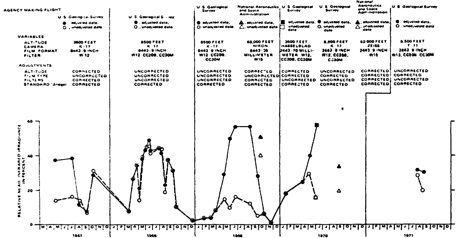
FIGURE 30 —Adjusted and unadjusted relative near-infrared irradiance, subreach 2b of the Gila River Phreatophyte Project, 1967-71.
