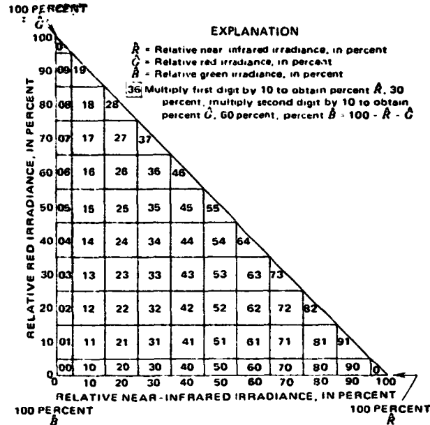
FIGURE 24 —Computer printout codes used in spatial analysis of relative near-infrared, relative red, and relative green irradiance.
