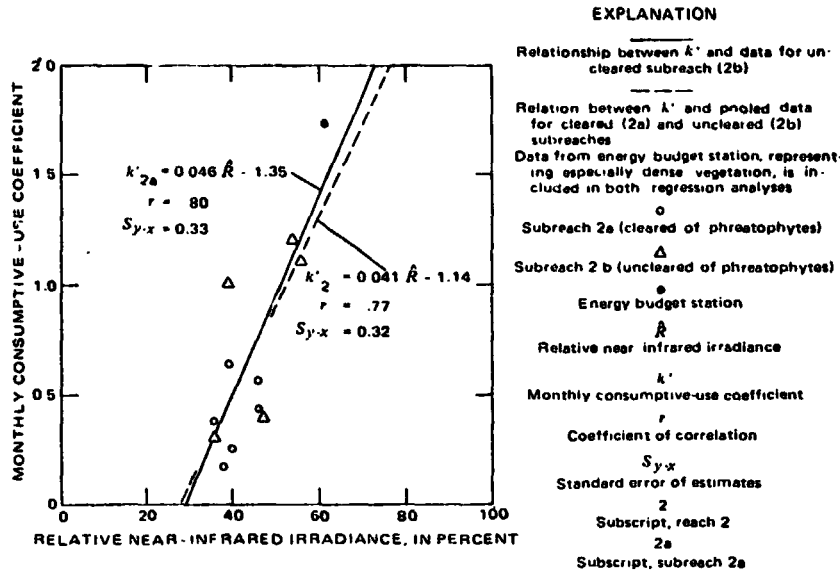
FIGURE 12.—Monthly consumptive-use coefficient versus relative near-infrared irradiance.
