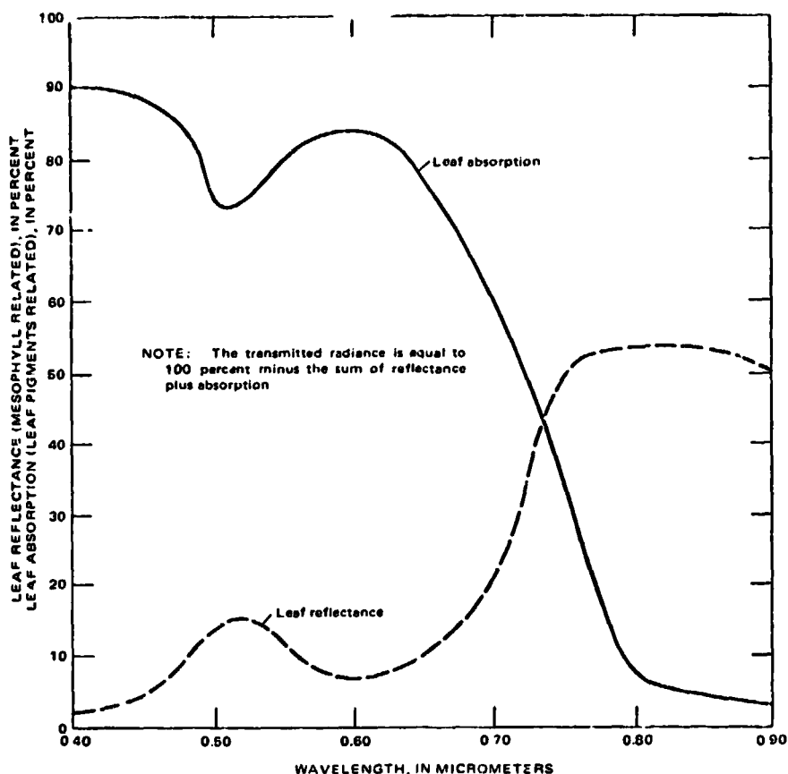
FIGURE 5.—Average leaf reflectance and absorption as a function of wavelength.
