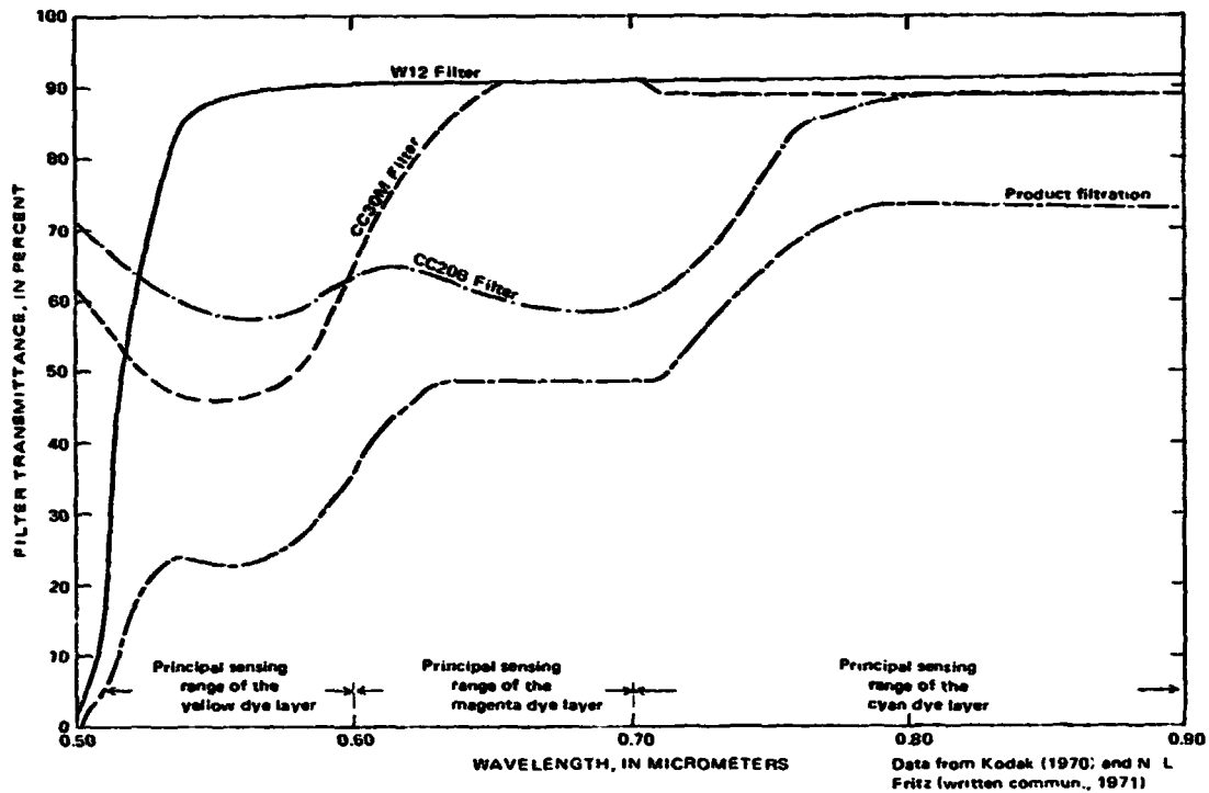
FIGURE 32.—Filter transmittance versus wavelength for the standard filter pack used in aerial photography in the study areas.
