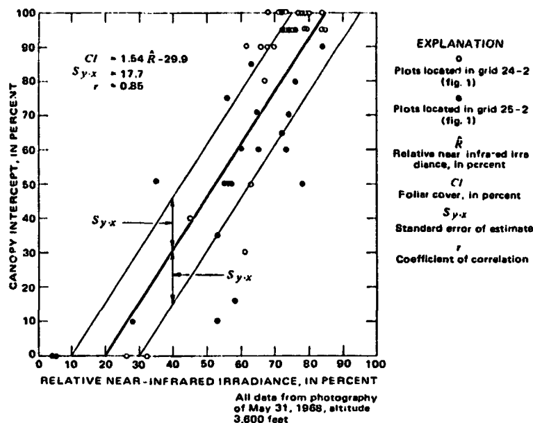
FIG. 9.—Foliar cover versus relative near-infrared irradiance for 50 3.67-acre (1.49-ha) plots, subreach 2b, Gila River Phreatophyte Project.
