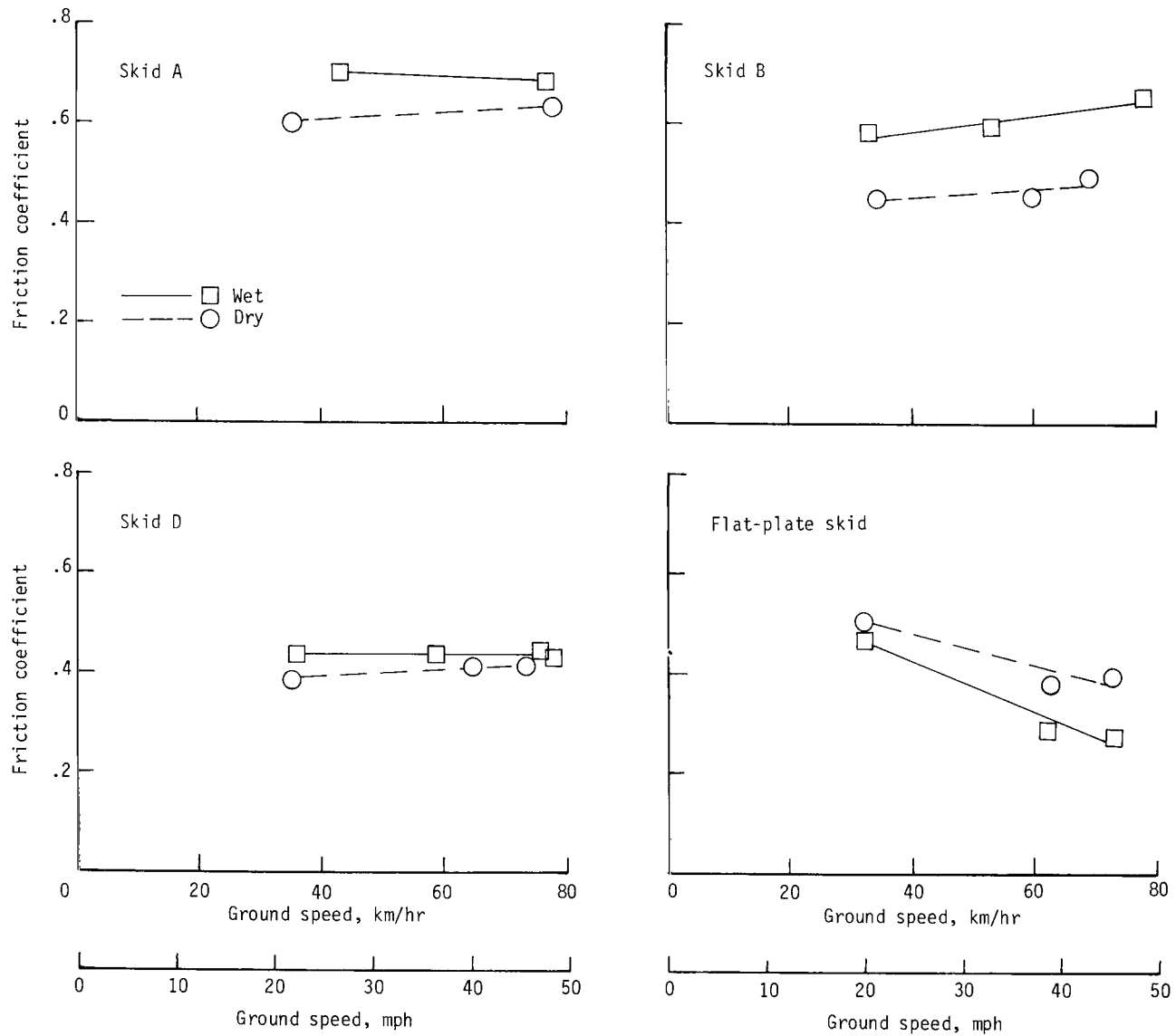
Figure 7.- Effect of surface wetness on friction coefficient developed by skids on the asphalt surface. Bearing pressure, 689 kPa (100 psi).
