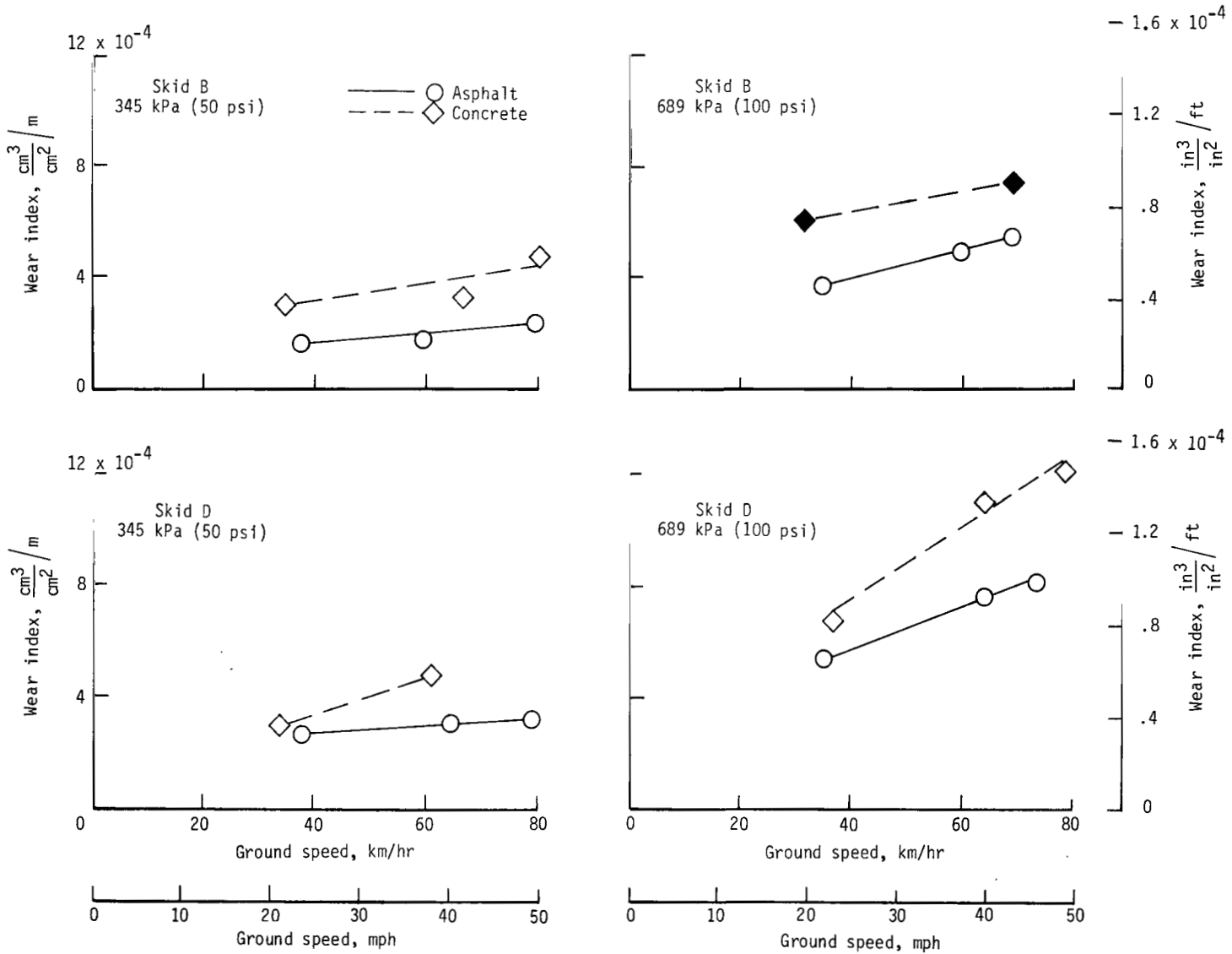
25 Figure 11.- Effect of runway surface on skid wear. Closed symbols denote wire loss due to fatigue.
