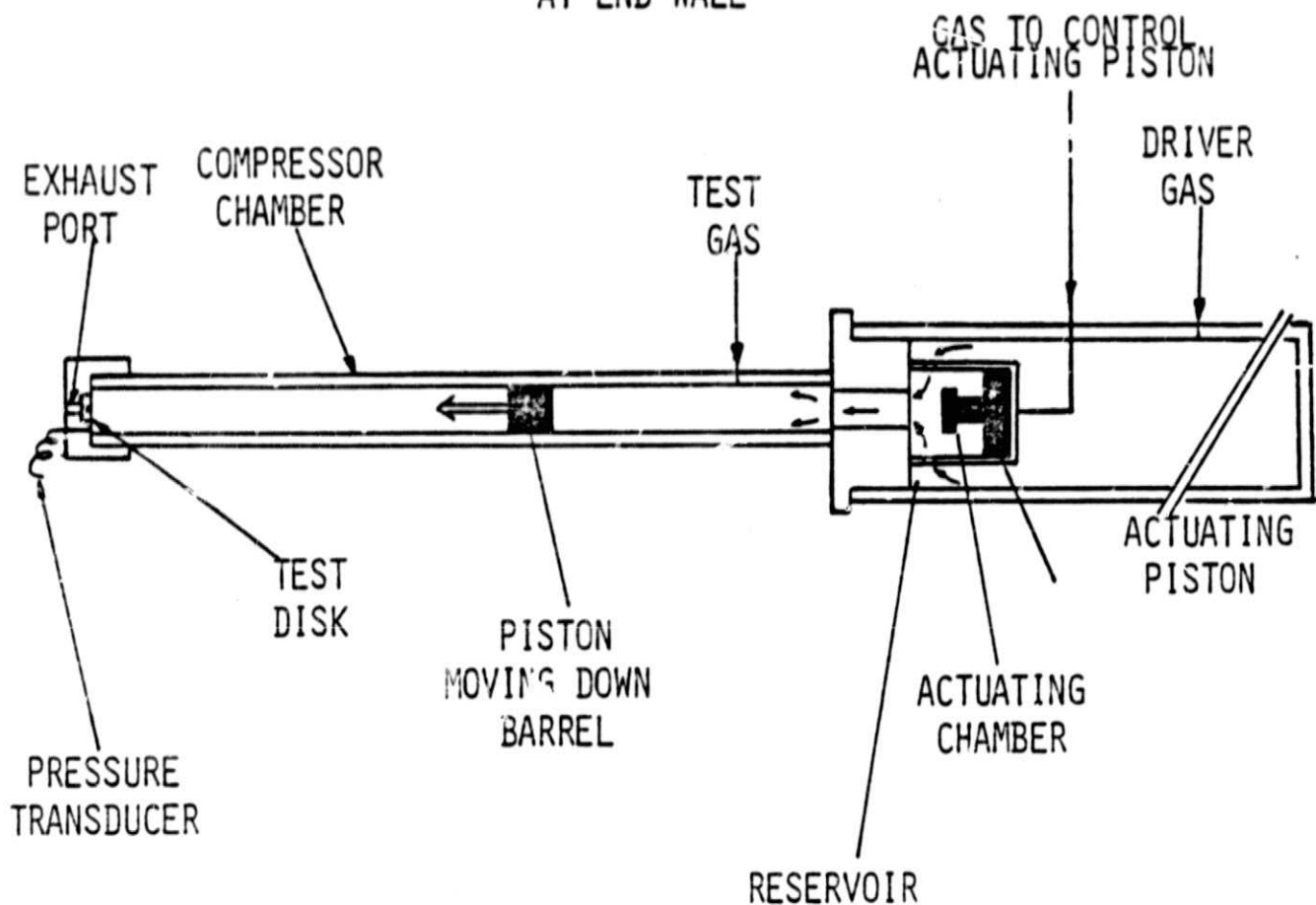
Fig. 1 Schematic diagram of the ballistic compressor showing test disk at end wall.
