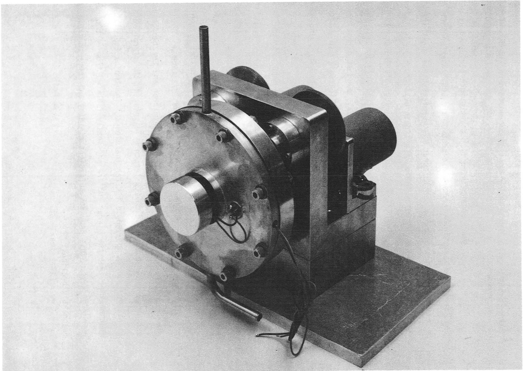
Figure 42. Photograph of Cavity Length Tuner
