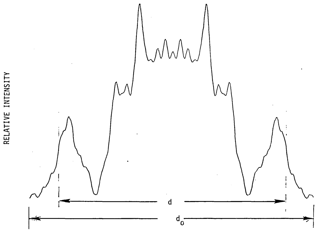
Figure 4. Near Field Intensity Distribution of Passive Cavity in the Plane of Mirror 1 When Scraper Mirror is Removed ( d = hole diameter of scraper mirror, d_0 = beam diameter at mirror 2).
