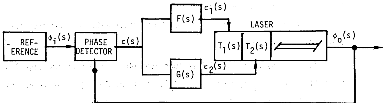
Figure 48. Closed-Loop System
