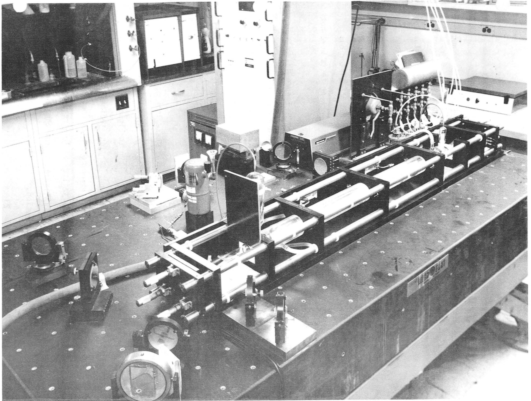
Figure 13. Unstable Resonator for Low Pressure Phase Lock Tests
