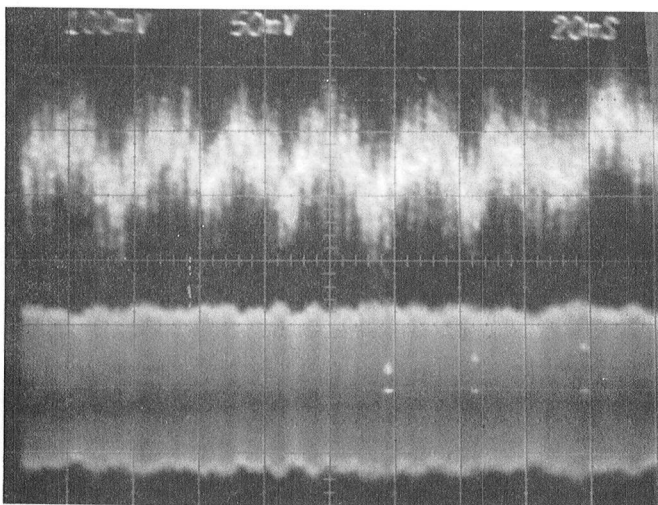
Figure 40. Oscilloscope traces of Fast Power Monitor (Upper) and Beat Signal (Lower), Run #1, 3/29/77
