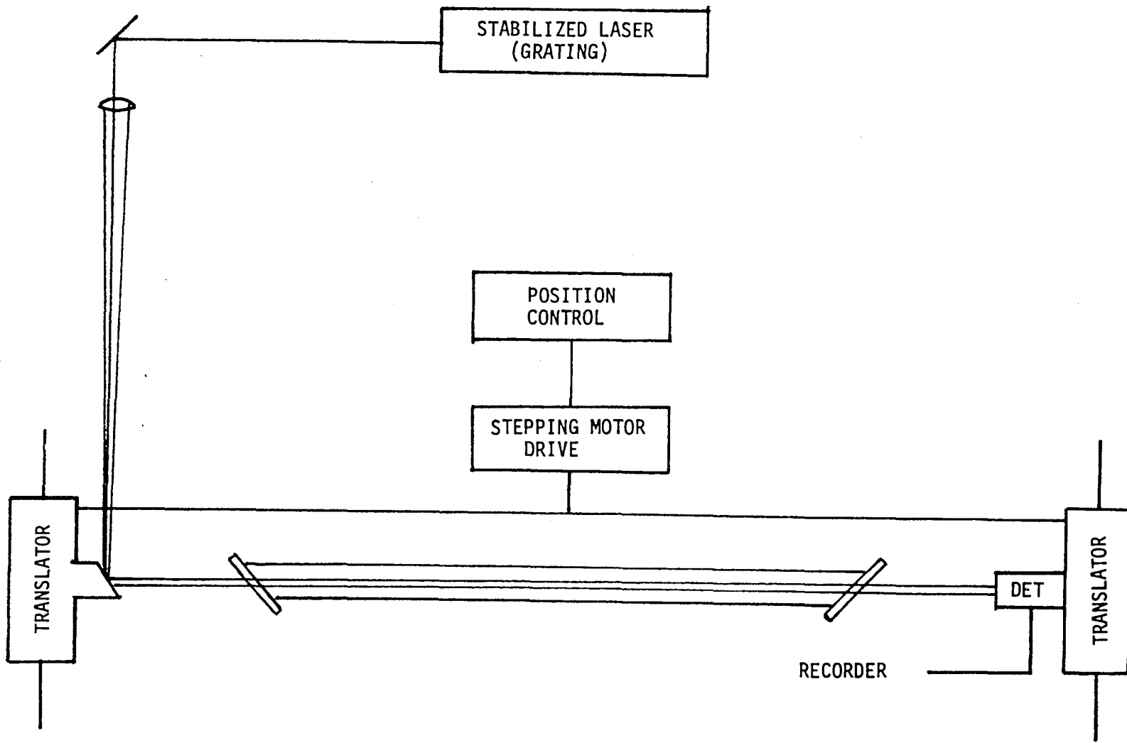
Figure 16. Apparatus for Measuring Radial Gain Profile
