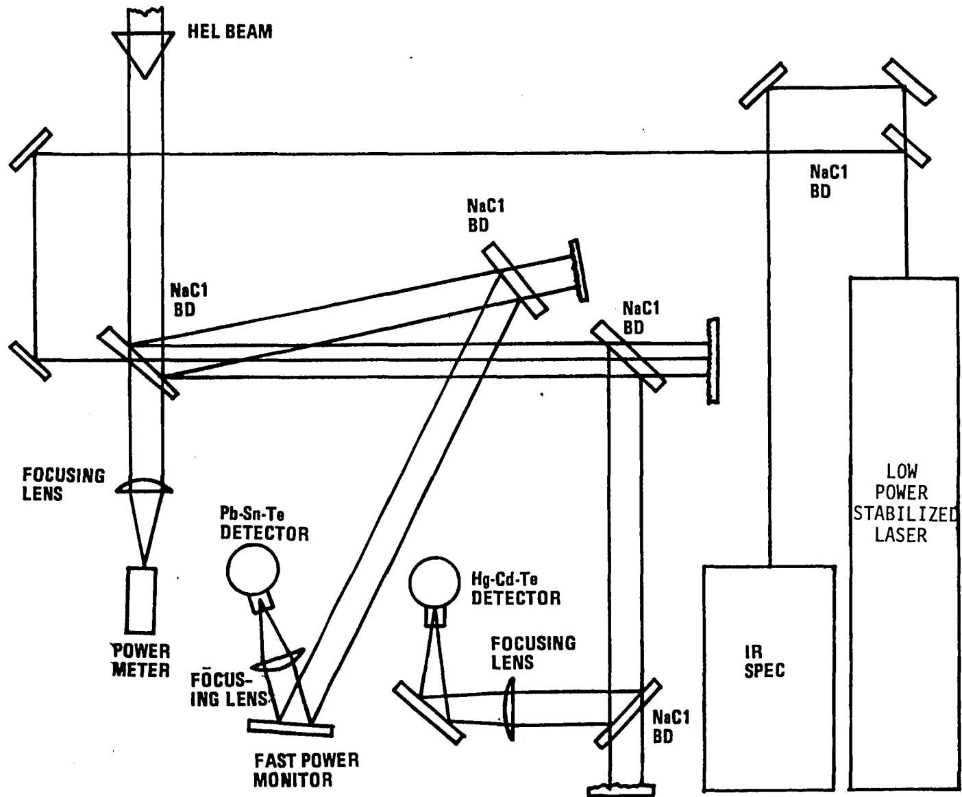
Figure 34. Test Room Optical Schematic (Tests 3/28/77 - 3/30/77)
