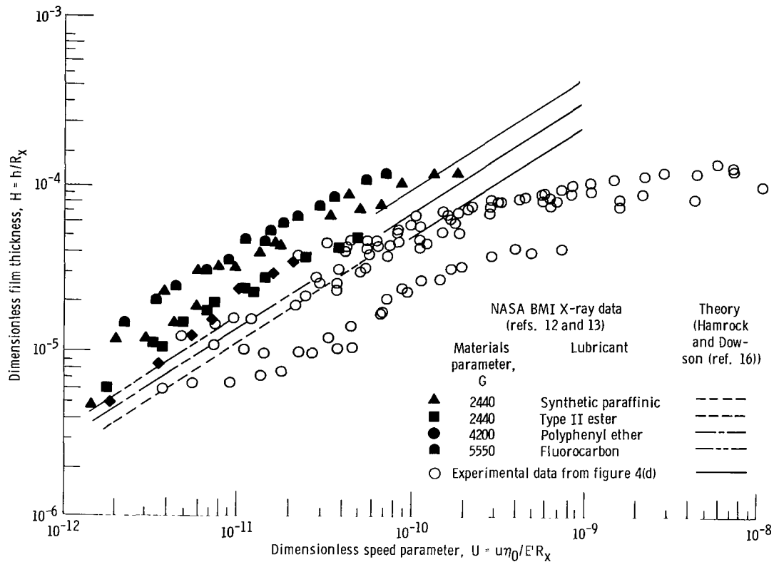
Figure 6. - Comparison with X-ray film thickness measurements.
