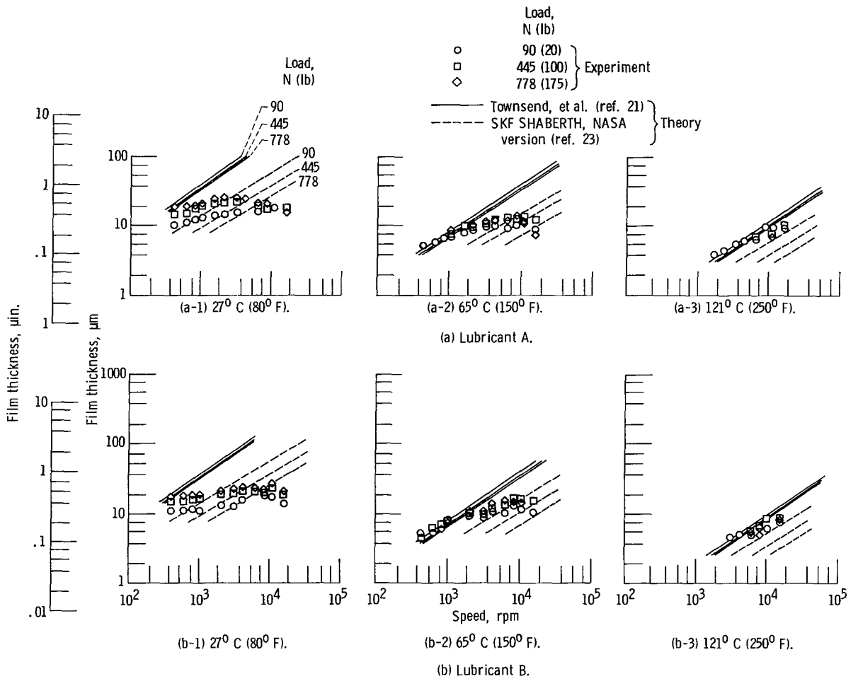
Figure 3. - Measured film thickness as a function of load, speed, and temperature for four lubricants.
