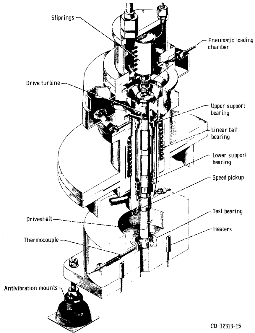
Figure 1. - EHD film thickness measurement rig.
