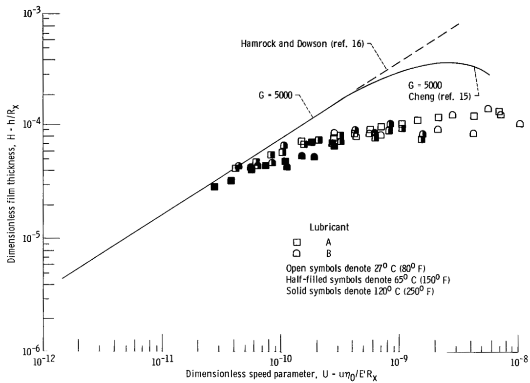
Figure 8. - Effect of inlet shear heating on film thickness and comparison with experiment.
