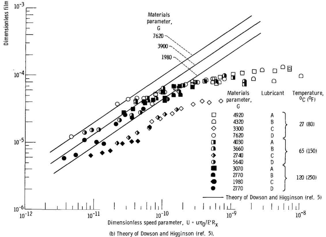
Figure 4. - Comparison of isothermal, fully flooded inlet theory with measurements for 90-newton (20-lb) load.
