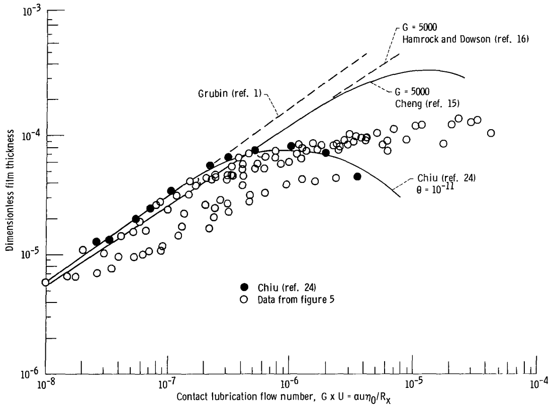
Figure 9. - Effect of kinematic starvation on film thickness and comparison with theory.
