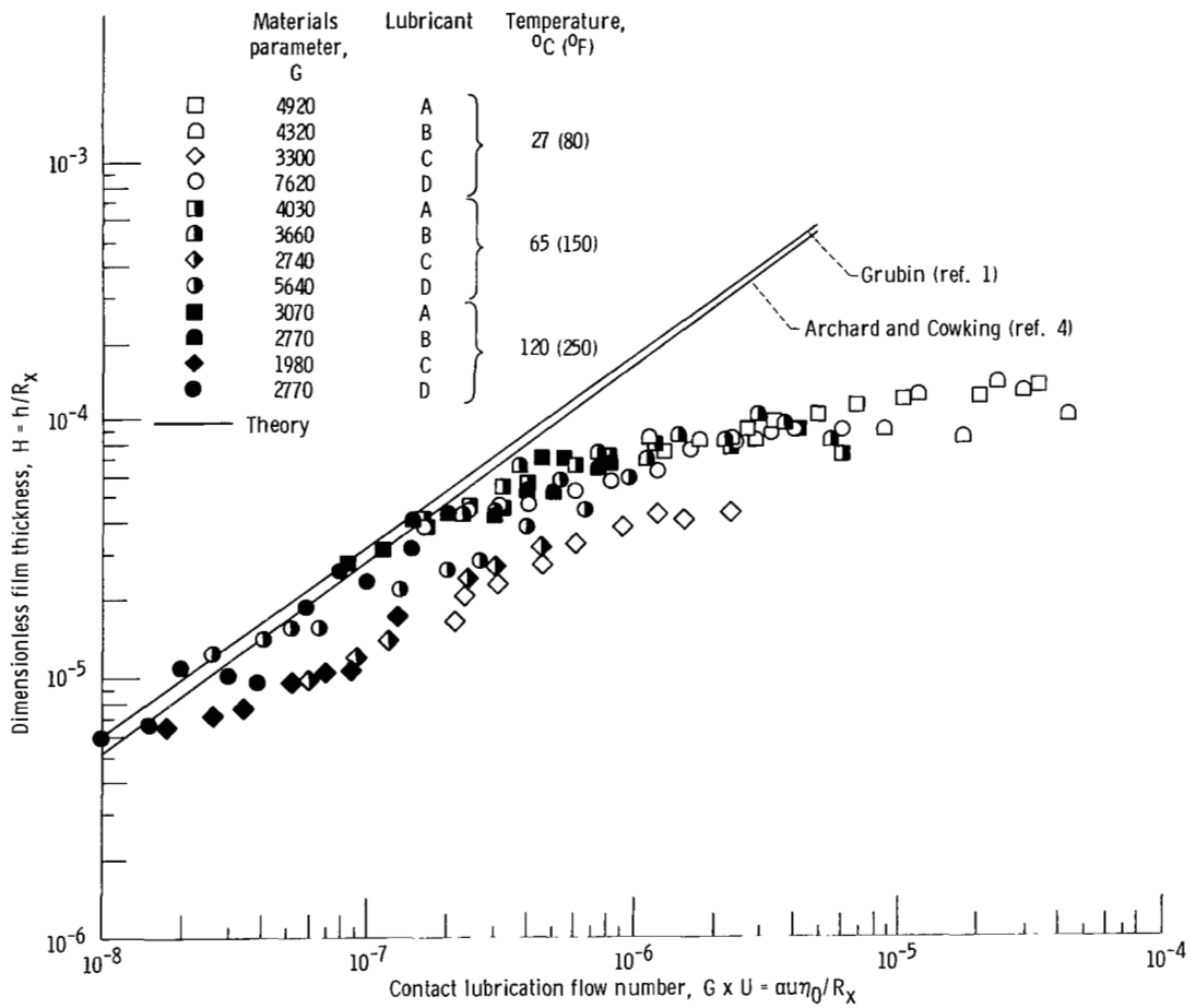
Figure 5. - Comparison of theory with experiment for 90-newton (20-lb) load.
