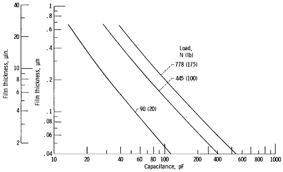
Figure 2. - Calculated capacitance for test bearing as a function of load and film thickness.
