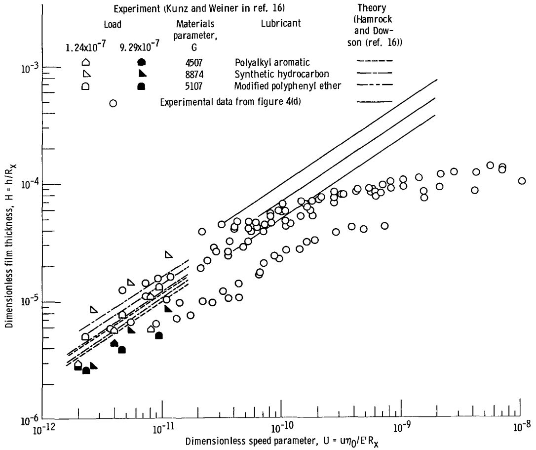
Figure 7. - Comparison with optical film thickness measurements under pure sliding.
