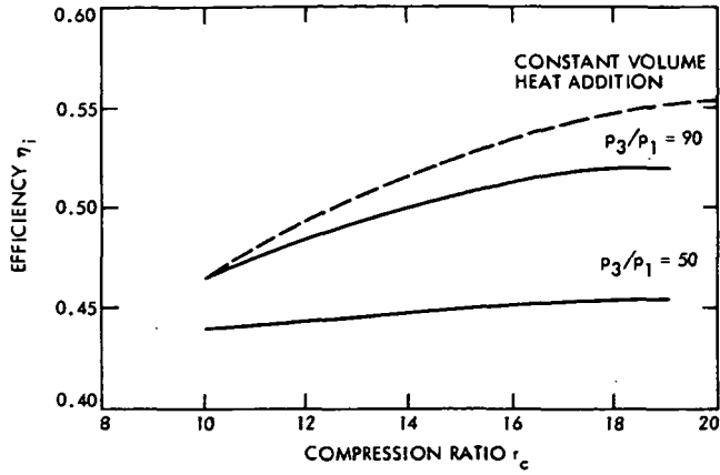
Fig. 4-23. Efficiency of limited-pressure, ideal fuel/air cycles with \phi = 0.9 and ambient temperature = 520^\circ\text{R}
