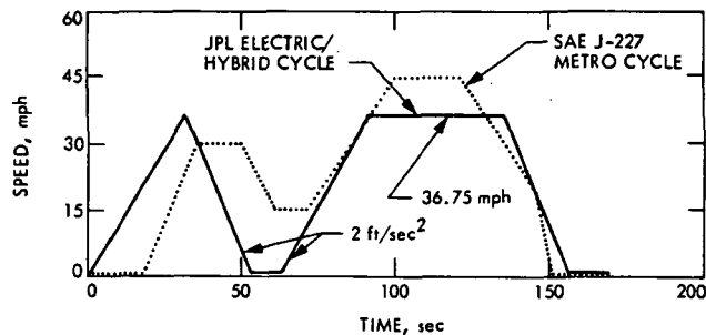
Fig. 8-3. Speed-time profile
