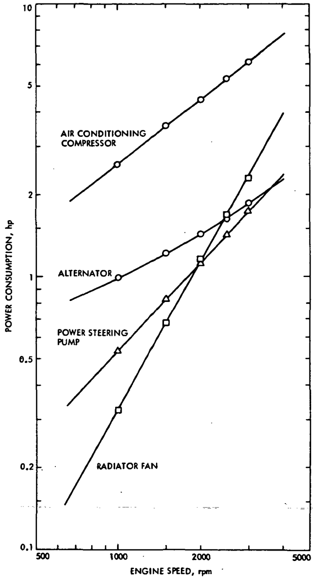
Fig. 10-3. Accessory horsepower
