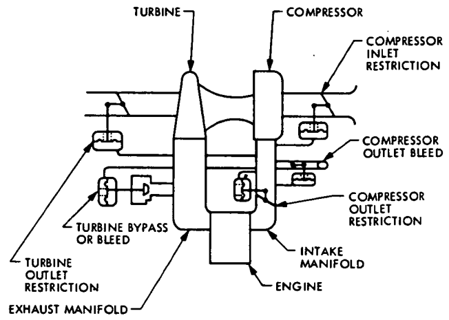
Fig. 4-31. Different methods of boost control (from Ref. 4-70)
