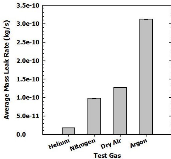
Figure 4. Average experimental leak rate of a silicone elastomer O-ring for four different gases, measured using a modified pressure decay method. Error bars represent measurement uncertainty.
