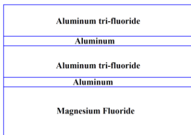
Figure 1. Metal dielectric Fabry-Perot type filter design using aluminum as the metal and aluminum tri-fluoride as the dielectric spacer layer deposited on a thin magnesium fluoride substrate.
