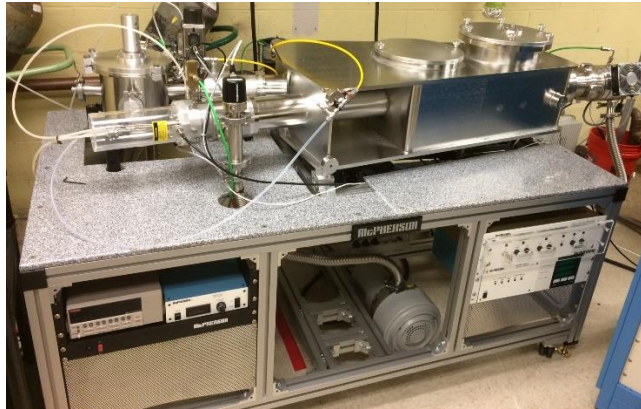
Figure 2. McPherson VUV reflectometer used for extreme ultraviolet and far ultraviolet (i.e. 58.4 nm to 200 nm) reflectance and transmittance measurements.
