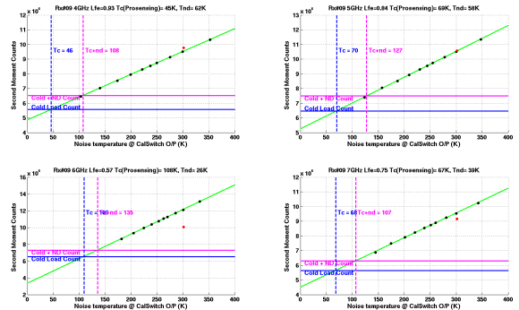
Figure 6: Final T_{CAL\_SWITCH} to C transfer function and estimated T_{ND} values for Receiver #09
