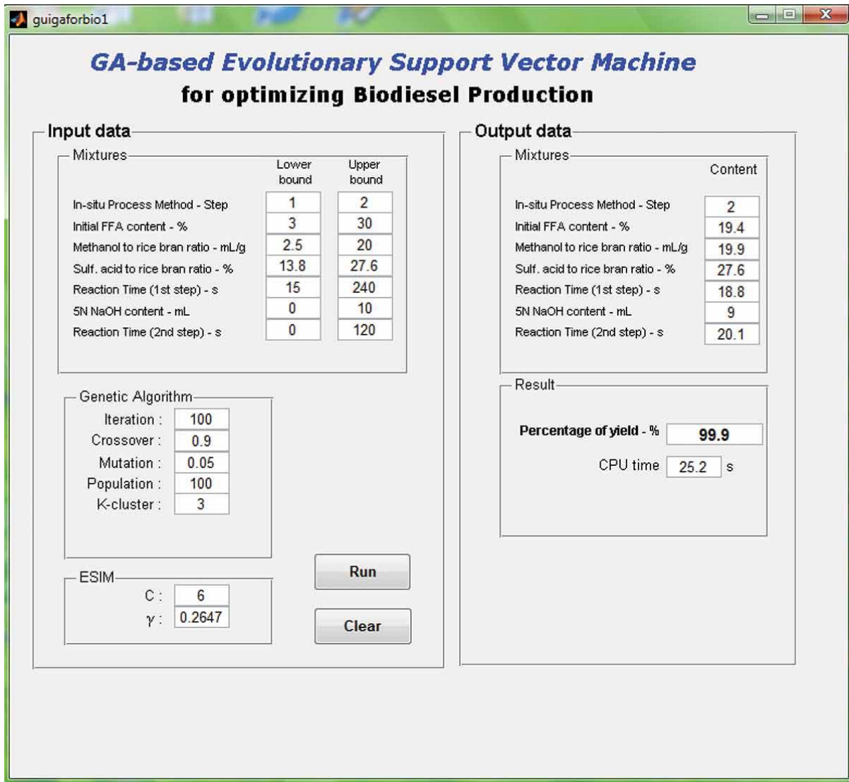
Fig. 4. Demonstration of Graphic User Interface (GUI) integrated with GA-ESIM
