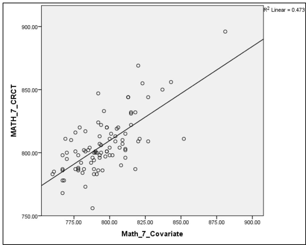
Figure 6. Scatterplot for seventh grade math scores vs. sixth grade math scores (covariate).
