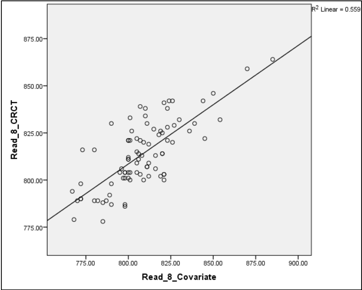
Figure 4. Scatterplot for eighth grade reading scores vs. seventh grade reading scores (covariate).
