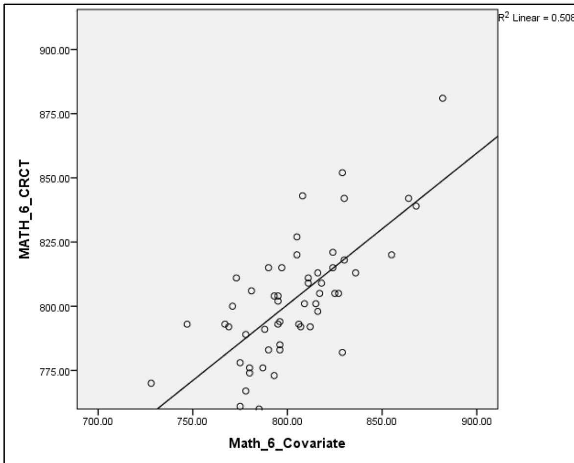
Figure 5. Scatterplot for sixth grade math scores vs. fifth grade math scores (covariate).
