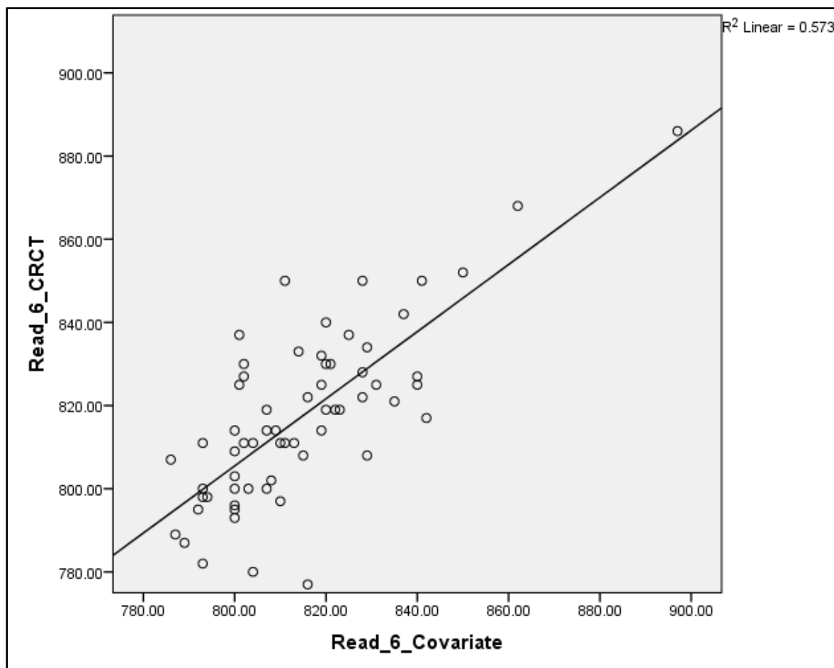
Figure 2. Scatterplot for sixth grade reading scores vs. fifth grade reading scores (covariate).
