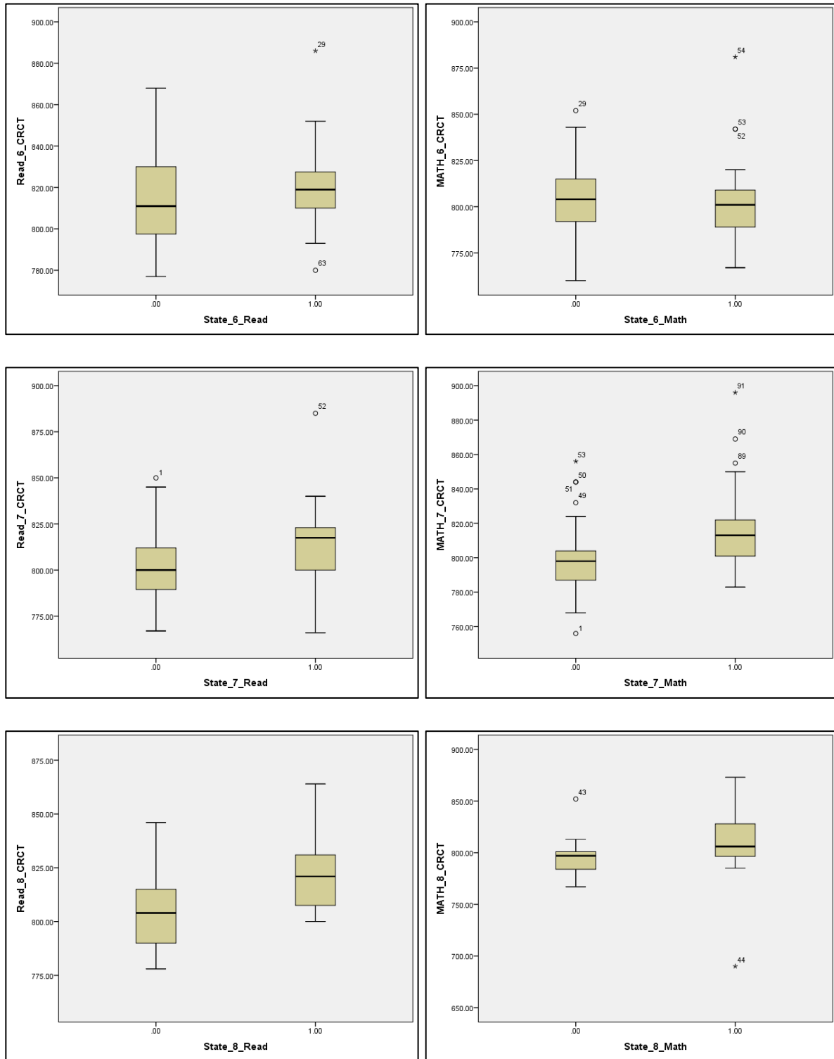
Figure 1. Boxplots for reading and math for grades 6–8.
