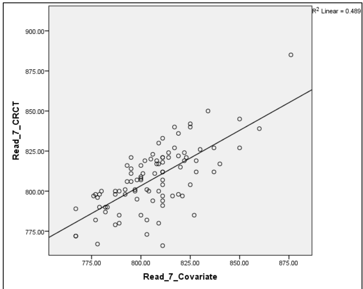
Figure 3. Scatterplot for seventh grade reading scores vs. sixth grade reading scores (covariate).
