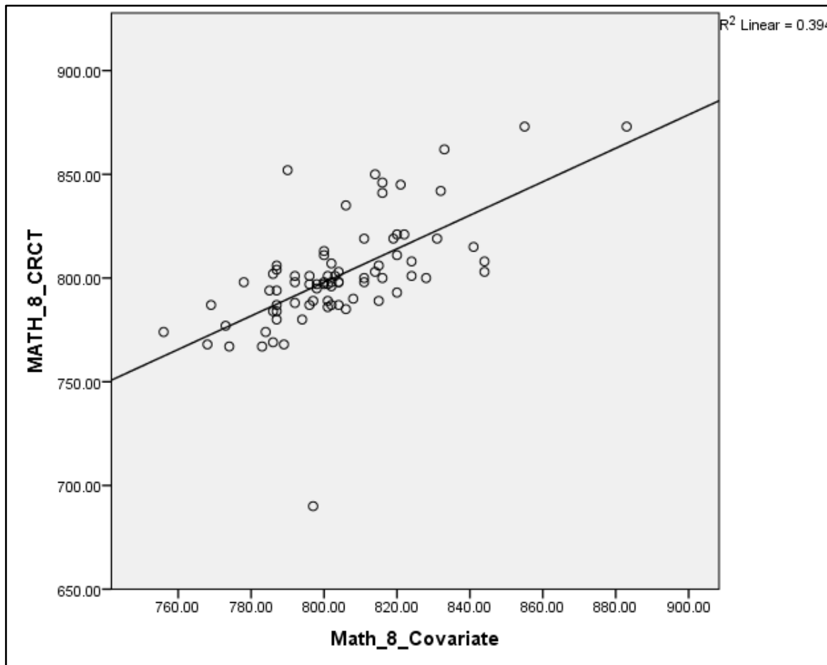
Figure 7. Scatterplot for eighth grade math scores vs. seventh grade math scores (covariate).
