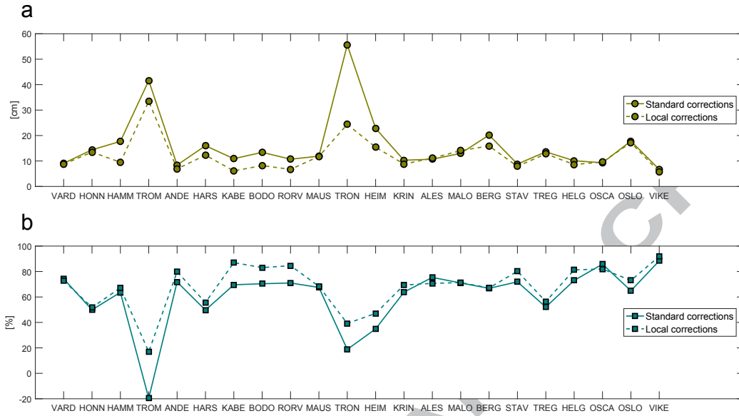
Figure 6: Comparison of CS2 with TGs using standard and local OT and IB corrections, in terms of (a) standard deviations of differences and (b) correlations. The TGs are ordered such that the northernmost TG appears first on the left-hand side of the horizontal axis, moving southward along the Norwegian coastline.
