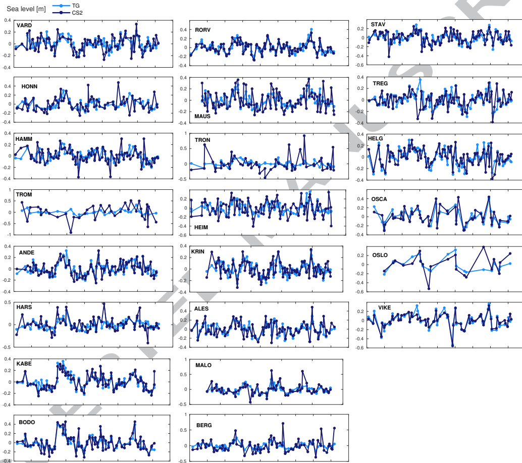
Figure 5: As Figure 4, but using local corrections.
