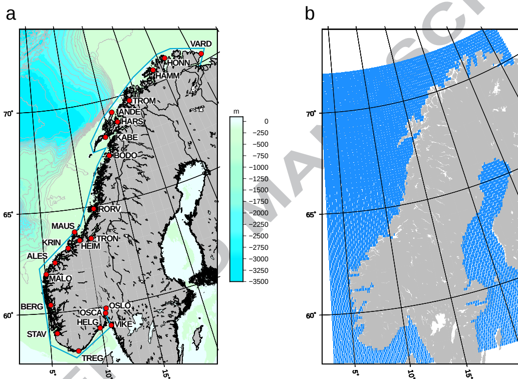
Figure 1: (a) The 22 Norwegian TGs considered in this study. The blue line shows the CS2 SARIn mode border, using the geographical mode mask version 3.8 (ESA, 2016). Bathymetry and 400 m isobaths are from the 2014 General Bathymetric Charts of the Oceans (GEBCO) (Weatherall et al., 2015). (b) FES2004 grid cells around Norway.
