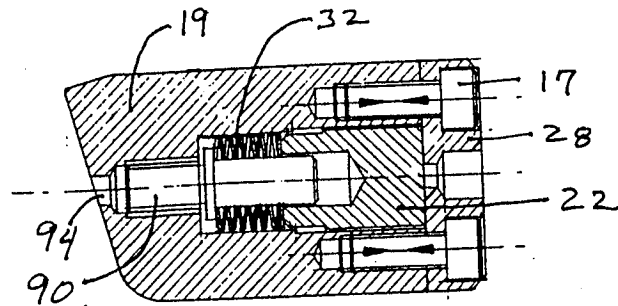
FIGURE 3 INTERNAL LATCH MECHANISM
