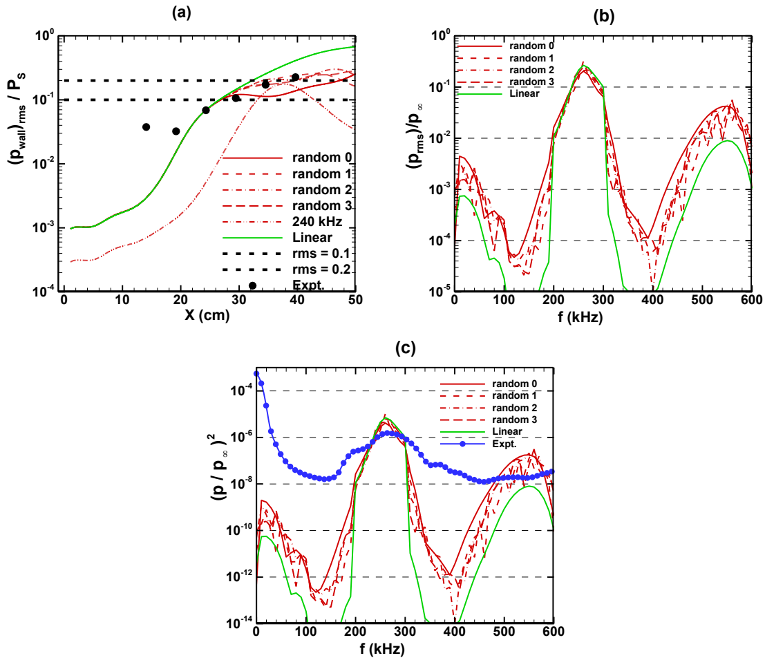
Figure 19. (a) Variations of the rms of the wall pressure fluctuations, (b) spectral amplitude of the pressure fluctuations at x = 30 cm, and (c) power spectral density at x = 30 cm for Case 2.
