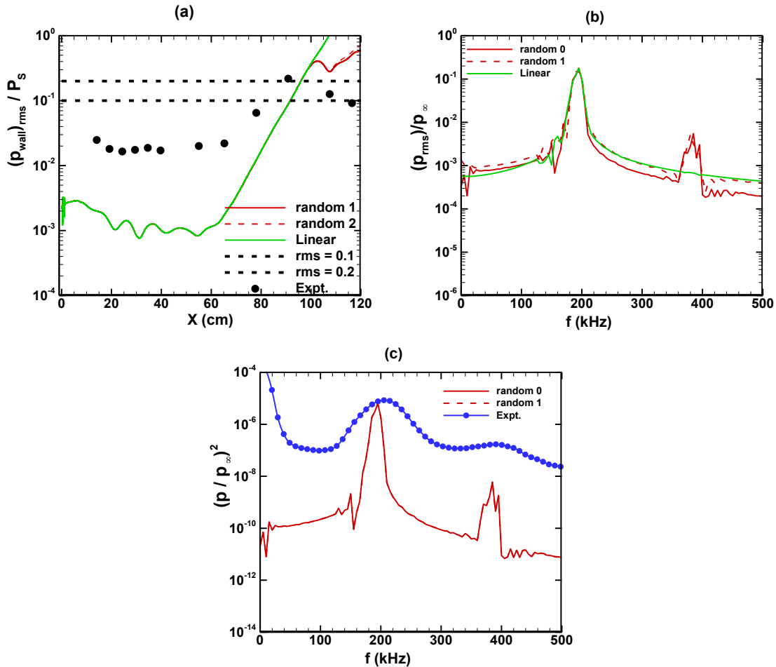
Figure 23. (a) Variations of the rms of the wall pressure fluctuations along the cone, (b) spectral amplitude of the pressure fluctuations, and (c) power spectral density at x = 90 cm for Case 4.
