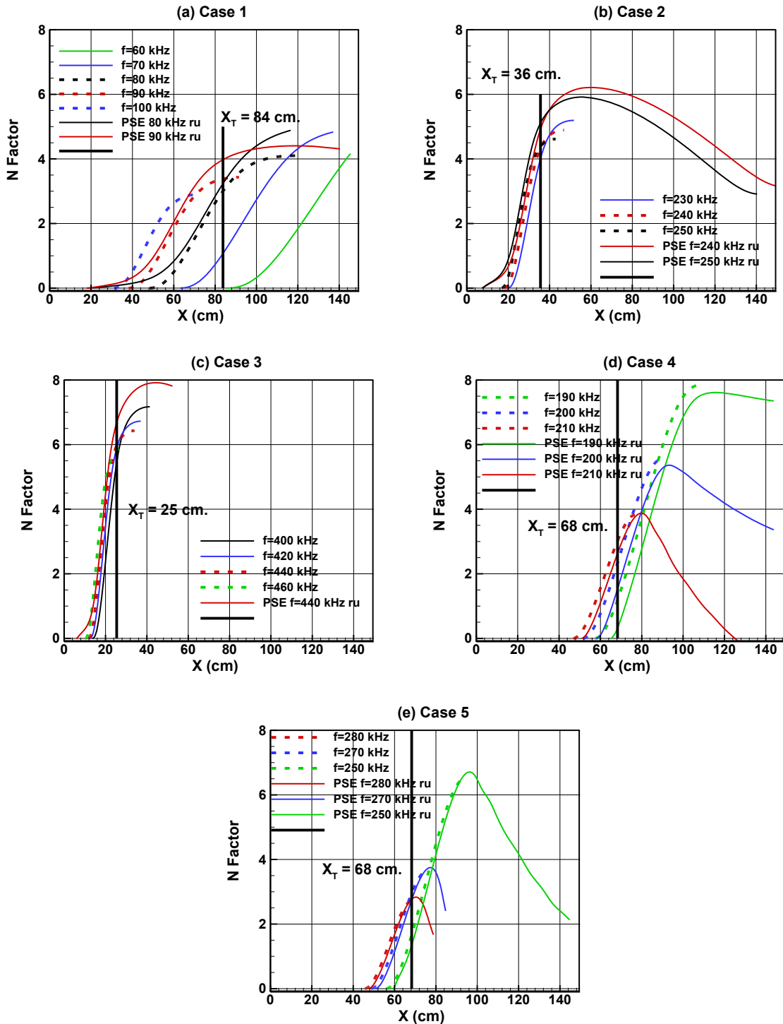
Figure 10. N-factor curves computed from the linear stability analysis and the PSE analysis based on (\rho u)_{max} for the (a) Case 1, (b) Case 2, (c) Case 3, (d) Case 4, and (e) Case 5.
