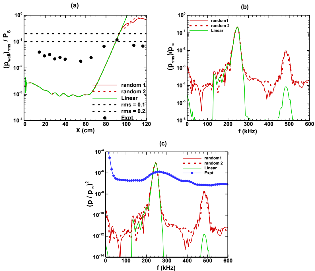
Figure 24. (a) Variations of the rms of the wall pressure fluctuations, (b) spectral amplitude of the pressure fluctuations at x = 90 cm, and (c) power spectral density at x = 90 cm for Case 5.
