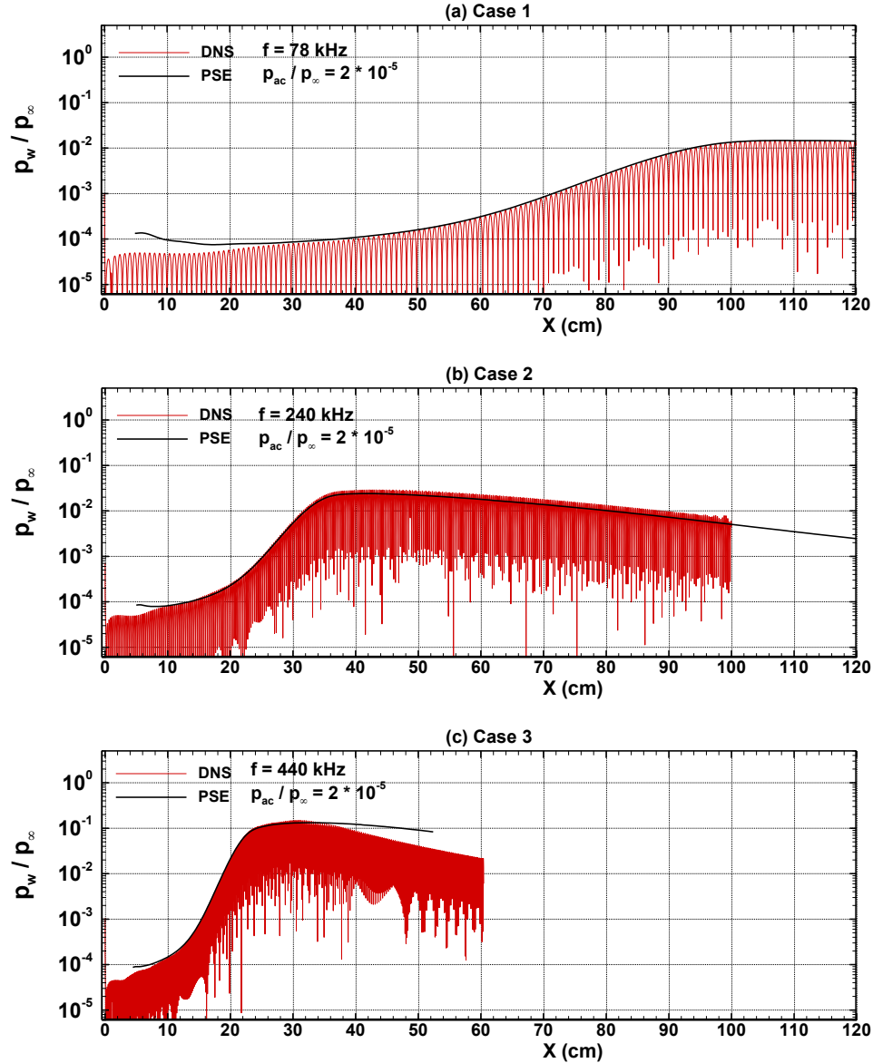
Figure 13. Amplitude of the pressure fluctuations on the wall generated by the slow acoustic wave for the (a) Case 1, (b) Case 2, and (c) Case 3.
