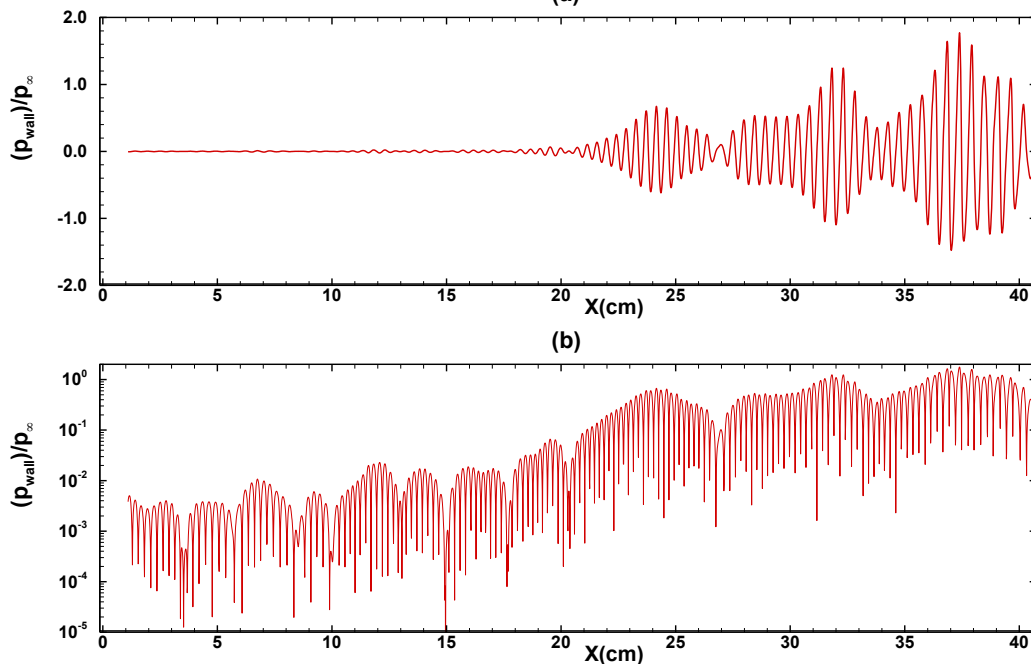
Figure 17. Amplitude of the pressure fluctuations on the wall generated by the slow acoustic waves for the Case 2 (a) in linear-scale, and (b) in log-scale.
