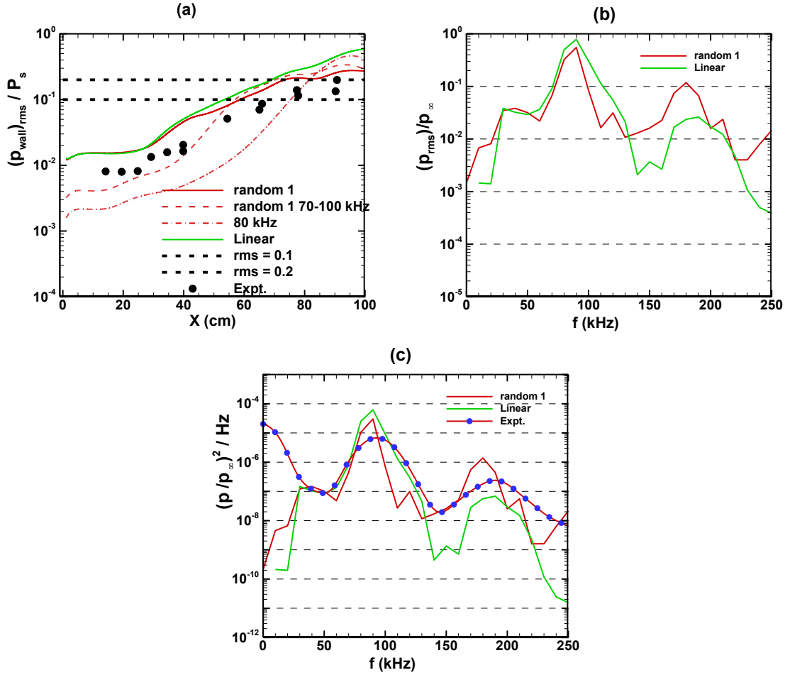
Figure 18. (a) Variations of the rms of the wall pressure fluctuations along the cone, (b) spectral amplitude of the pressure fluctuations at x = 80 cm, and (c) power spectral density at x = 80 cm for Case 1.
