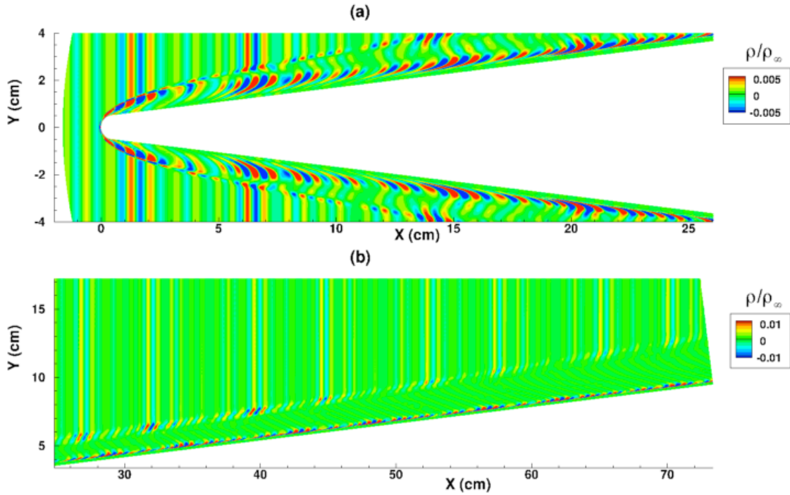
Figure 21. Density fluctuations generated by the interaction of broadband slow two-dimensional acoustic disturbances with the sharp cone for Case 5. (a) in a larger domain, and (b) inside the boundary layer.
