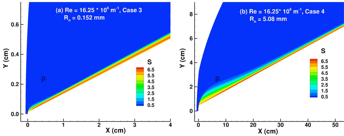
Figure 7. Contours of entropy for flow over the (a) sharp (Case 3), and (b) blunt (Case 4) cones (not to scale).
