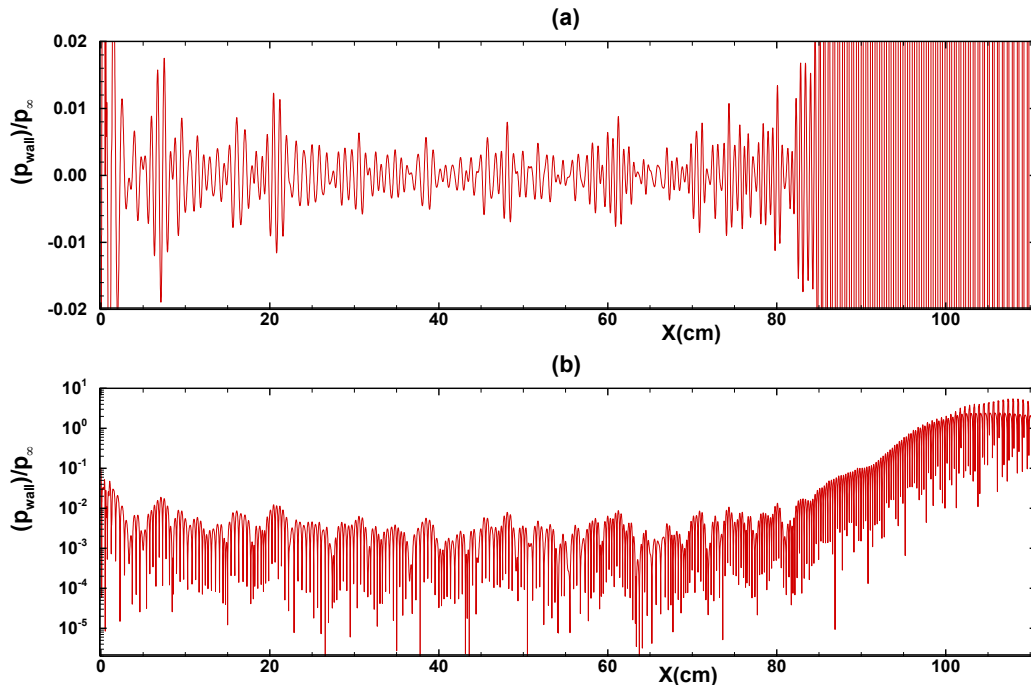
Figure 22. Amplitude of the pressure fluctuations on the wall generated by the slow acoustic waves for Case 5 (a) in linear scale, and (b) in log-scale.
