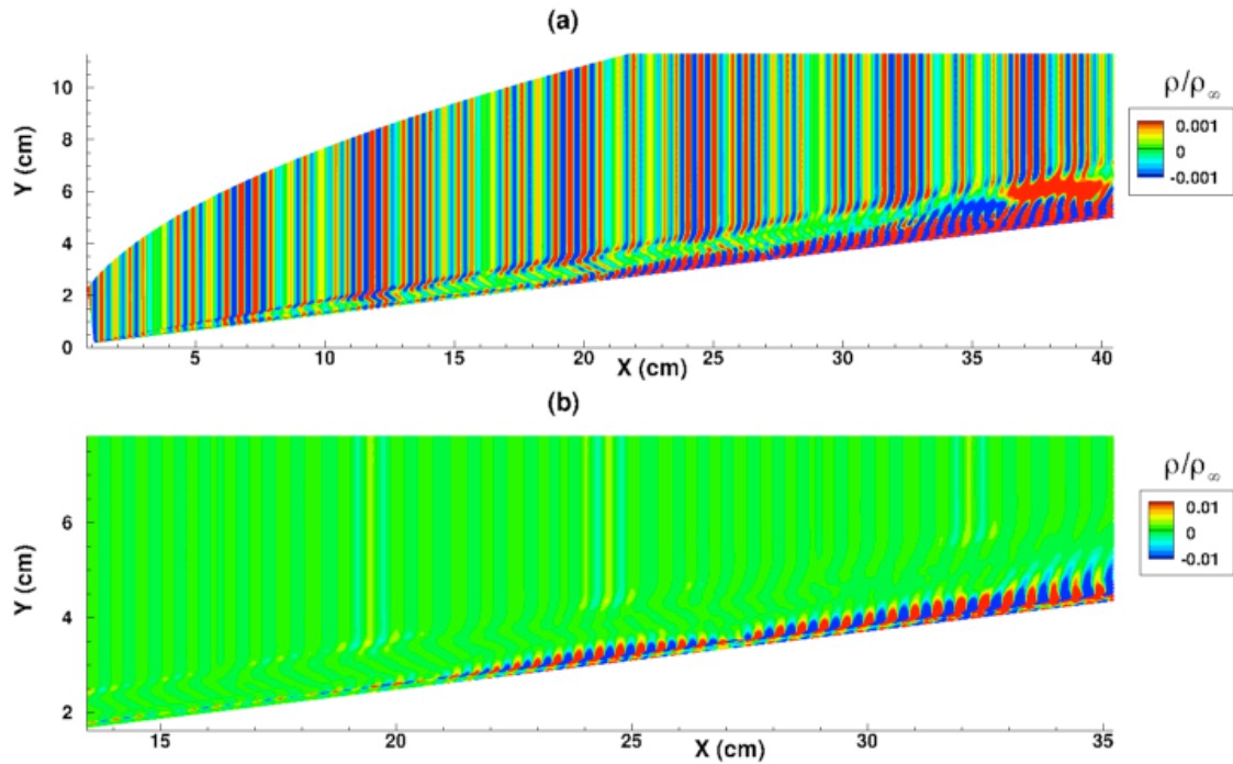
Figure 16. Density fluctuations generated by the interaction of broadband, slow two-dimensional acoustic disturbances with the sharp cone for the Case 2. (a) in a larger domain, and (b) inside the boundary layer
