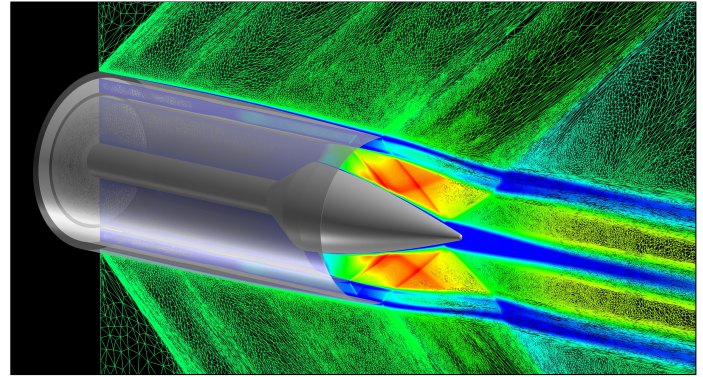
FIGURE 9. ADJOINT-BASED MESH ADAPTATION FOR AN ENGINE NOZZLE IN A SUPERSONIC EXTERNAL FLOW. TAKEN FROM [41].
