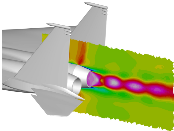
FIGURE 5. CROSS-SECTION OF ENGINE PLUME CONTOURS FOR MODIFIED F-15. TAKEN FROM [38].
