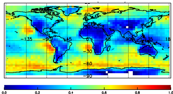
Figure 1. Mean low cloud amount from CALIOP, 2008 annual average.
