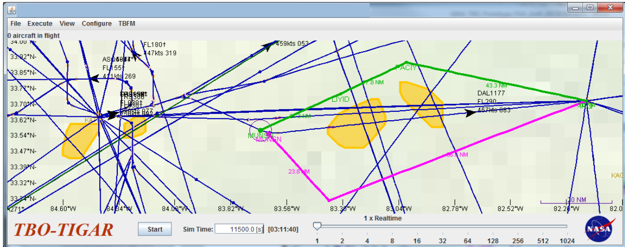
Figure 3. TBO-TIGAR plan view display with example DRNAV (green) and DRNP (magenta) re-routes.
