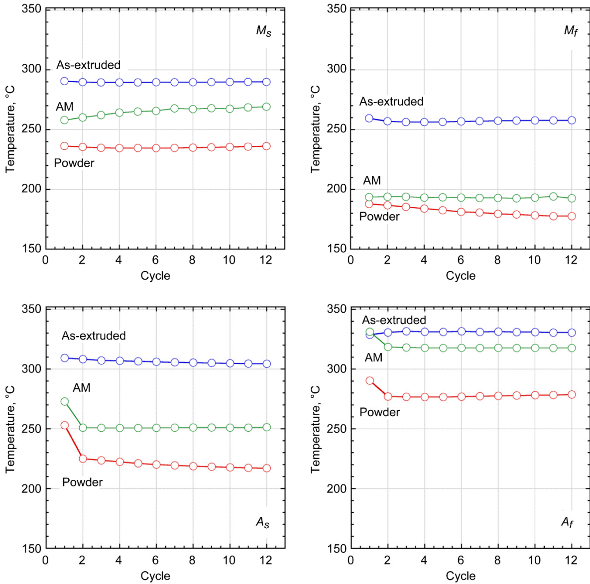
Figure 3.—Differential scanning calorimetry (DSC) curves for \text{Ni}_{49.8}\text{Ti}_{30.2}\text{Hf}_{20} as a function of cycle number.
