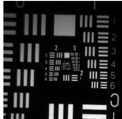
Figure 5. USAF-1951 resolution target. Image taken with 76.2 mm extension tube configuration.
