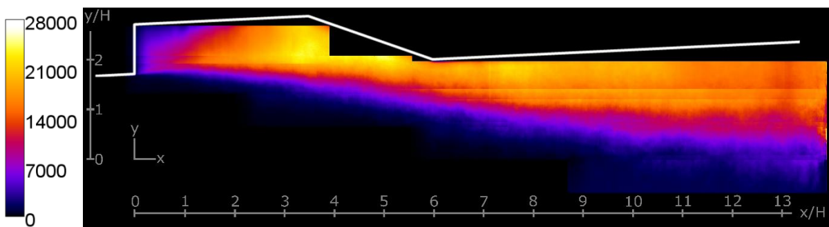
Figure 8. Mean OH PLIF signal intensity, Case A.
