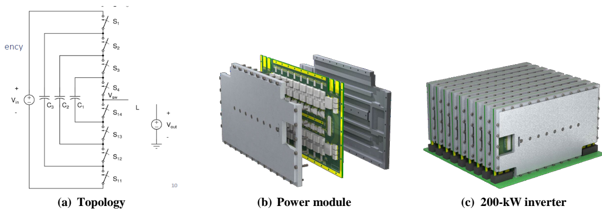
Figure 14. University of Illinois gallium nitride 200-kW inverter.
