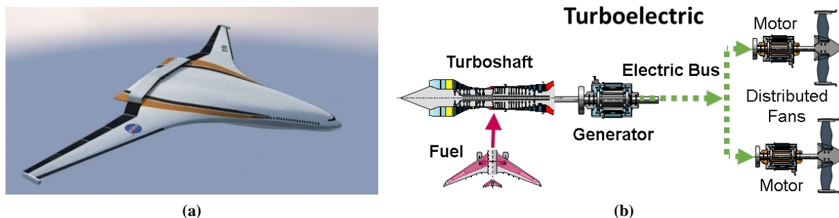
Figure 4. NASA N3-X.
