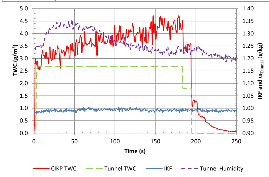
Figure 10. Transient results at V=152 m/s, T_o=-10^\circ\text{C} , p_o=100 kPa, MVD=22 \mu\text{m} and LWC=2.7 \text{g}/\text{m}^3
