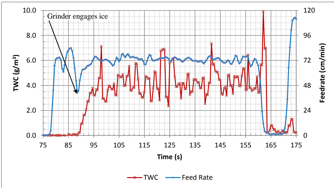
Figure 17. TWC from IKP and ice feed rate with time at a tunnel speed of 147 m/s, T_0 = -14^\circ\text{C}
