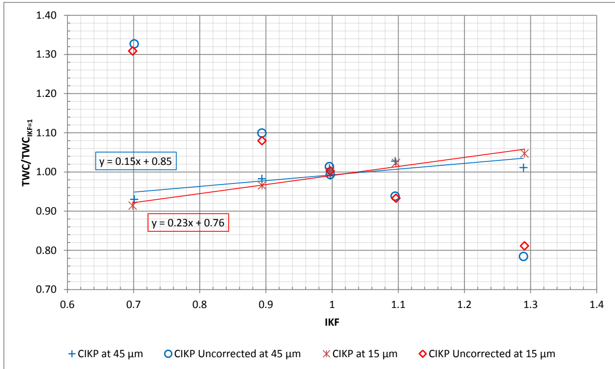
Figure 9. TWC divided by TWC at an IKF=1 with varying IKF at T_o = -10^\circ\text{C} , p_o = 100\text{ kPa} with average V = 77\text{ m/s} and LWC = 2\text{ g/m}^3 for sweeps with MVD = 15\ \mu\text{m} and 45\ \mu\text{m} . Least squares fits to the corrected data are shown
