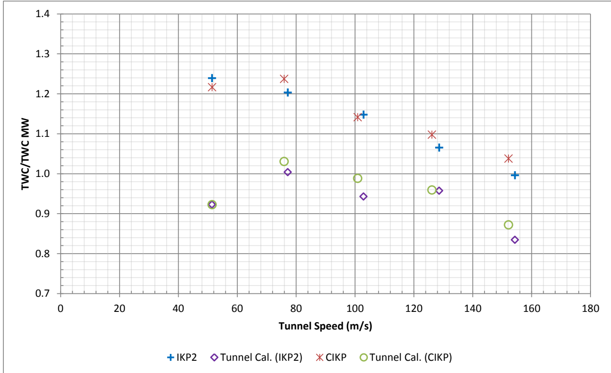
Figure 8. TWC divided by the corresponding MW TWC with varying air speed at T_0 = -10^\circ\text{C} , p_0 = 100\text{ kPa} with average MVD=22 \mu\text{m} and LWC =1.9 \text{g}/\text{m}^3
