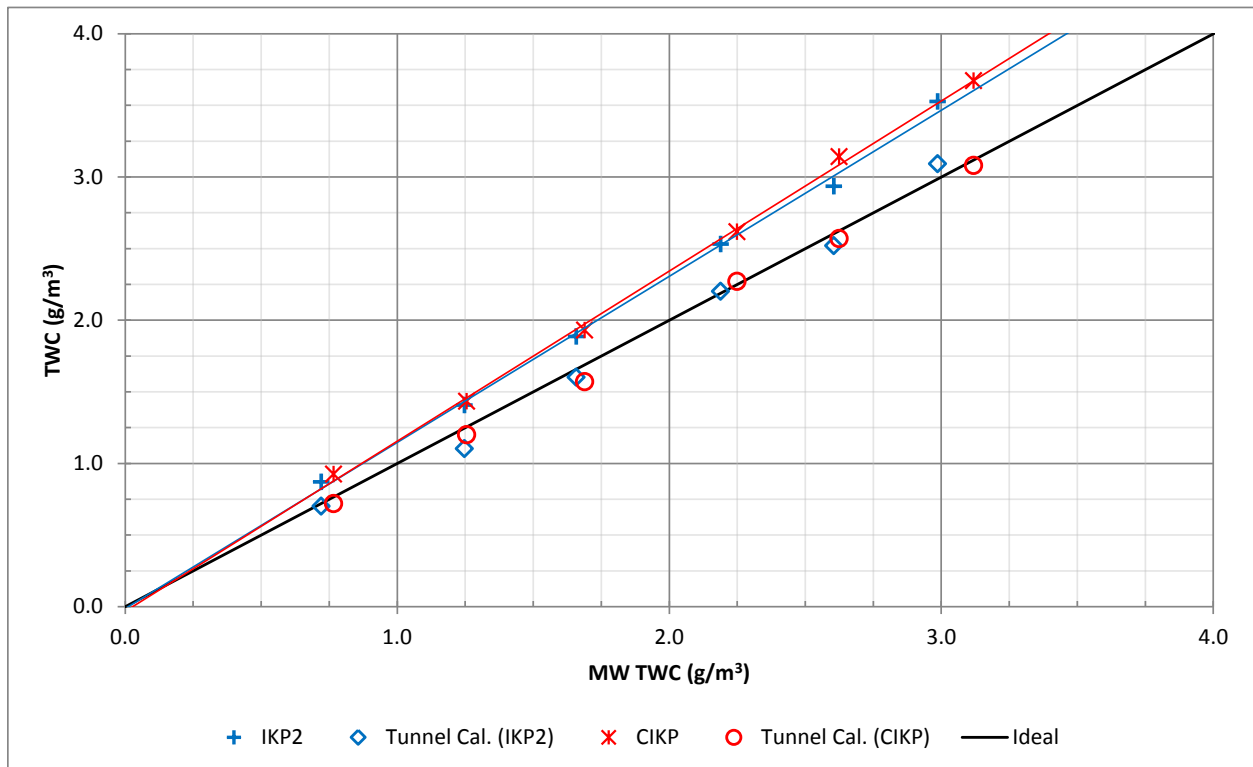
Figure 3. TWC results under liquid water conditions at T_o=-10^{\circ}\text{C} , p_o=100\text{ kPa} , V=77\text{ m/s} and nominal \text{MVD}=22\ \mu\text{m} with least squares fit lines for IKP results
