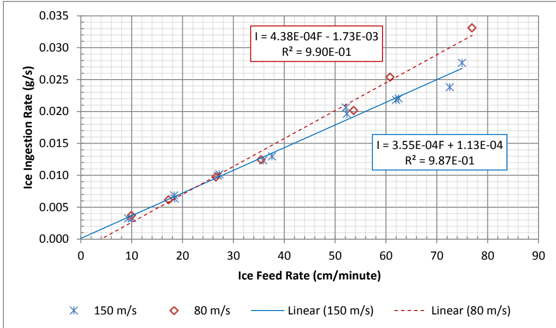
Figure 16. Ice ingestion rate versus feed rate for 80 and 150 m/s
