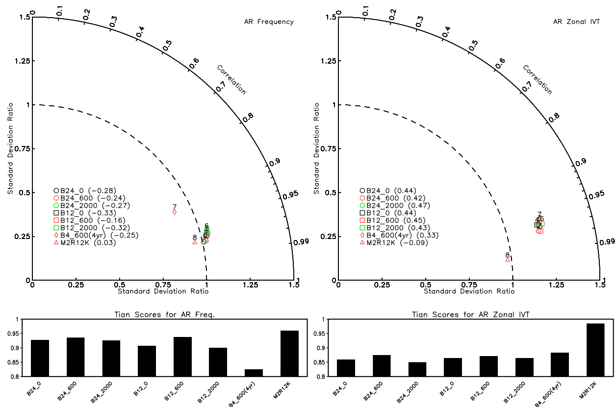
Figure 17. (upper) Taylor diagram based on comparing the spatial patterns of AR frequency between MERRA-2 (the reference) and different downscaling experiments. Numbers in brackets indicate the mean bias between the two maps being compared normalized by the standard deviation of the reference map. (lower) Tian scores. Note that the vertical scale starts from 0.8 to better visualize the differences.
