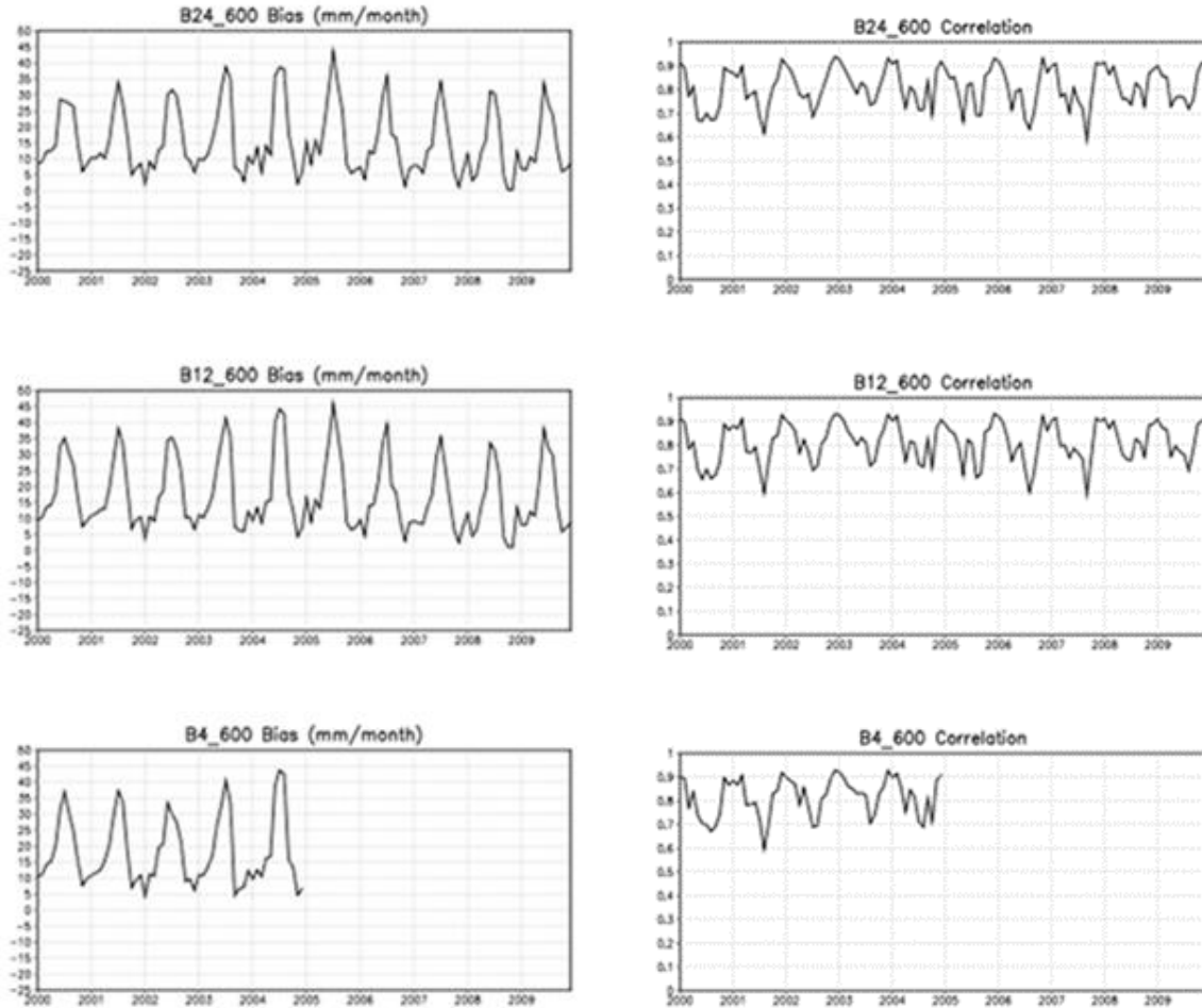
Figure 14. Area-mean bias (left) and spatial correlation (right) of monthly precipitation between models and PRISM, for the three model resolutions: B24_600 (top row), B12_600 (middle row), and B4_600 (bottom row).
