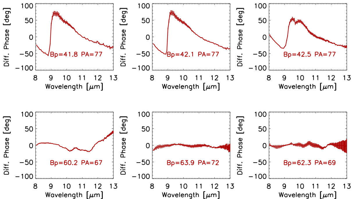
Fig. 4. Non-zero differential phases measured by MIDI for R Leo ordered in increasing projected baseline ( B_p ).
