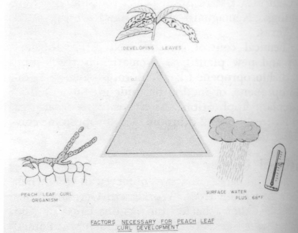
Environmental factors necessary for peach leaf curl development.
