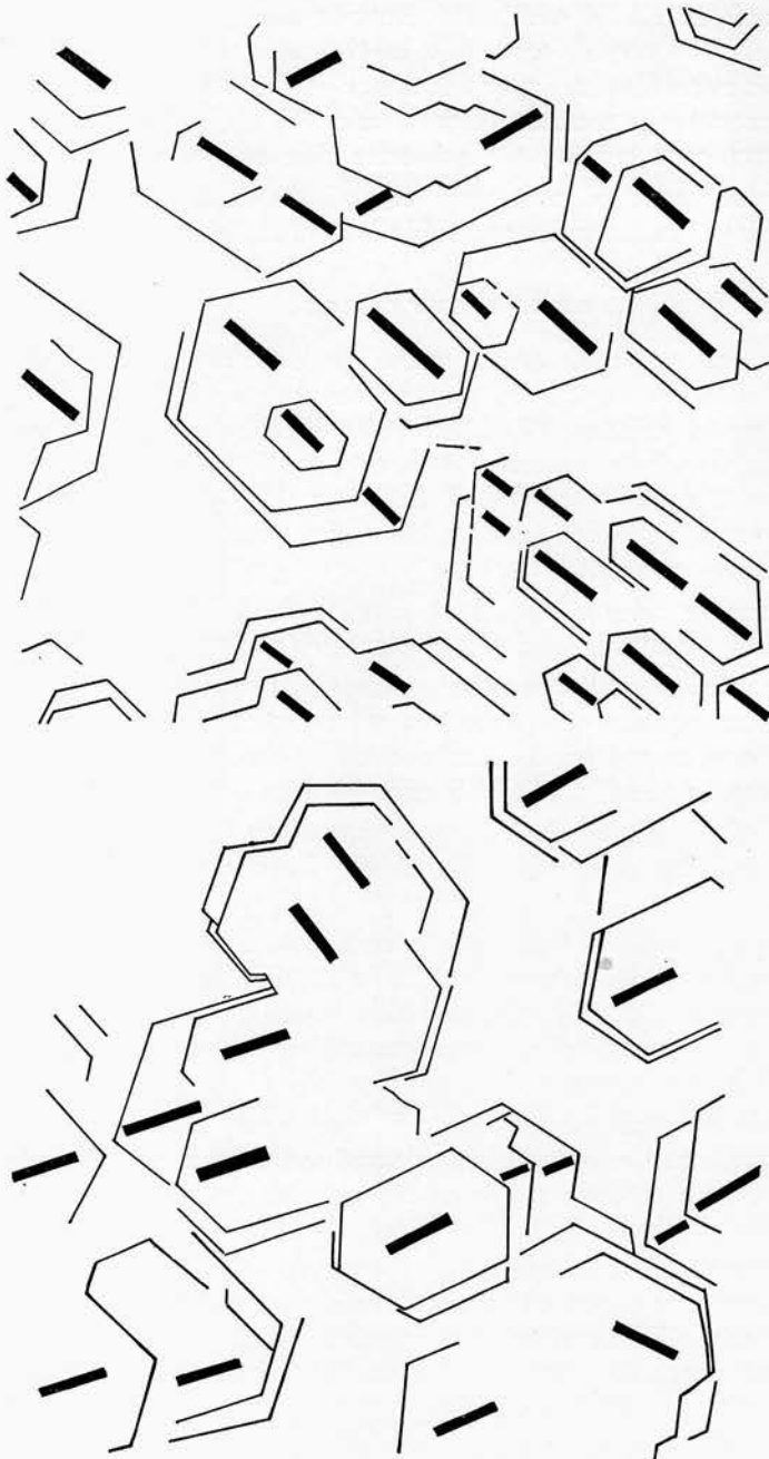
Textfig. 2. — See fig. 45. Nautilus pompilius LAMARCK. Two representative fields of the concave adoral surface of the penultimate septum. The outlines of hexagonal crystals and the direction of their a-axis (thick lines) are shown. The crystals exhibit parallel growth and overgrowth, aggregation predominantly along the (010) plane. Note the divergent direction of the a-axes in closely adjacent groups of crystals.
