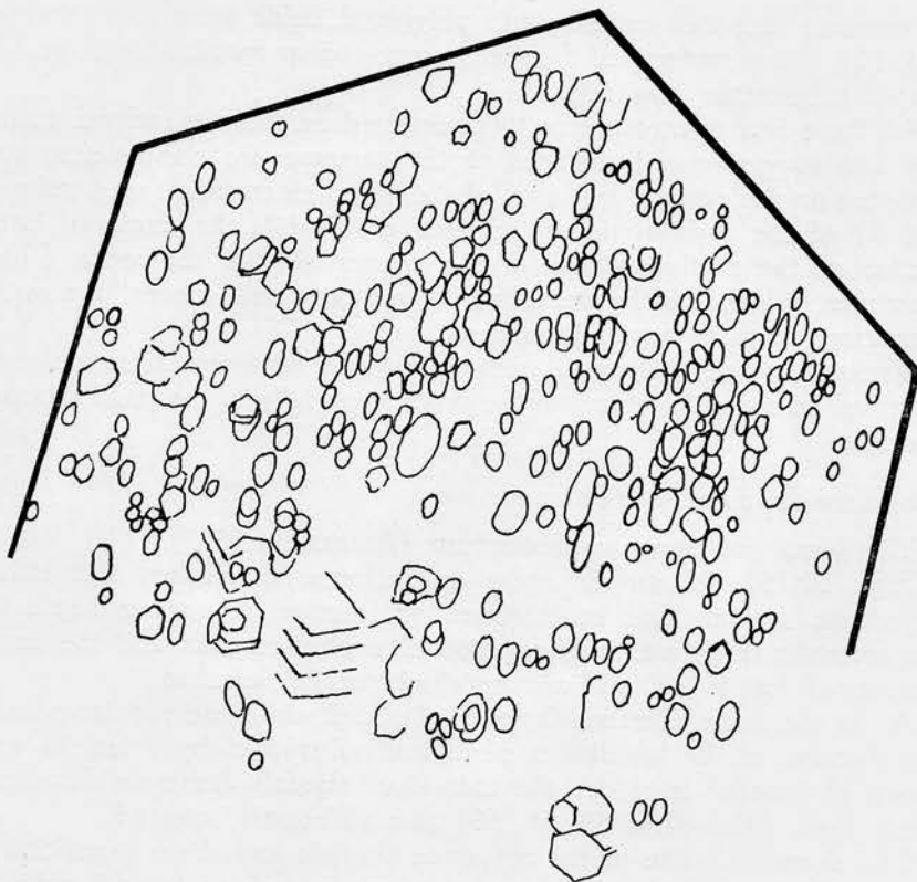
Textfig. 3. — Nautilus pompilius LAMARCK. Concave adoral surface (unetched) of the penultimate septum.
