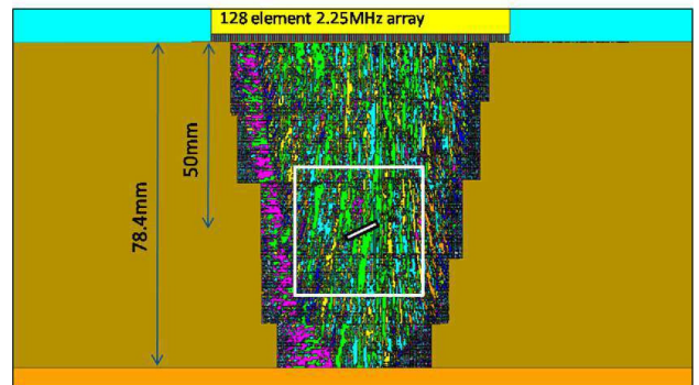
Figure 3. Geometry input to the finite element simulation where a 5 mm crack with 40^\circ orientation (relative to the horizontal axis) is embedded in an austenitic weld microstructure. The 128 element 2.25 MHz array is placed directly above the flaw over the weld material. The white box depicts the sampling domain.
