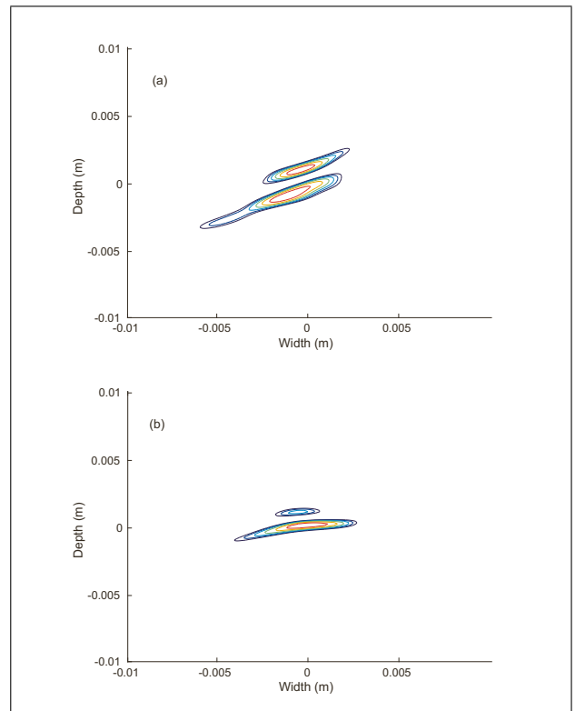
Figure 10. Reconstructions plotted at the -6 dB threshold of (a) the 5 mm crack embedded within the anisotropic steel weld and (b) the 2.5 mm diameter disc embedded to the left of the weld (see Tables I and II respectively) by the Total Focussing Method.
