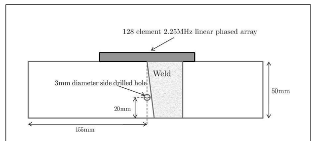
Figure 5. This schematic depicts a cross section (the x - z plane in which we are interested) of a steel sample containing an ultrasonically noisy MMA weld. A 3 mm diameter flaw is embedded in the parent material to the left of the the weld (marked by the hatched area) and the 128 element 2.25 MHz array is placed centrally above the defect, over the parent and weld materials.
