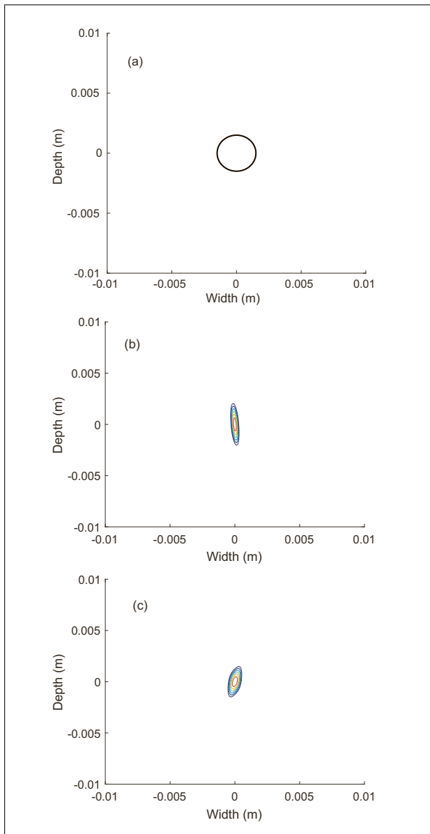
Figure 11. The geometry of the 3 mm diameter disc is plotted in (a). Reconstructions from FMC data arising from the phased array inspection of a steel block (see Table II) by the Factorisation Method applied to (b) the scattering matrix arising at 2.25 MHz and (c) the multi-frequency scattering matrix.
