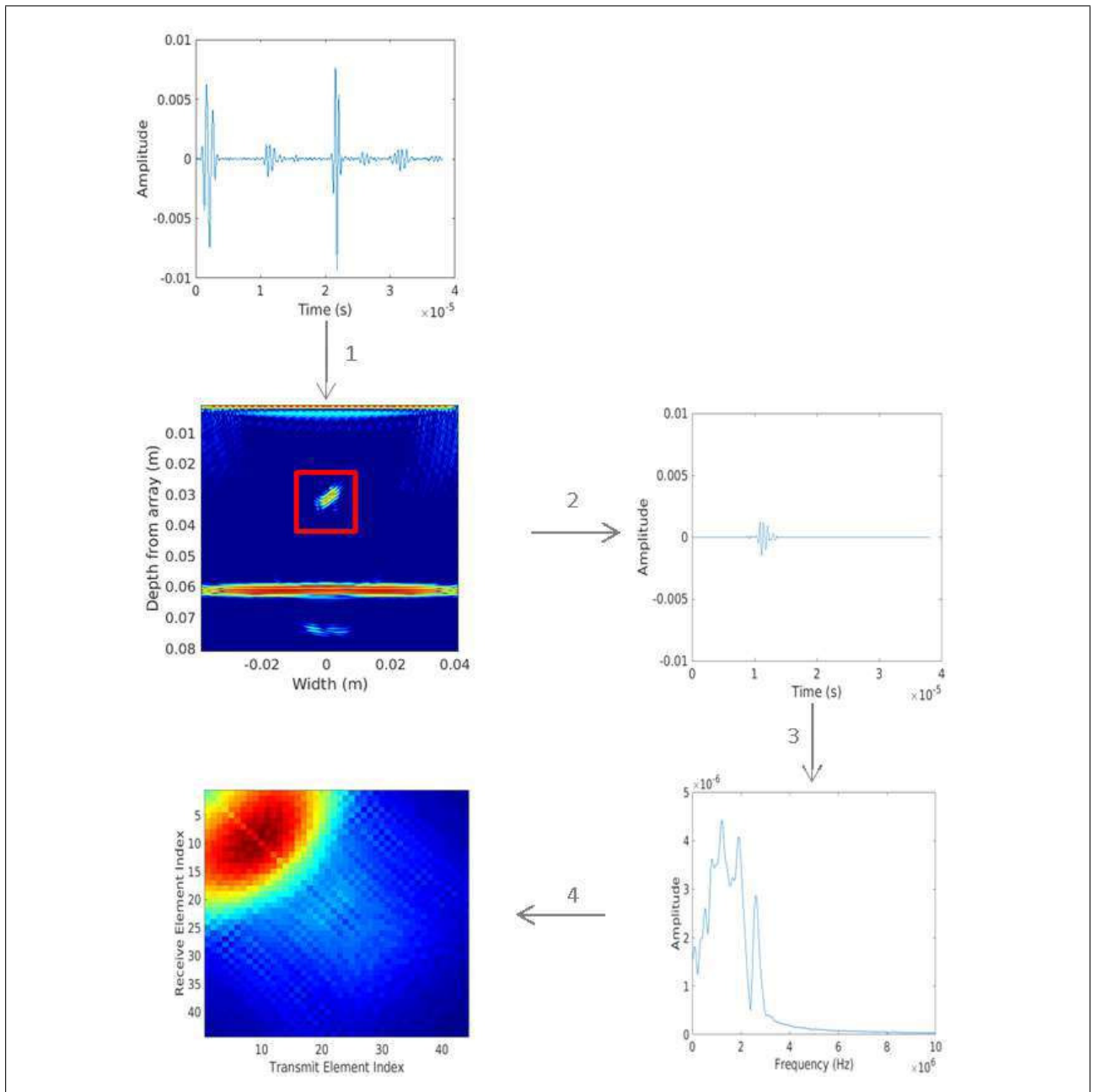
Figure 2. Processing of time domain FMC data for extraction of scattering matrices. Firstly the flaw is located using the standard TFM. Then, the distance of the defect from the array coupled with the estimated wave speed gives rise to a time interval pertaining to scattering by the defect. The Fourier transform is applied to the FMC data in this interval. Then, the amplitude at a specified frequency is plotted for each transmit-receive pair to generate the scattering matrix.
