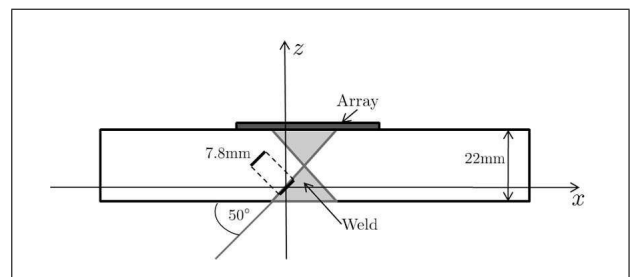
Figure 6. This schematic depicts a cross section (the x - z plane in which we are interested) of the stainless steel test sample constructed from welded austenitic plates of 22 mm depth. A lack-of-fusion crack of 7.8 mm length lies along the left hand side of the weld (marked by the shaded area) at an angle of 50° (relative to the horizontal axis).
