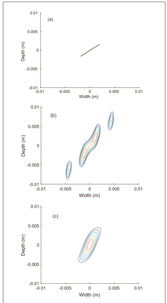
Figure 7. Crack reconstructions from FMC data arising from finite element simulation of the scattering of ultrasonic waves by a 5 mm crack with 40^\circ orientation embedded in a homogeneous medium. Image (a) depicts the known defect size and geometry. This was reconstructed by (b) the Factorisation Method applied to the scattering matrix arising at 1.5 MHz and (c) the Factorisation Method applied to the multi-frequency scattering matrix.
