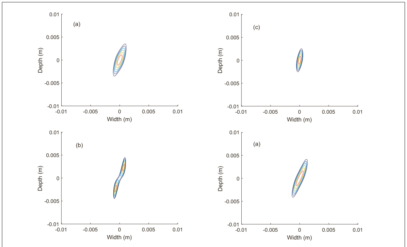
Figure 8. Crack reconstructions from FMC data arising from finite element simulation of the scattering of ultrasonic waves by a 5 mm crack with 40^\circ orientation embedded in a heterogeneous medium by the Factorisation Method applied to (a) the scattering matrix arising at 1.5 MHz, (b) the scattering matrix arising at 1.5 MHz regularised by the TSVD ( m = 10 ), (c) the multi-frequency scattering matrix and (d) the multi-frequency scattering matrix regularised by the TSVD ( m = 4 ).
