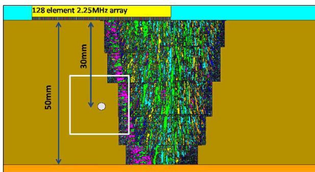
Figure 4. Geometry input to the finite element simulation where a 2.5 mm diameter side-drilled hole is embedded in the parent material (stainless steel) close to a highly scattering polycrystalline region which represents an austenitic steel weld. The 128 element 2.25 MHz array is placed directly above the flaw over the parent and weld materials. The white box depicts the sampling domain.
