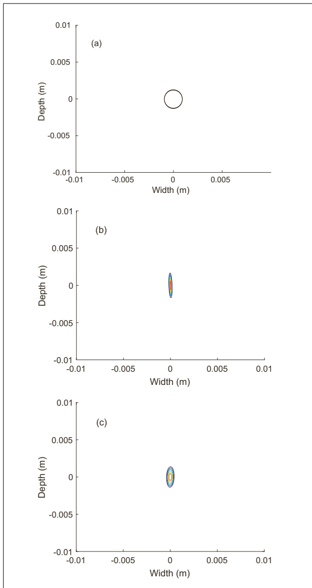
Figure 9. Reconstructions of a 2.5 mm diameter disc as shown in image (a) from FMC data arising from finite element simulation (see Table III) by the Factorisation Method applied to (b) the scattering matrix arising at 2.25 MHz and (c) the multi-frequency scattering matrix.
