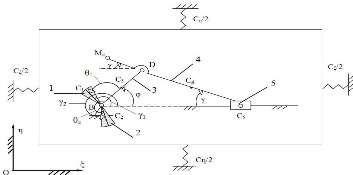
Figure 1. 1, 2 – loose pendulums axle-mounted on the crankshaft, 3 – crankshaft, 4 – crank rod, 5 – slider, M_k – correction mass.
