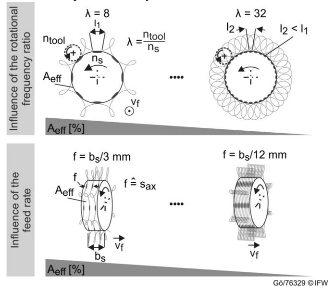
Fig. 3 Effective contact area
