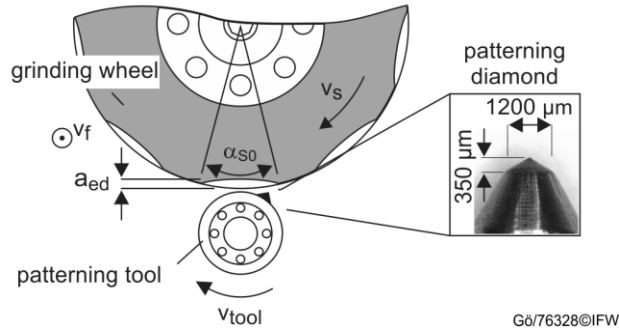
Fig. 1 Patterning process
