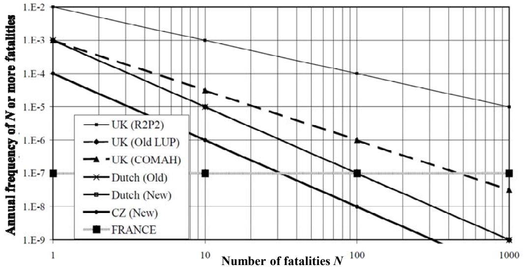
Fig. 1: F-N curves relating expected fatalities ( N ) from an accidental event or failure and the annual frequency of occurrence ( F ) of events with not less than N fatalities in various countries [23]
