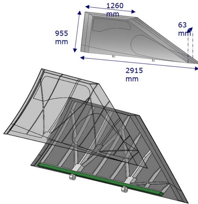
Figure 21 Rudder design
