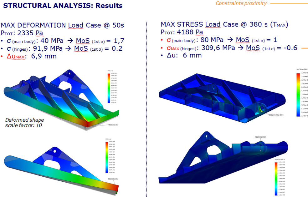
Figure 20 Flap mechanical analysis results
