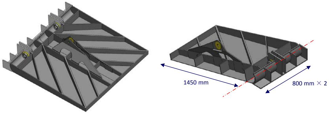
Figure 17 Flap design
