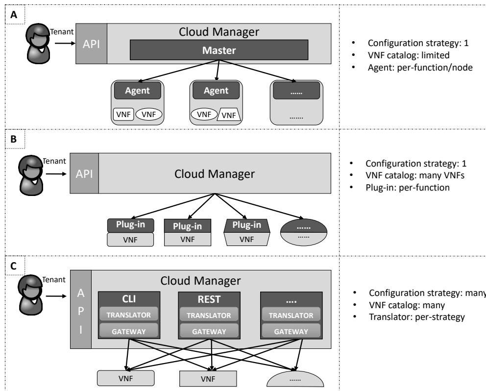
Fig. 4.2 Possible configuration-oriented CM architectures.
