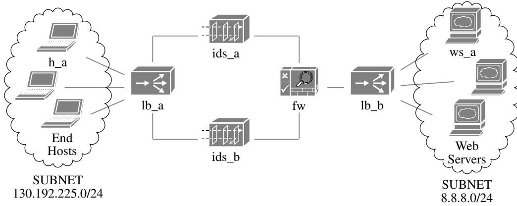
Fig. 2.1 Topology example.
