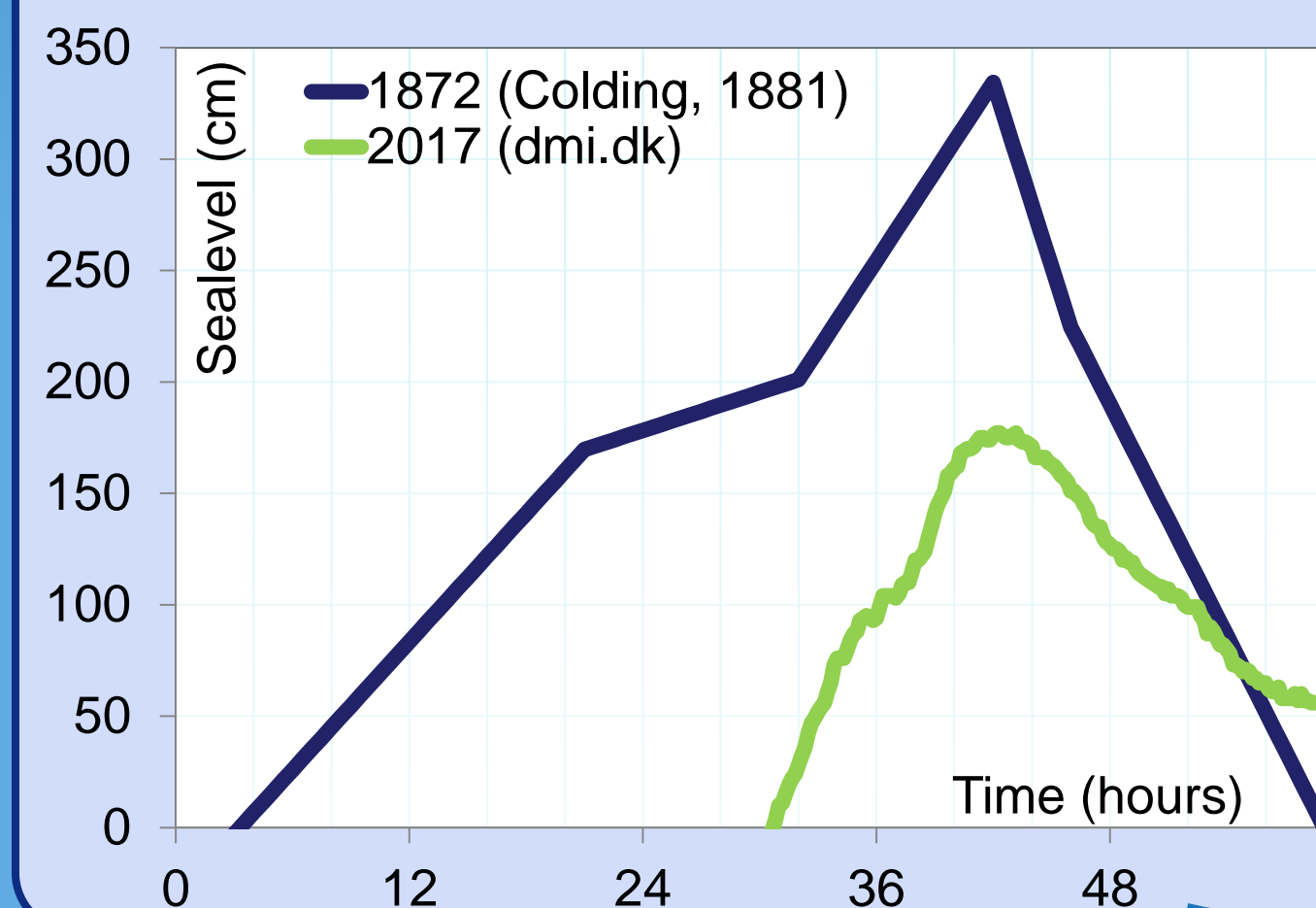
Above: Damages the storm surge in 1872. Ref: Holger Drachmann, Illustreret Tidende. Left: Sea level (cm) in the Danish town Aabenraa during the storm surges of 1872 and 2017. Right: Sea level (meters) reconstructed by the Danish Coastal Authorities (2011).
