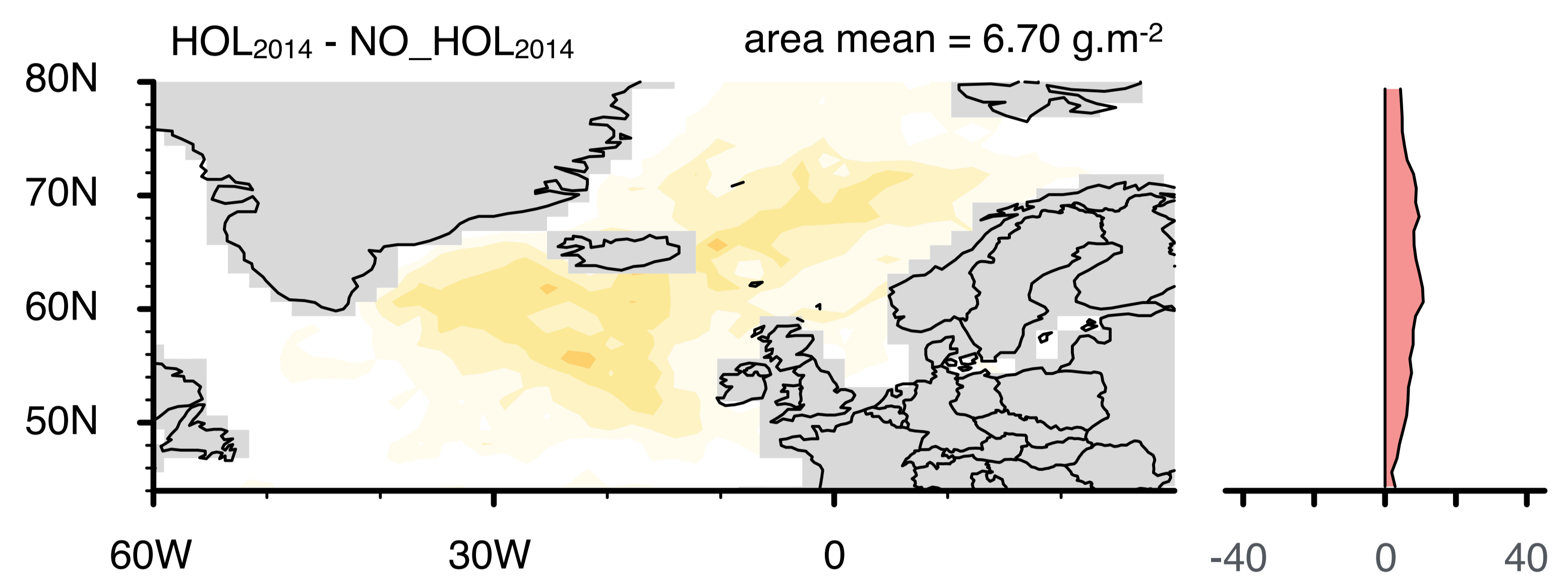
CAM5-NCAR
