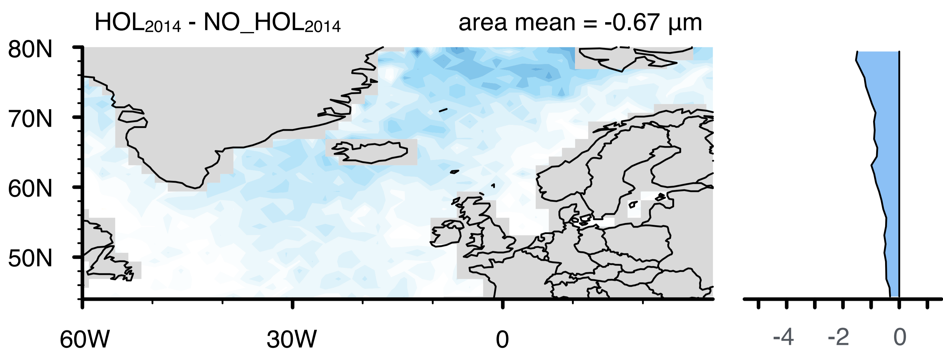
HadGEM3-CLASSIC
