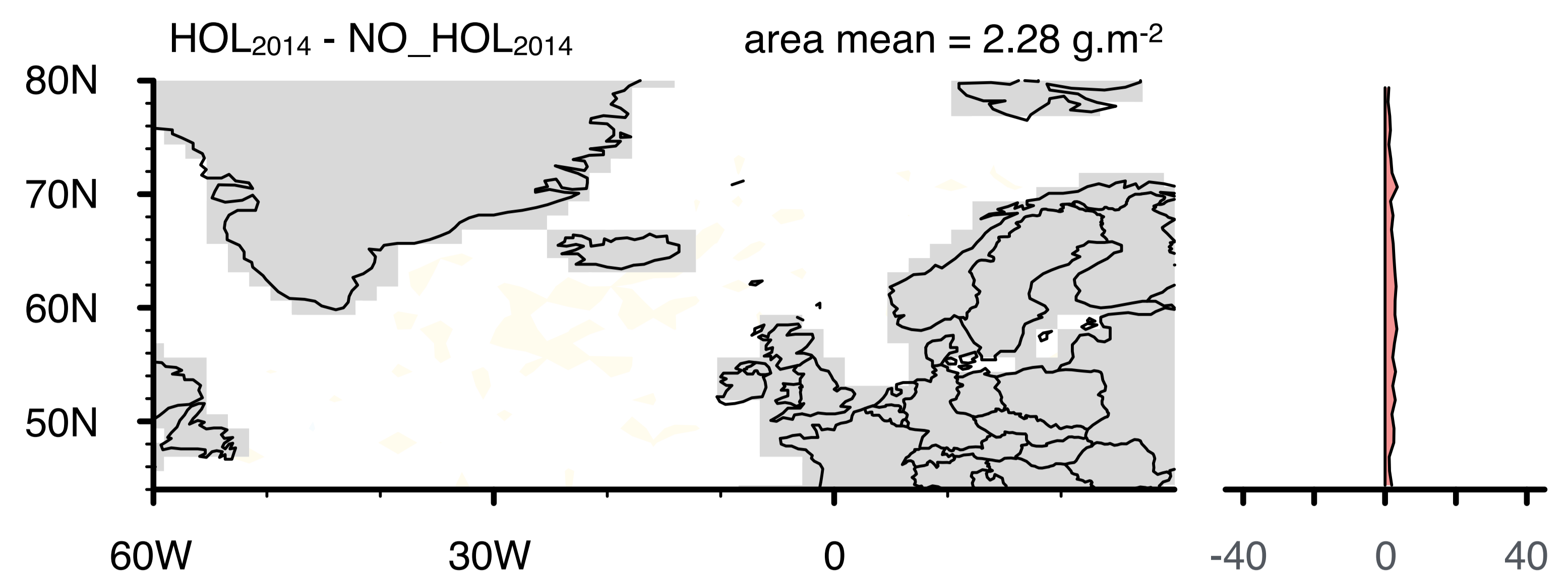
HadGEM3-CLASSIC
