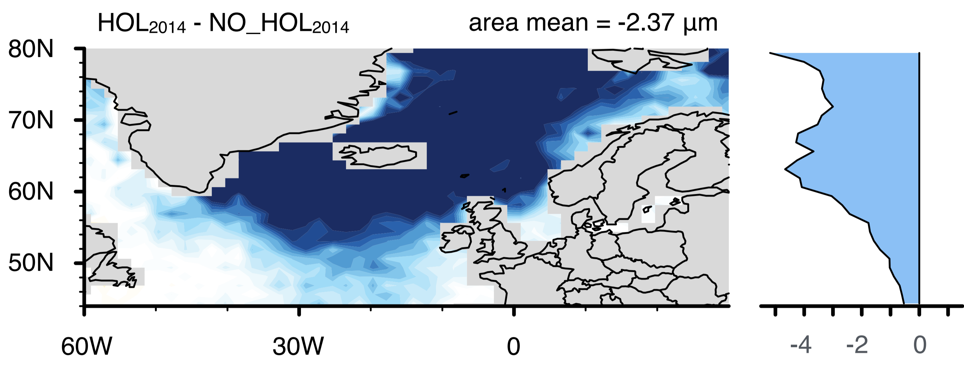
CAM5-NCAR
