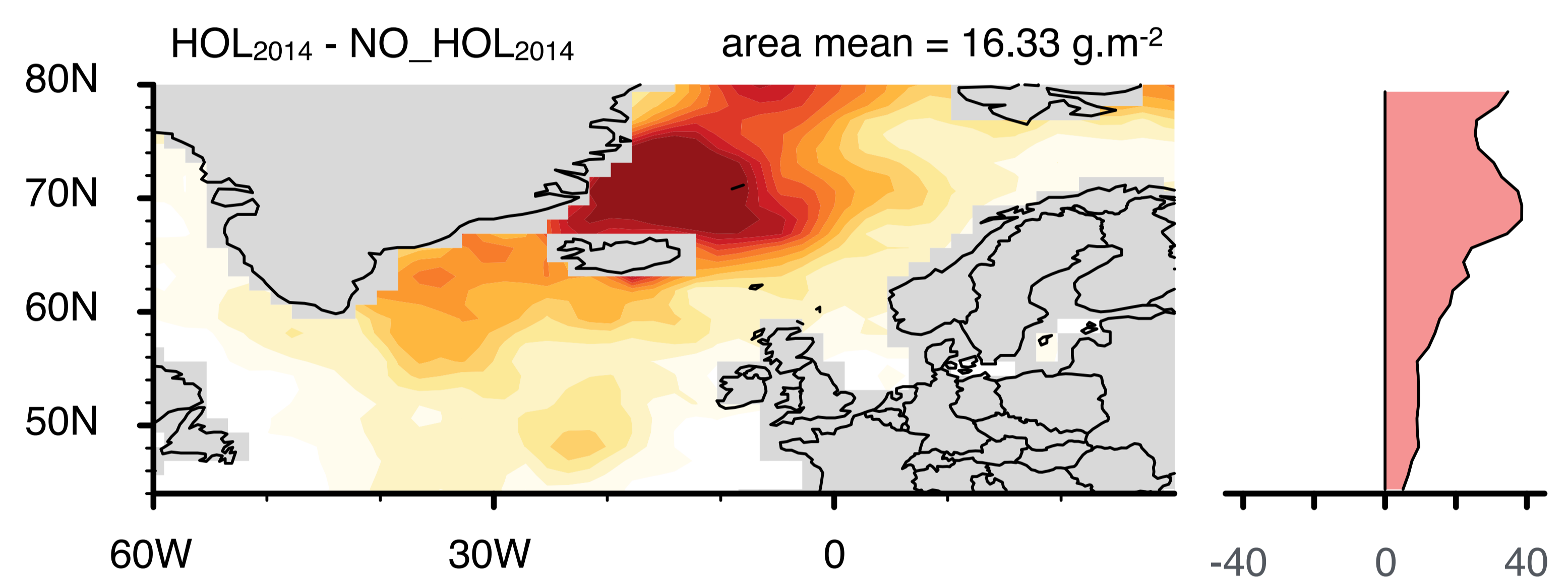
CAM5-Oslo
