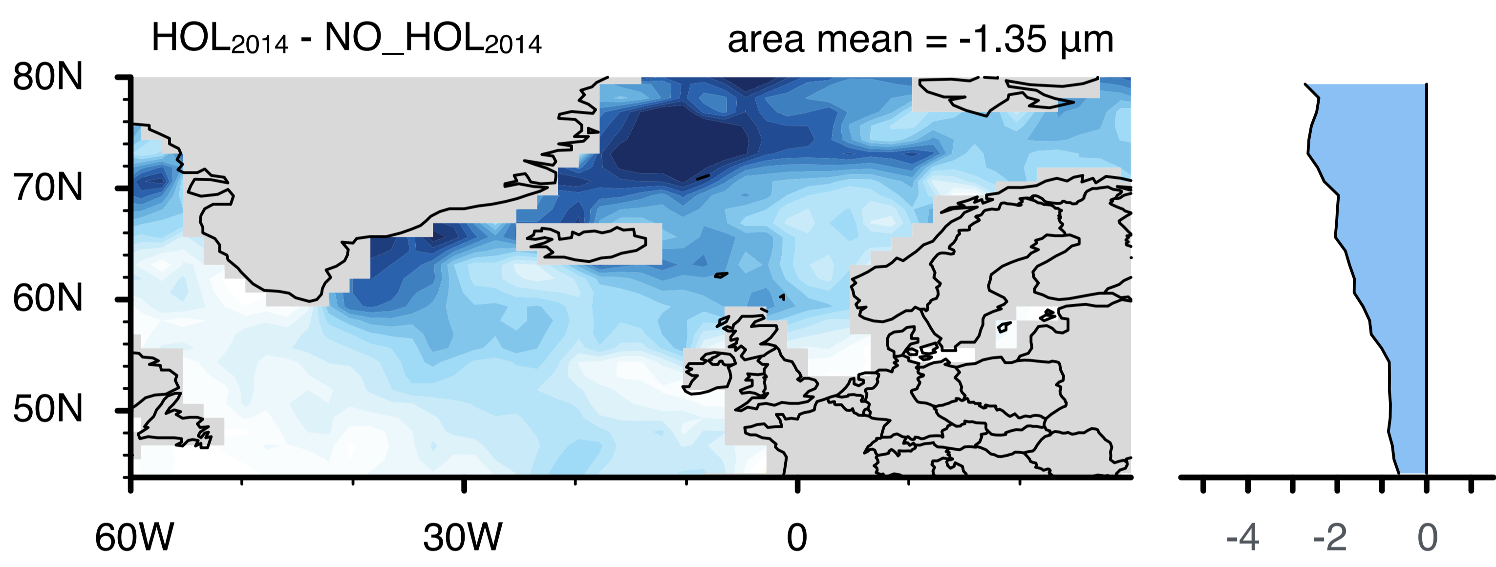
CAM5-Oslo
