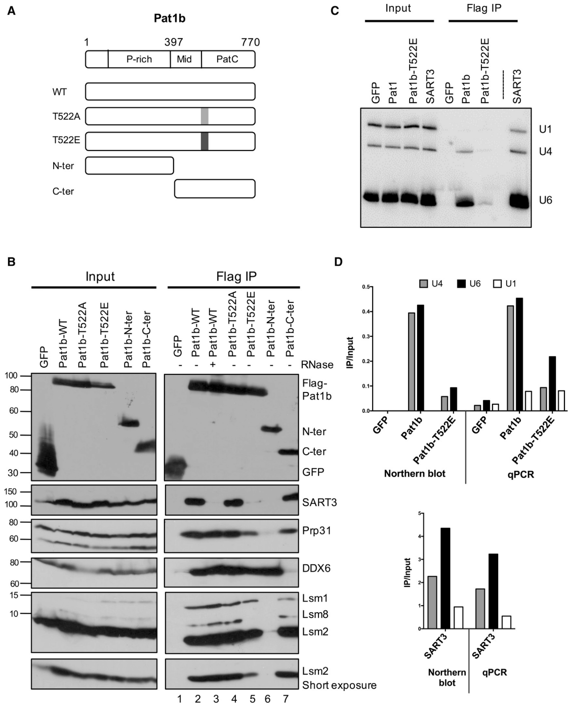
Figure 2. Pat1b Interacts with Tri-snRNP Protein and RNA Components
