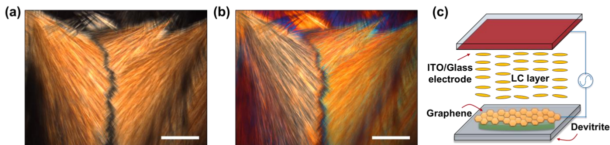
Figure 1. Devitrite-based tunable optical diffusers. (a) Polarized light microscope image showing different arrangements of devitrite crystals within a 30 \mu\text{m} thin slice of heat-treated soda–lime–silica float glass. Scale bar = 500 \mu\text{m} . (b) The image of the region in (a) taken with a sensitive tint wave plate inserted at 45^\circ to the polarizer and probe. Scale bar = 500 \mu\text{m} . (c) Schematic of the tunable devitrite-LC electro-optical device.
