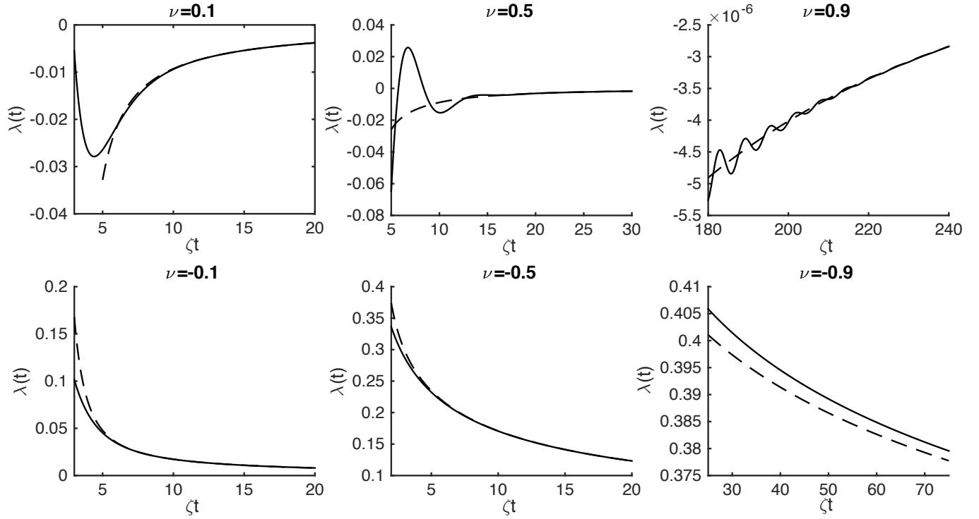
Fig. 3. Comparison at long times of the integral expression, (15), of the noiseless Green function (solid line) with its series approximation (dashed line), (18). The latter consists of the first 5 terms for 3 values of \nu , 0.1 (left), 0.5 (center), and 0.9 (right) over differing time ranges.
