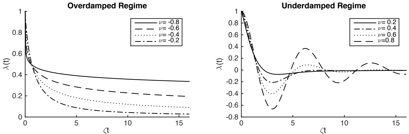
Fig. 1. The noiseless Green function, \lambda(t) , for varying \nu in (14) over the overdamped (left) and underdamped (right) regimes in the range [-0.8, -0.2] and [0.2, 0.8] in steps of 0.2. Time is plotted in units of 1/\zeta . As \nu is made more negative, \lambda(t) approaches 0 more slowly. As \nu is made more positive, the amplitude of the oscillations increases and they last longer.
