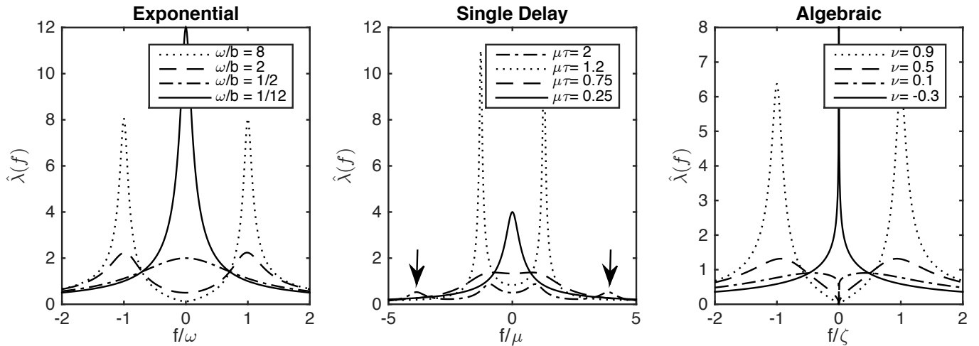
Fig. 5. Motional narrowing in the dependence of the a.c. susceptibility on the frequency, f , of the applied electric field. All three cases, exponential (left), single delay (center), and algebraic (right), display two peaks in the coherent limit which, as damping is increased, initially broaden more and more and move towards each other (to the center, i.e., the region f = 0 ). On increasing the damping beyond a critical value in each case, however, the line narrows rather than broadens as the damping is increased. Frequency is plotted on the horizontal axis in units of the coherent parameter \omega , \mu and \zeta for the three respective cases. Units along the vertical axis are arbitrary. Two arrows in the central panel locate the additional peaks that develop for the single delay process. The sharp transition at f = 0 for the algebraic memory, which is a jump from a vanishing to an infinite value, can be seen when comparing the \nu = -0.3 case with the \nu = 0.1 case.
