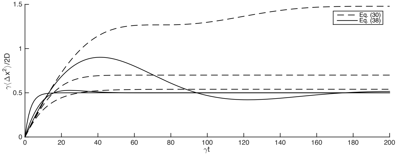
Fig. 8. Time-dependence of the extent of the particle (as measured by the value of the MSD) and apparent violation of the Balescu-Swenson theorem. The MSD for the exponential memory is plotted for a constant \gamma and three values of the damping parameter b/\gamma : 0.5, 2.5 and 12.5. The correct results as given by our theory, (30), correspond to the dashed lines. Their saturation values are seen to increase as b/\gamma is increased. As all cases have the same \gamma , that increase signifies a violation of the Balescu-Swenson theorem. By contrast, all three solid lines which are predictions of the incorrect generalization, (38), of the Smoluchowski equation (see text) saturate to the same single value (as given by the time-local equation) even though the corresponding values of b/\gamma are different (as in the respective dashed line cases).
