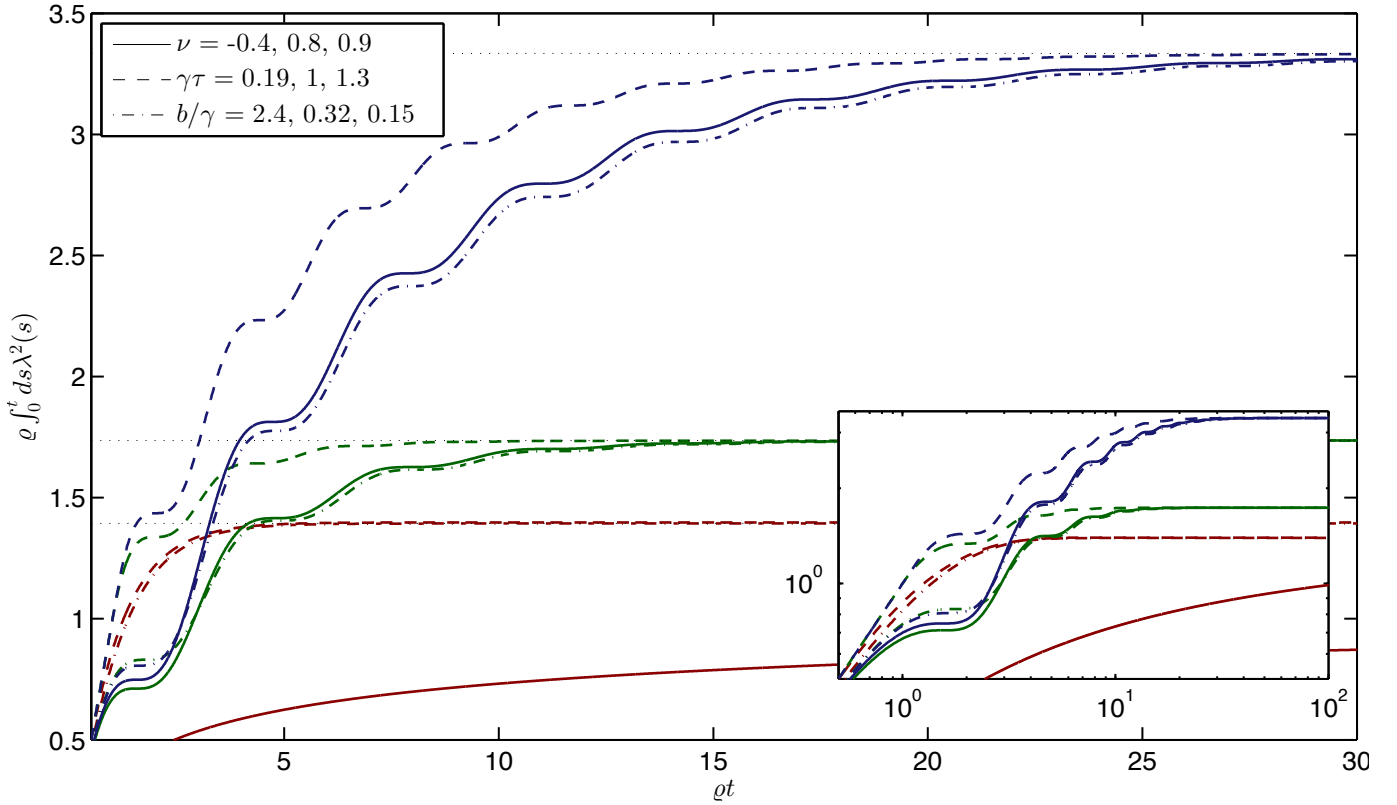
Fig. 7. Comparing the dynamics of the MSD for the algebraic ( straight line ), exponential memory ( dot-dashed line ) and single delay ( dashed line ) memories when their MSD have a mutual saturation value. We set \rho equal to the coherent parameter for each of the memories divided by the diffusion constant, i.e., \omega for exponential, \mu for the single delay, and \zeta for the algebraic respectively. Two curves for each memory depict dynamics in the underdamped regime and one for each memory in the overdamped regime. The inset plot shows that same figure with logarithmic axes.
