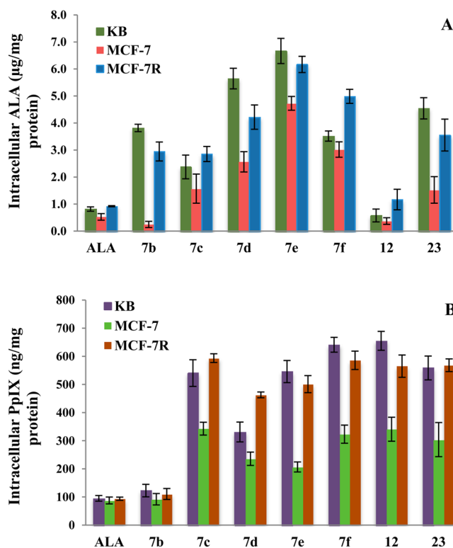
Figure 7. (A) Chemically extracted cellular concentrations per mg protein of intracellular ALA or ALA–HPOs with cellytic after 2 h incubation at 100 \mu M. (B) PpIX cellular concentrations per mg protein measured at 24 h by chemical extraction using cellytic following 2 h incubation with ALA and ALA–HPO conjugates at 37 ^{\circ} C.
