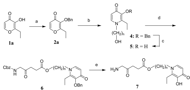
Scheme 1. Synthesis of ALA–HPO Conjugates 7 a
