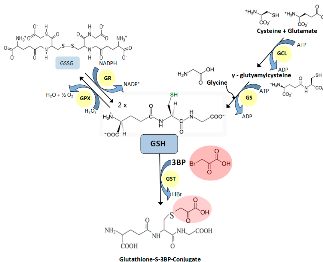
Figure 2. Glutathione metabolism. Crucial enzymes involved in glutathione metabolism: GCL—γ-glutamylcystine synthetase; GS—glutathione synthetase; GR—glutathione reductase; GPX—glutathione peroxidase; GST—glutathione S-transferase.
