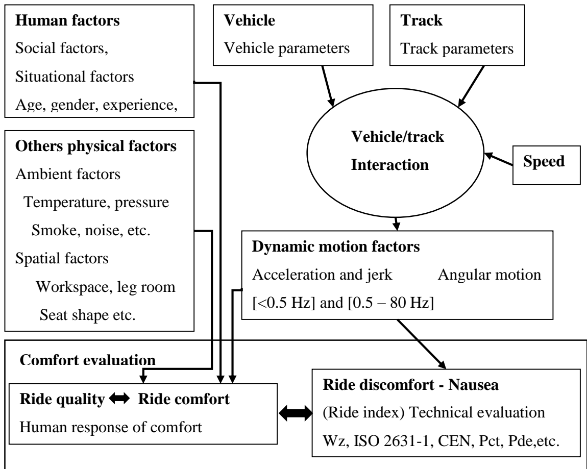
Figure 2.5: Influence from vehicle, track, other physical factors and human factors on ride comfort and ride quality (Iwnicki & Dahlberg, 2006)
