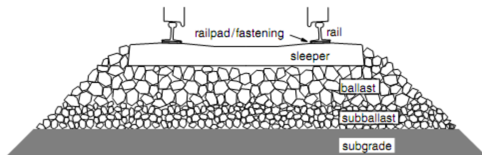
Figure 2.1: Components of track (Iwnicki & Dahlberg, 2006)
