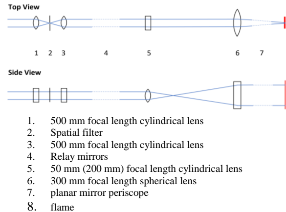
Figure 2. OH (CH 2 O) PLIF optics.
