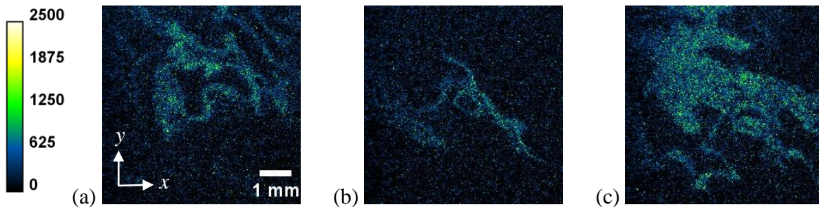
Figure 10. Selected \text{CH}_2\text{O} PLIF images. False color. In the mixing region adjacent to the cavity. Image center coordinates: x/H = (a) 4.61, (b) 4.73, (c) 4.86, y/H = 1.71 .
