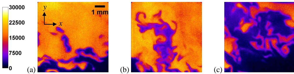
Figure 6. Selected OH PLIF images. False color. Downstream of the cavity. Image center coordinates: x/H = (a) 5.60, (b) 5.65, (c) 6.25, y/H = 1.60 .
