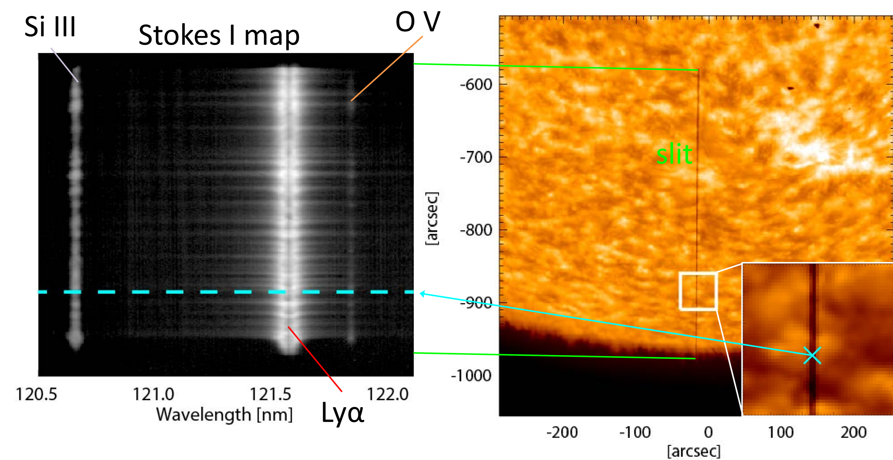
Fig.1 Stokes I map with CLASP (left) and CLASP/SJ Ly \alpha image (right)
