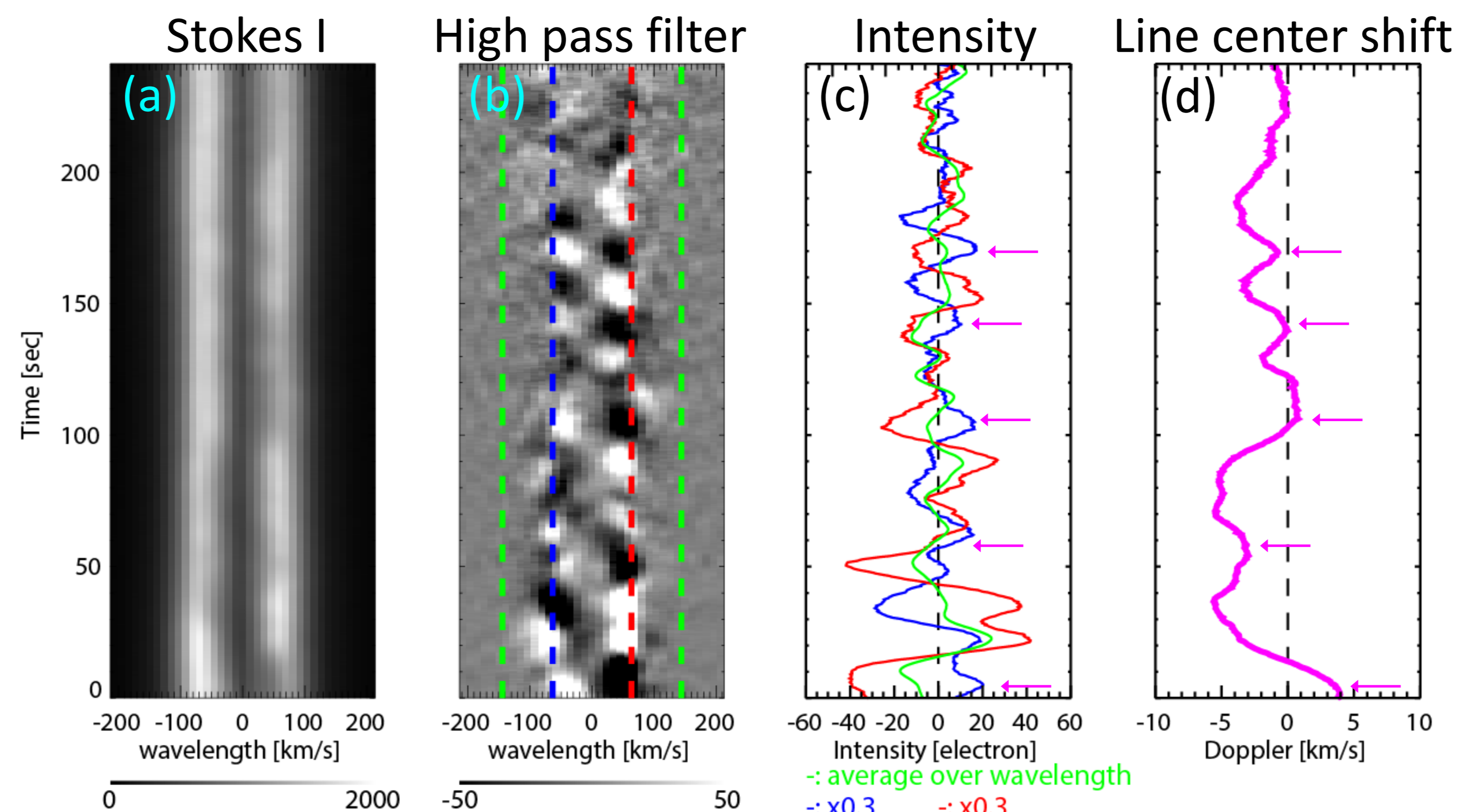
Fig.2 Temporal evolution of Stokes I profiles at "X" of Fig.1 for (a) Ly \alpha & (b) high-pass-filtered Ly \alpha . Time profile of (c) the high pass filtered intensity and (d) Doppler velocity.
