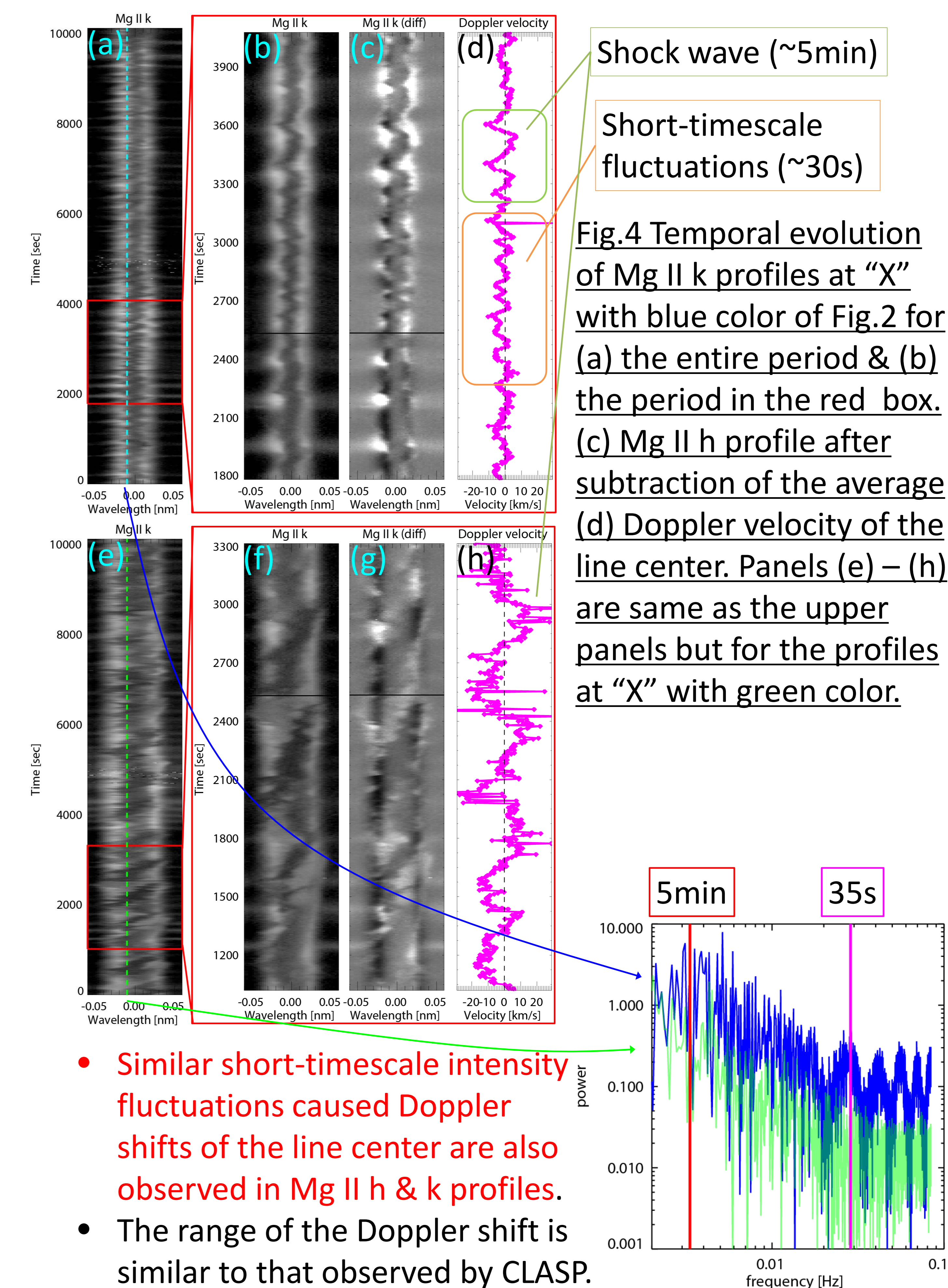
Fig.5. Power spectrum of intensity along the dashed lines in Fig.4
