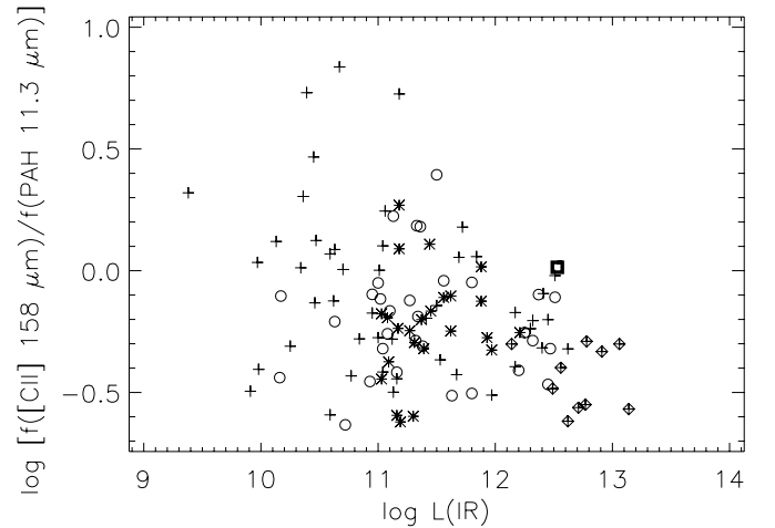
Figure 6. Ratio of [C II] and PAH 11.3 \mu\text{m} line fluxes, compared to total infrared luminosity L_{\text{IR}} in L_{\odot} . Crosses are AGNs from the EW classification, open circles are composite AGNs plus starbursts, and asterisks are starbursts. Sources with diamonds (all AGNs) are upper limits to [C II] line fluxes in Table 1. Square is Markarian 231.
