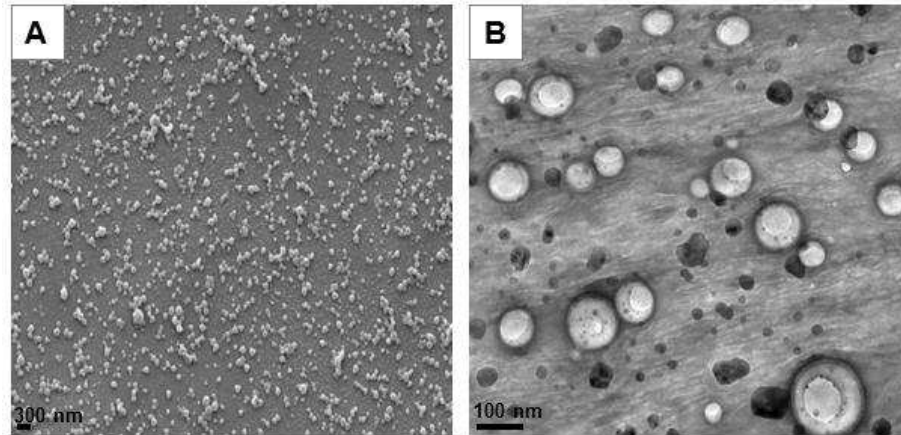
Figure 7. (A) Scanning electron microscope (SEM) and (B) transmission electron microscope (TEM) images showing the morphology of DiD labeled chitosan-PLGA nanoparticles.
